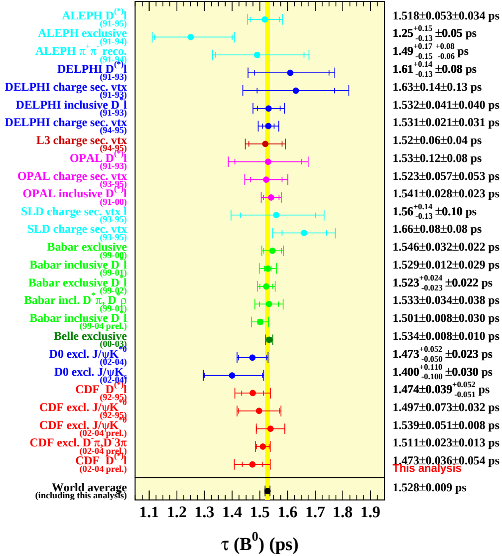
Figure 6.2: A comparison of \tau(B^0) measured by other experiments and this analysis. The result of this analysis is included in the world average.
