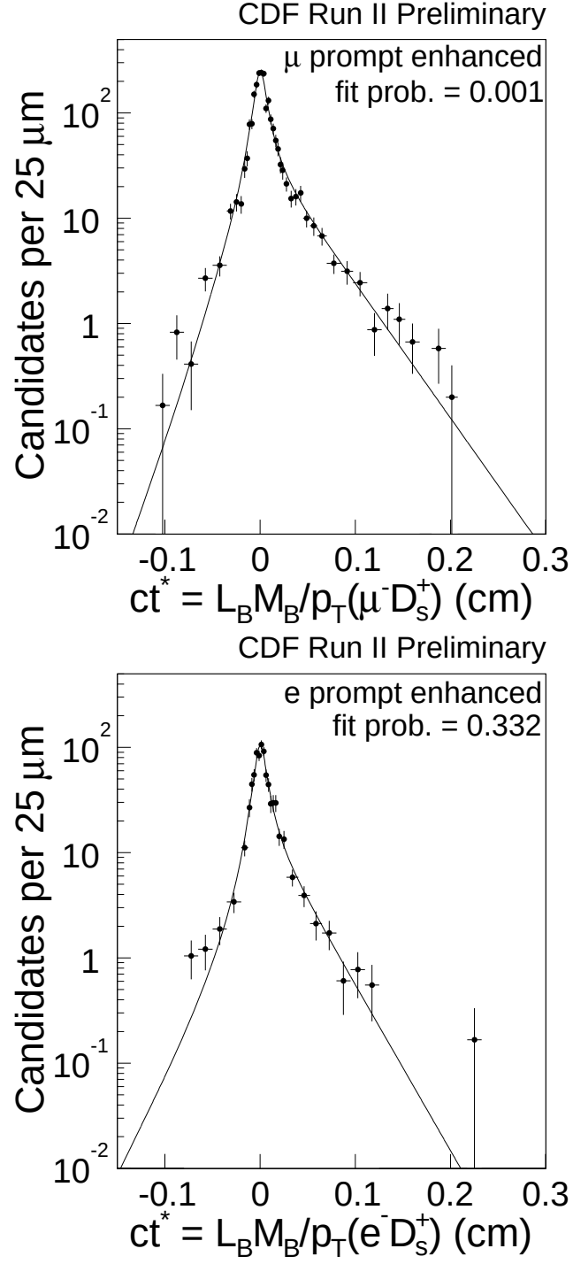
Figure 5.3: Fit results for the prompt enhanced samples when we determine the resolution scale factor.
