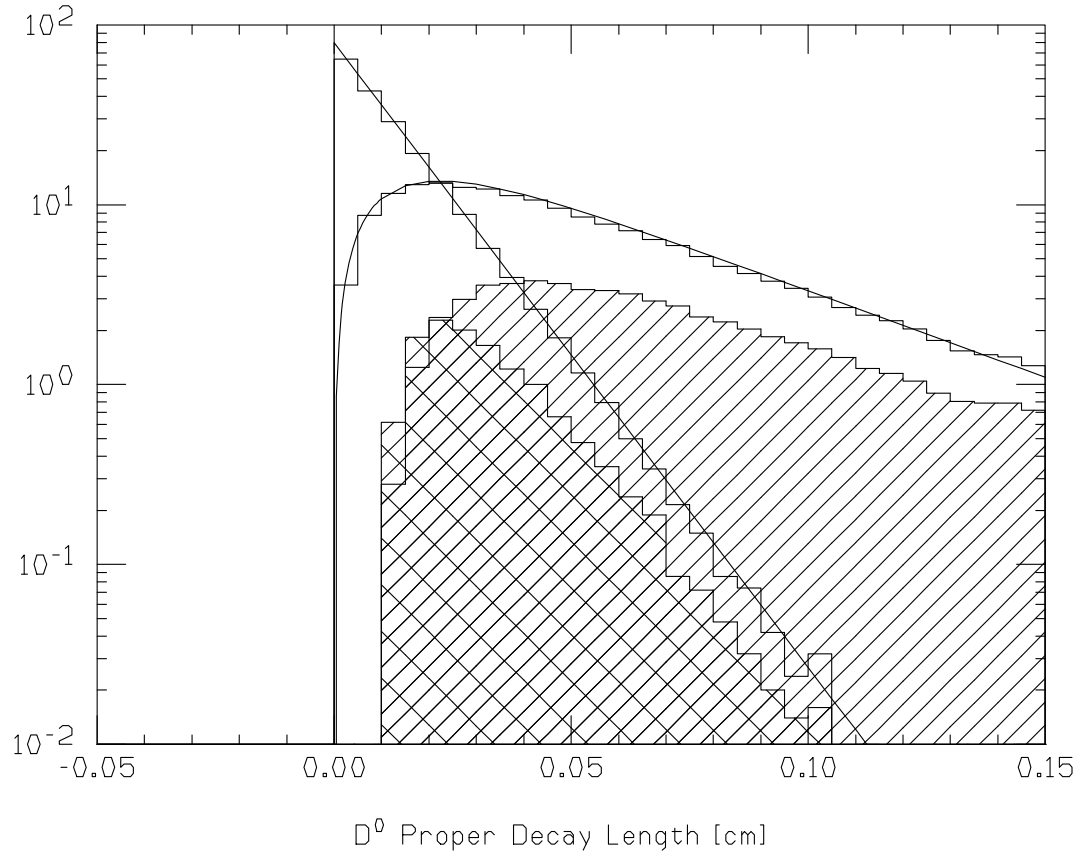
Figure C.1: Distributions of variable ct_2 for prompt and secondary charm mesons (curves). Results of toy Monte Carlo experiments are overlaid as histograms.
