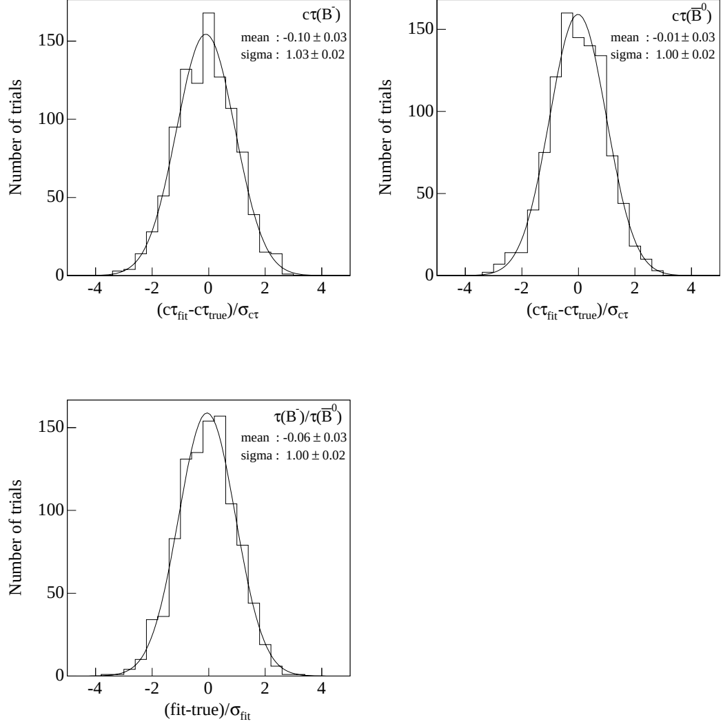
Figure B.1: Pull distributions to check lifetime fitter using toy Monte Carlo samples.
