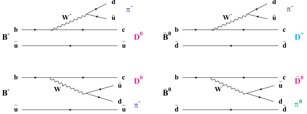
Figure 1.4: External (top) and internal (bottom) spectator diagrams for B^- (left) and \bar{B}^0 (right). In the diagrams of B^- decay the final state contains the same particles, that occurs the Pauli Interference.
