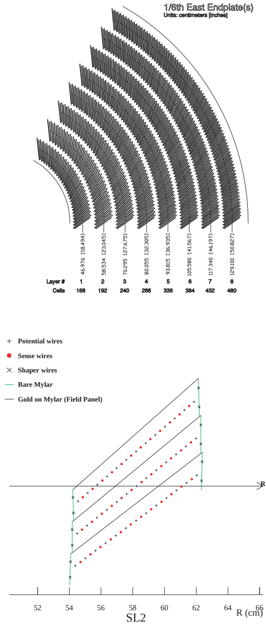
Figure 2.10: r - \phi view of the COT. Upper figure is a view of east endplate. Lower figure shows three drift cells of the COT in superlayer 2.
