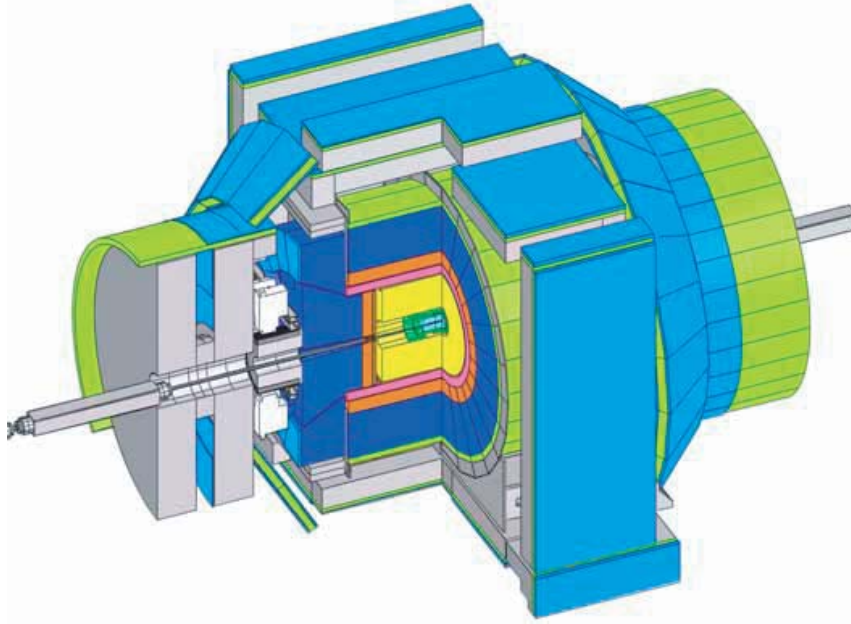
Figure 2.4: Solid cutaway view of the CDF detector.
