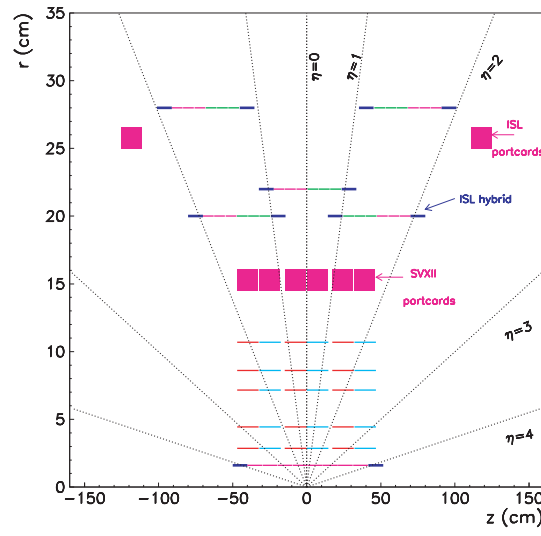
Figure 2.8: Schematic layout of the silicon tracking system.
