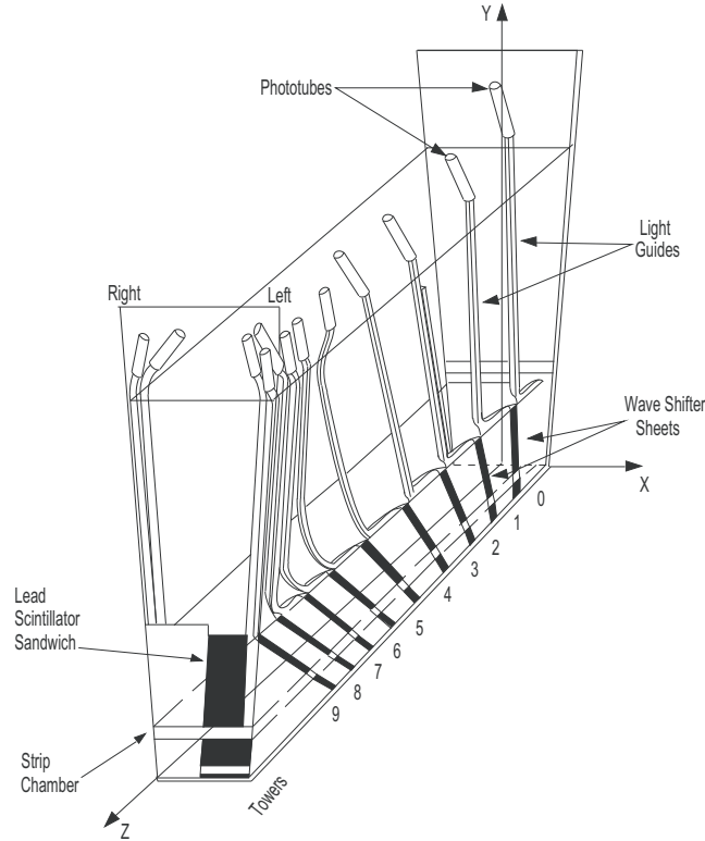
Figure 2.12: One wedge of the CEM with its light collecting system.
