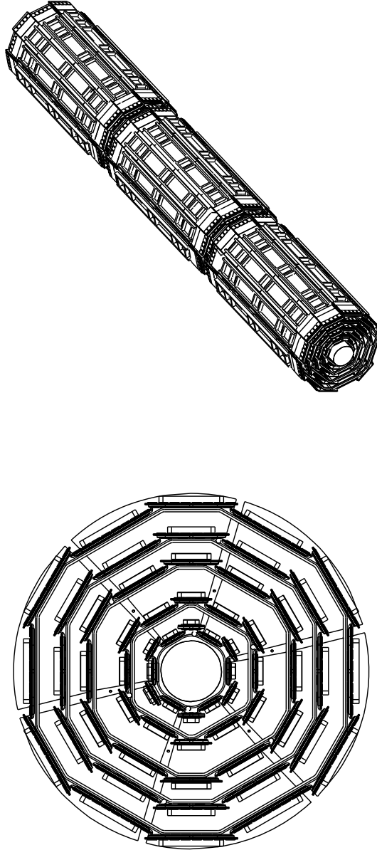
Figure 2.7: Figures of the SVX II detector. Upper figure shows a view of three barrels, and lower figure is r - \phi view for one barrel. Each barrel has 5 layers, and each layer has 12 wedges.
