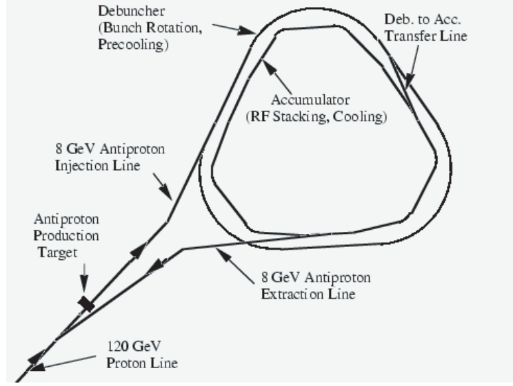
Figure 2.3: Layout of the anti-proton source.
