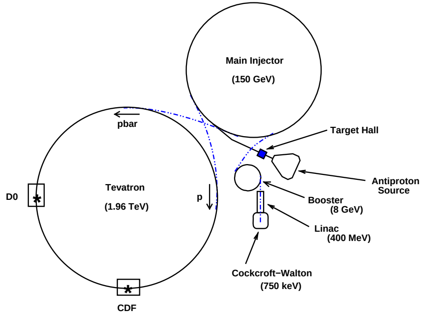
Figure 2.2: Schematic view of the accelerator complex at the Fermilab.
