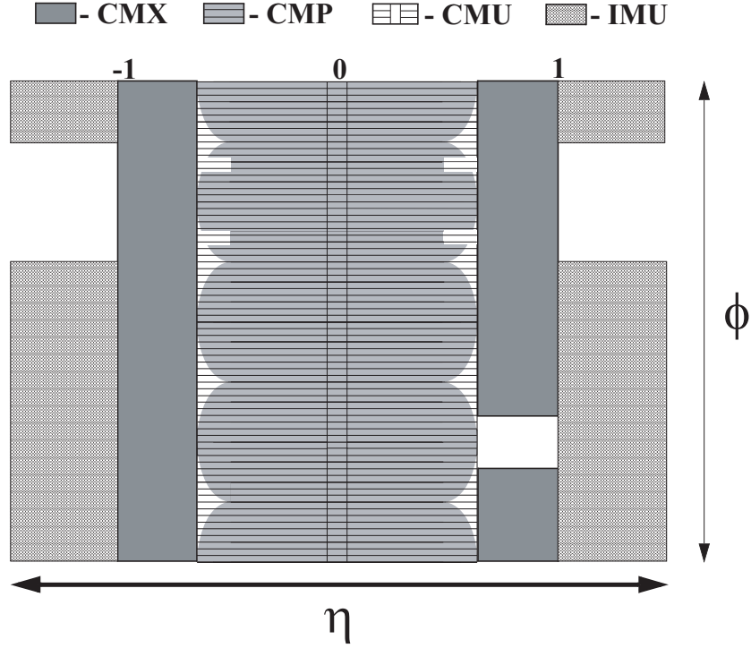
Figure 2.13: Location of the muon detectors for Run II in azimuth \phi and pseudo-rapidity \eta .
