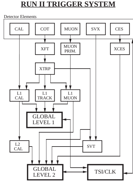
Figure 2.16: Architecture of the three-level pipelined and buffered trigger system used in the CDF experiment. (The numbers are for 132 ns operation, while actual operation is with 396 ns bunch spacing.)
