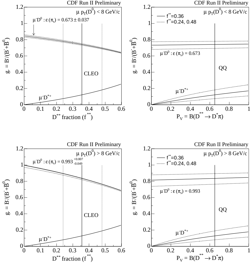
Figure 4.23: The changes of g_- as functions of f^{**} and P_V under several conditions for muon dataset. In the left plots P_V is set to the default value 0.651. Upper plots are for the p_T(D^0) < 8 \text{ GeV}/c region, and lower plots are for the p_T(D^0) > 8 \text{ GeV}/c region. The lifetime ratio \tau(B^-)/\tau(\bar{B}^0) is set to be unity.
