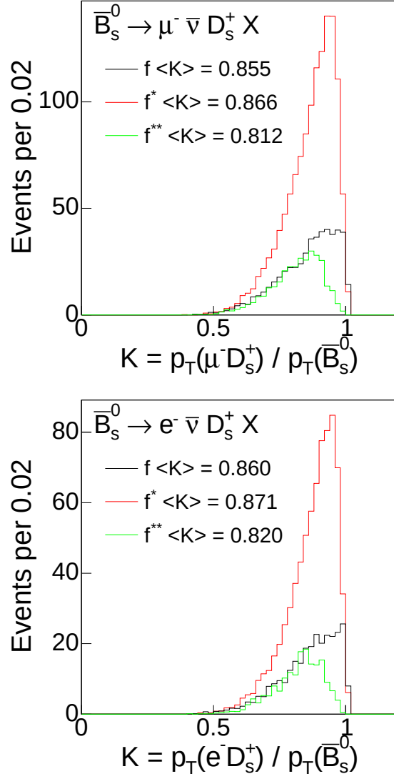
Figure 5.10: Comparison of the distributions of the momentum ratio K for different semileptonic decay modes, \bar{B}_s^0 \rightarrow \ell^- \bar{\nu} D_s^+ , \rightarrow \ell^- \bar{\nu} D_s^{*+} and \rightarrow \ell^- \bar{\nu} D_s^{**+} .
