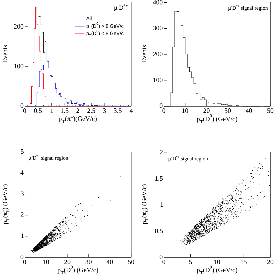
Figure 4.20: The p_T distributions of the slow pion and the D^0 meson, and their correlation. The plots are for \mu^- D^{*+} signal region events. Lower two correlation plots are same but with different scale.
