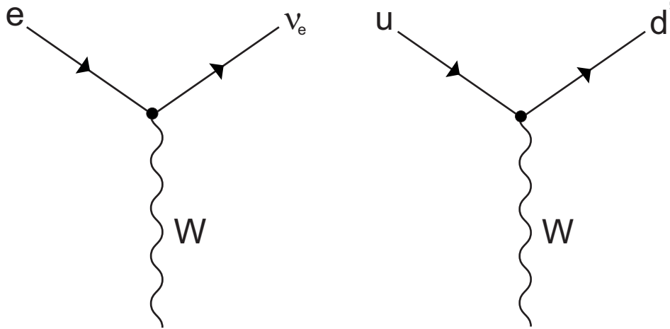
Figure 1.1: Examples of the interaction with W boson for lepton and quark case.
