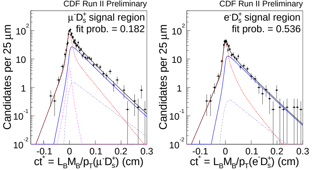
Figure 5.7: The ct^* distributions and lifetime fit results. Left plot is for the muon, and right plot is for the electron dataset. Overlaid curves are the fit functions. Blue curves show the semileptonic \bar{B}_s^0 signal components, red curves are the combinatorial background function. Dashed green and blue curves show the charm and bottom background components, respectively.
