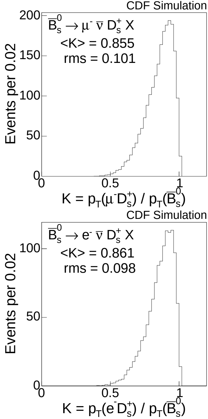
Figure 5.1: The K factor distributions for the muon dataset (top) and the electron dataset (bottom).
