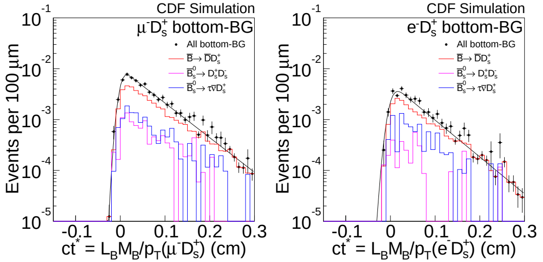
Figure 5.6: The ct^* distributions for bottom background events obtained from the Monte Carlo simulation for muon and electron datasets. Colored histograms show contributions from each processes, and points show sum of all the contributions. Overlaid curves are fit results for the total background shapes and represent the bottom background template functions.
