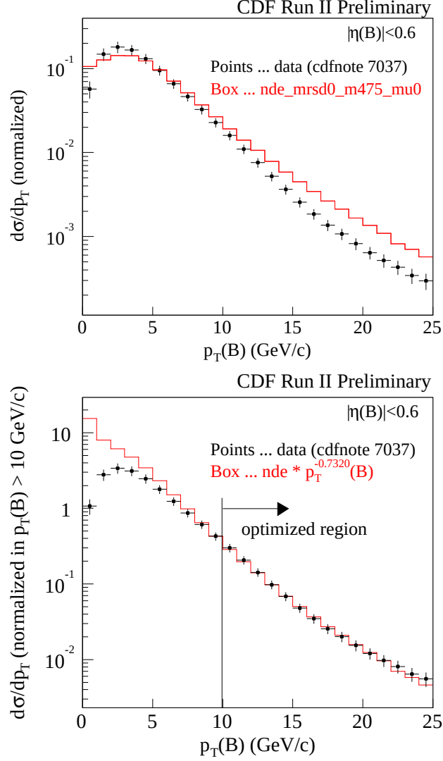
Figure 4.1: Comparison of the B^-/\bar{B}^0 meson transverse momentum spectra between the NDE calculation and the Run II measurement using B \rightarrow J/\psi X . Points show the measured spectrum, and red histogram is the NDE spectrum. Upper plot is a comparison before tuning the NDE spectrum, while lower plot is after tuning.
