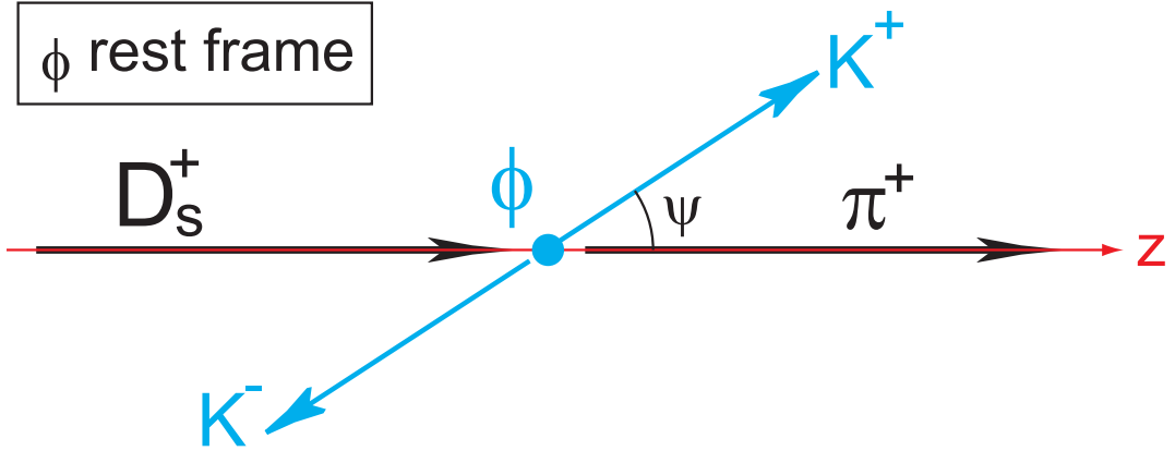
Figure 3.5: A schematic drawing which shows the definition of helicity angle \psi .
