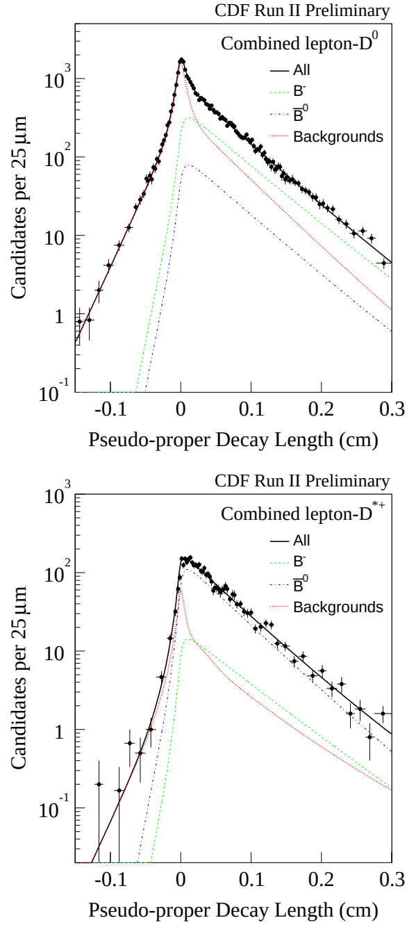
Figure 4.22: The muon and electron combined fit result.
