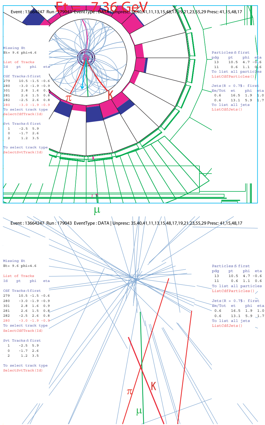
Figure 3.2: An event display of a typical \ell^- D^0 candidate. Lower figure is a close view of the upper figure around the collision point.
