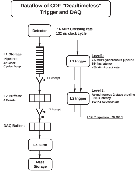
Figure 2.16: Architecture of the three-level pipelined and buffered trigger system used in the CDF experiment. (The numbers are for 132 ns operation, while actual operation is with 396 ns bunch spacing.)
