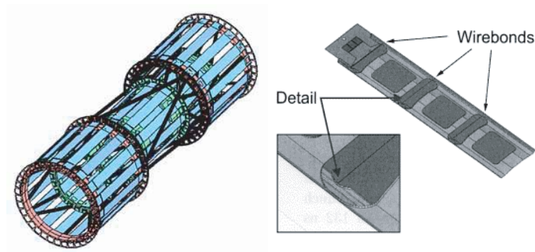
Figure 2.9: Figure of the ISL detector.
