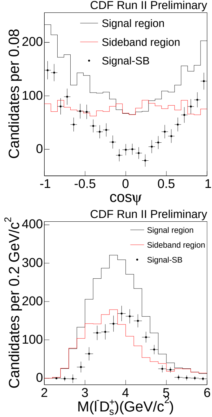
Figure 3.6: The \cos\psi and M(\ell D_s^+) distributions for the \ell^- D_s^+ (muon and electron combined) sample. Distributions for signal, sideband region events are shown as well as the difference between them.
