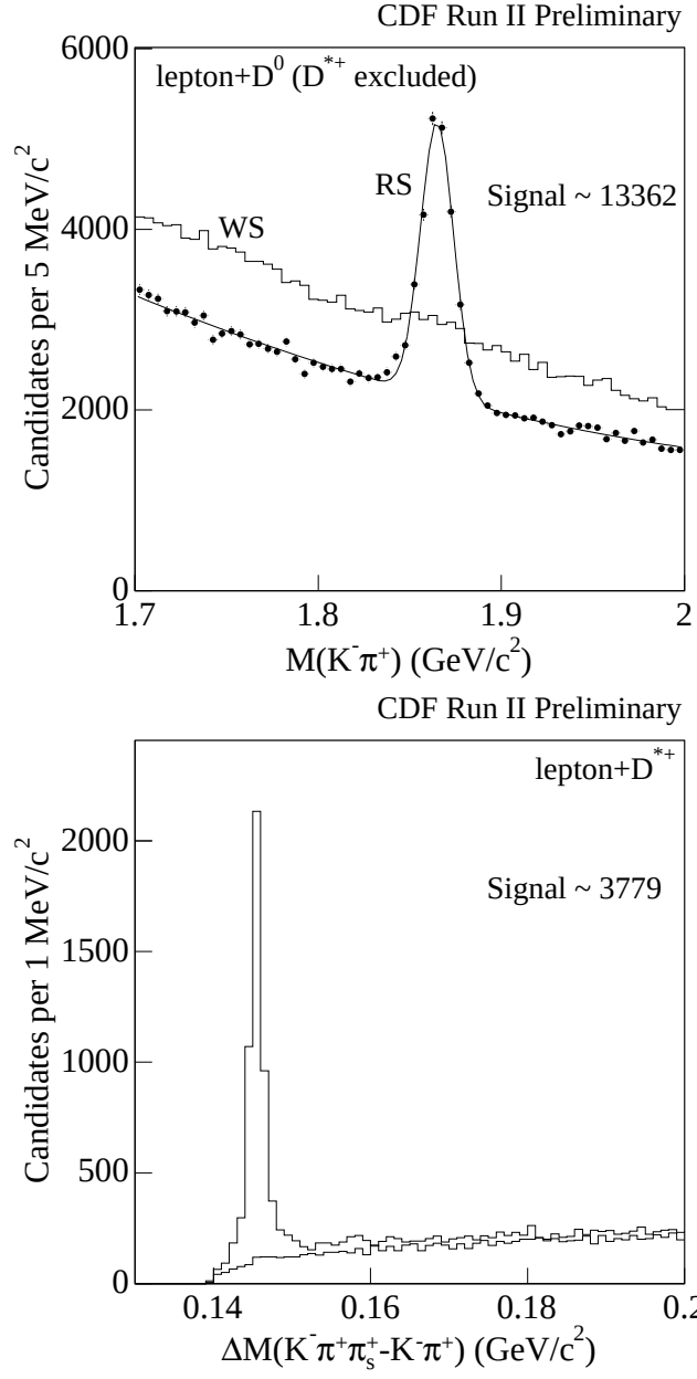
Figure 3.4: M(K^-\pi^+) and \Delta M(K^-\pi^+\pi_s^+ - K^-\pi^+) plots for the \ell^-D^0 ( D^{*+} excluded) and the \ell^-D^{*+} samples (muon and electron combined dataset).
