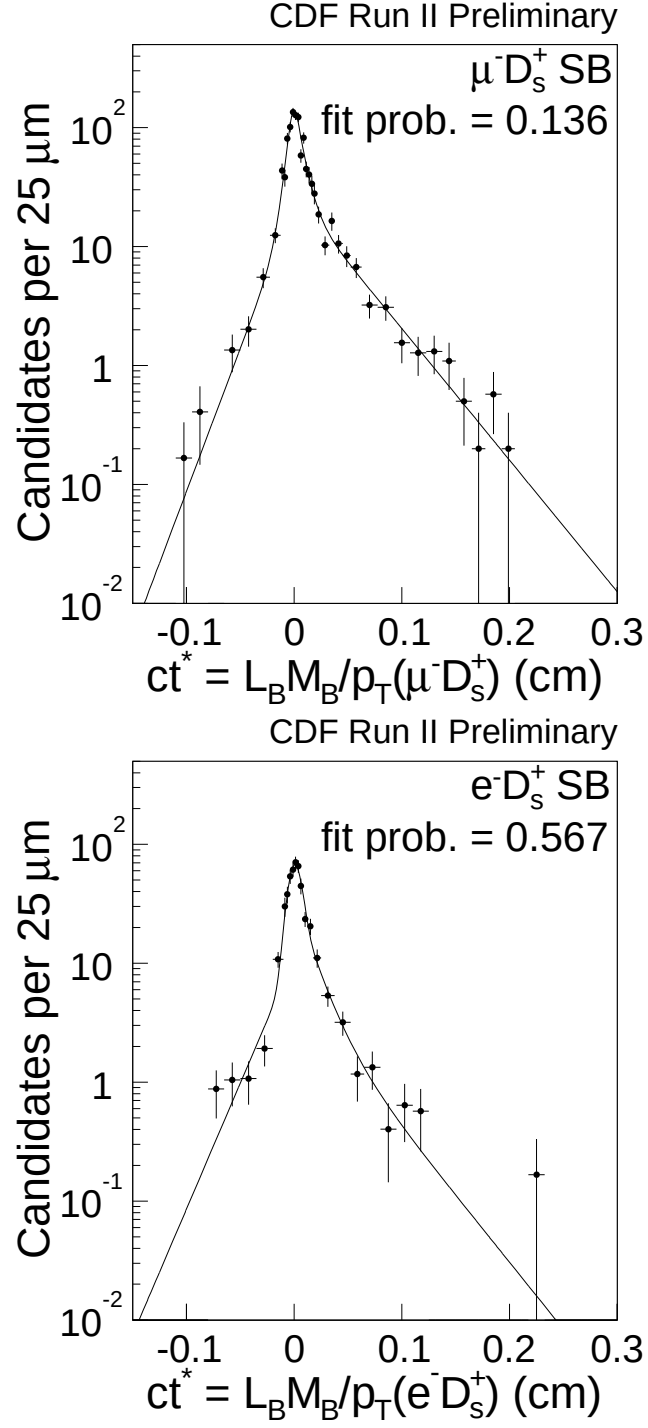
Figure 5.2: Fit results for the ct^* distributions of the sideband events. Overlaid curves show \mathcal{F}_{BG} , which represent the combinatorial background shape to be used in the final lifetime fit.
