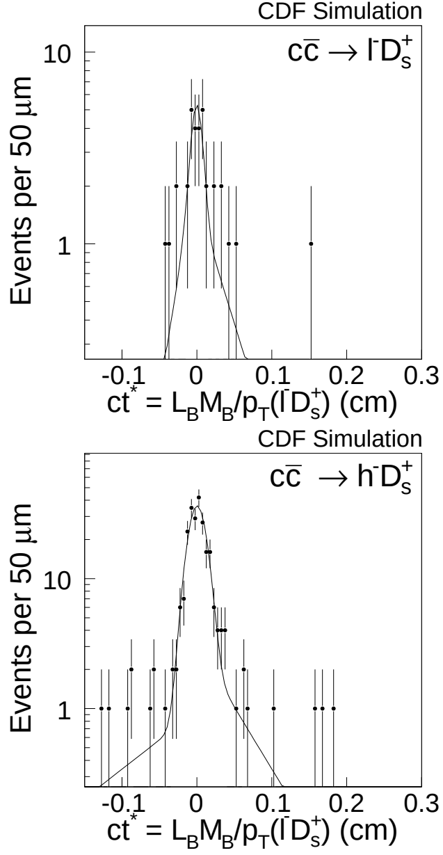
Figure 5.5: Non-zero ct^* distributions for prompt c\bar{c} events.
