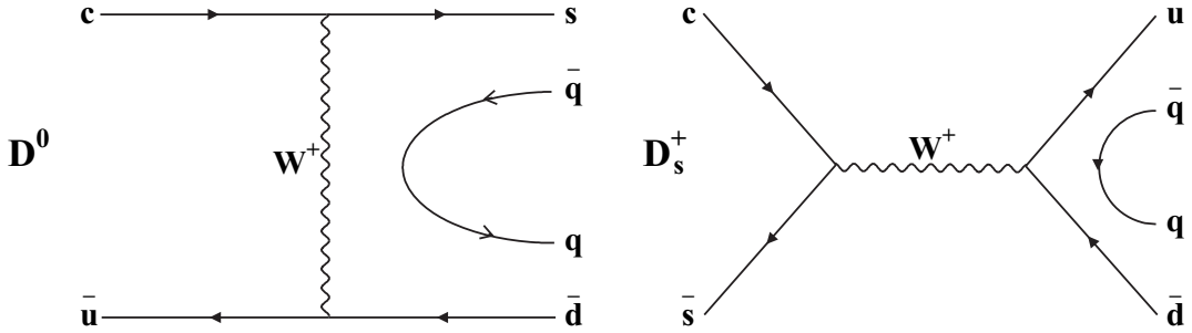
Figure 1.3: Weak annihilation diagrams for charm mesons.
