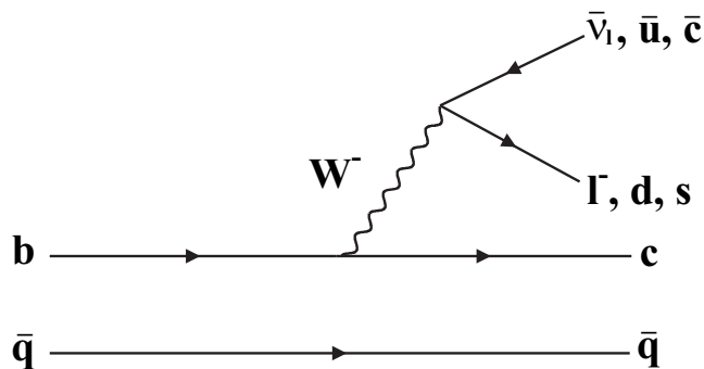
Figure 1.2: The spectator decay diagram of a B meson.
