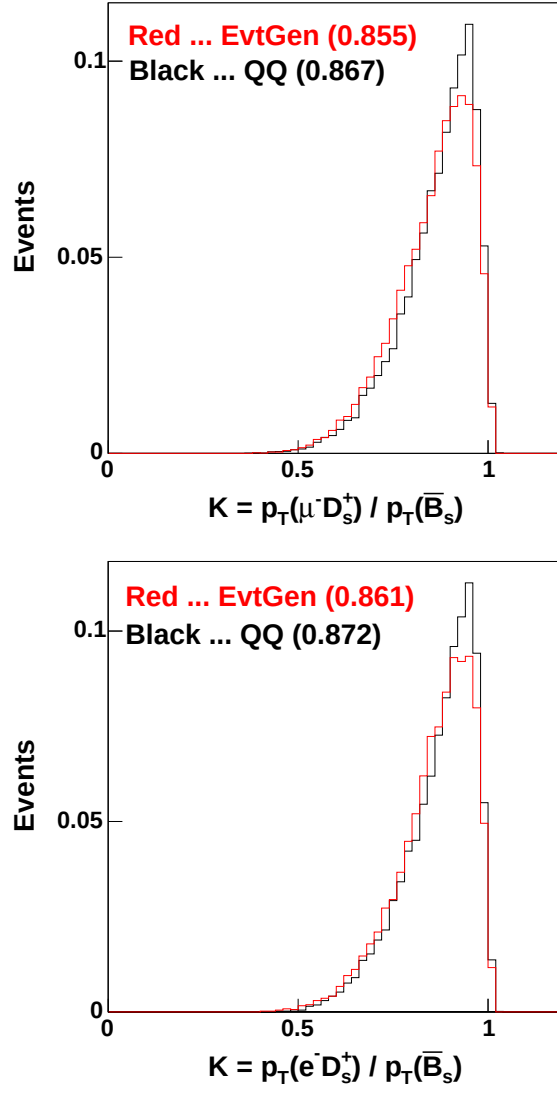
Figure 5.9: Comparison of the K factor distributions with different generators (EvtGen and QQ), for the muon and electron datasets.
