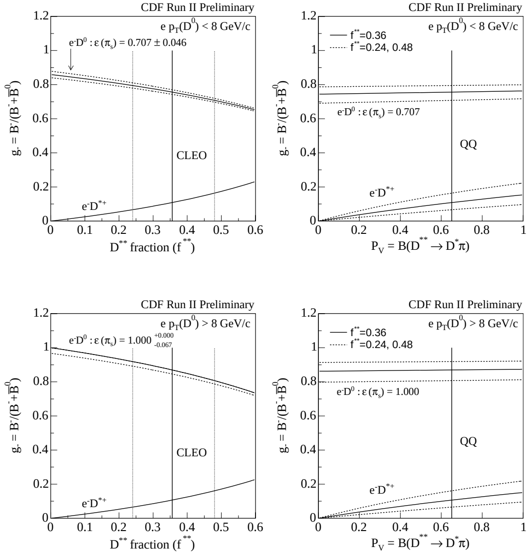
Figure 4.24: Same as the previous figures but for the electron dataset.
