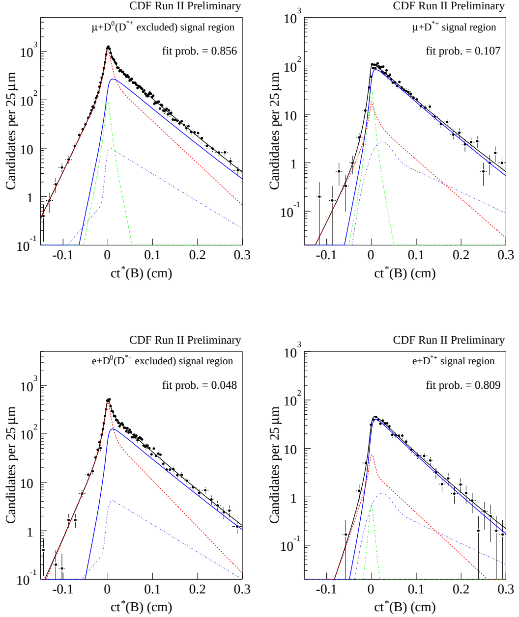
Figure 4.21: The ct^* distributions (points) and the fit results for the muon dataset (upper) and for the electron (lower). Blue curves show the semileptonic B^-/\bar{B}^0 signal components, Red curves are the combinatorial background shape. Dashed green and blue curves show charm and bottom background components, respectively.
