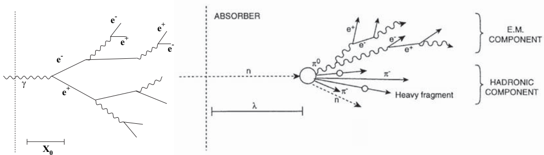
Figure 2.11: Development of an electromagnetic shower (left) and a hadronic shower (right).
