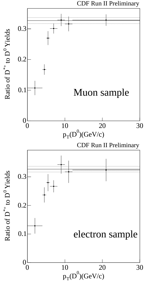
Figure 4.19: The ratio of D^{*+}/D^0 yield against D^0 meson transverse momentum. The lines show a level of plateau, which corresponds to the tracking efficiency of 99.6%.
