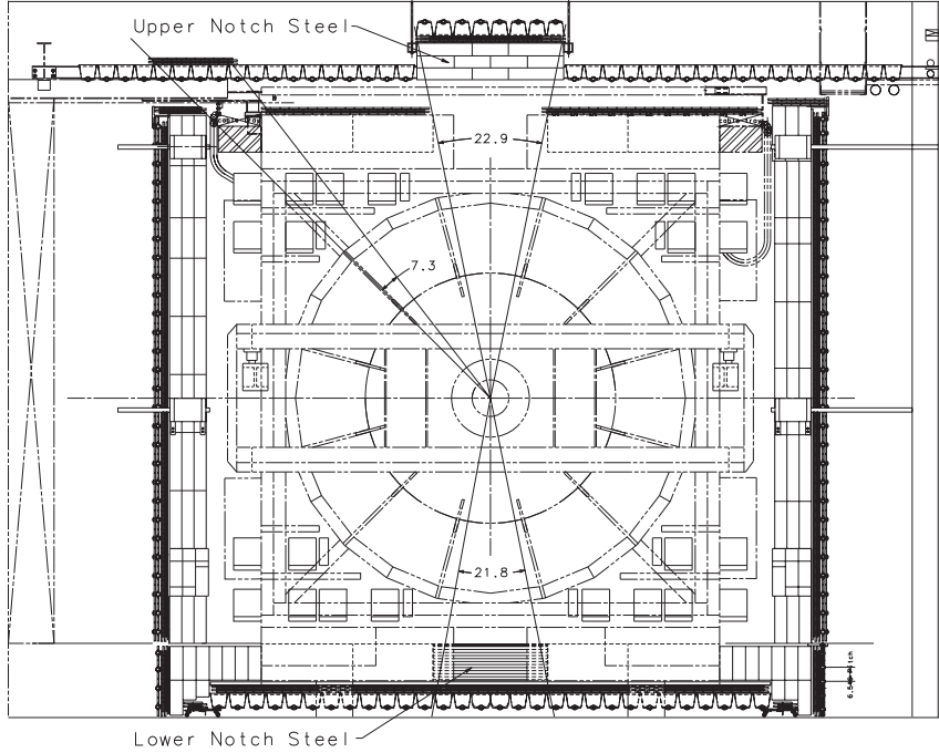
Figure 2.15: Configuration of the CMP. The dark gray square structure surrounding the central detector shows the CMP modules and scintillators.
