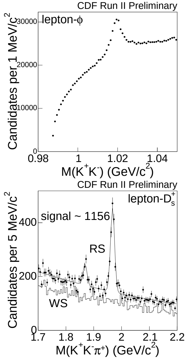
Figure 3.8: M(K^+K^-) and M(K^+K^-\pi^+) plots for muon and electron combined sample.
