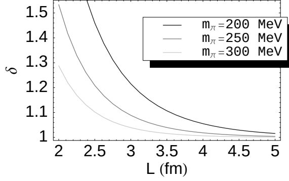
Figure 2.2: The ratio, \delta = d_n^{(L)} / d_n^{(\infty)} , of the neutron edm at finite volume to its value at infinite volume as a function of spatial lattice size L , for c(\mu) = 0 .
