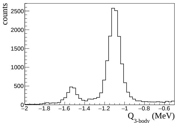
Fig. 2. Experimental Q -value spectrum for the three-body ^2\text{H}(^{10}\text{B}, \alpha^7\text{Be})n reaction.
