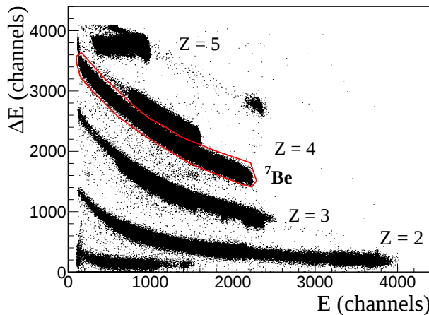
Fig. 1. Typical \Delta E – E matrix. Grey/red contour indicates the selected {}^7\text{Be} events.
