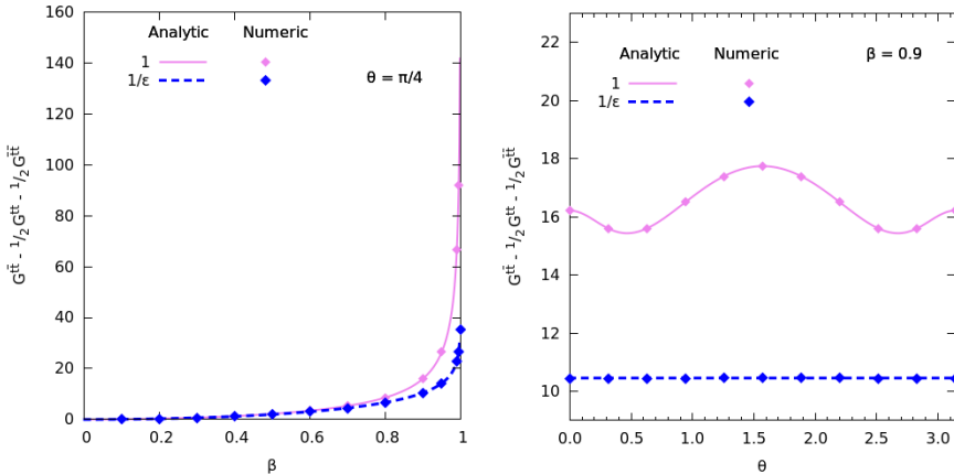
Fig. 2. The numerical and the analytic calculation of the kinematical part of G_{tt}^{\text{fer}} - G_{tt}^{\text{fer}}/2 - G_{tt}^{\text{fer}} . Up to a global power of q_T' , the soft function depends only on the velocity \beta and the polar angle, \theta , of p_t .
