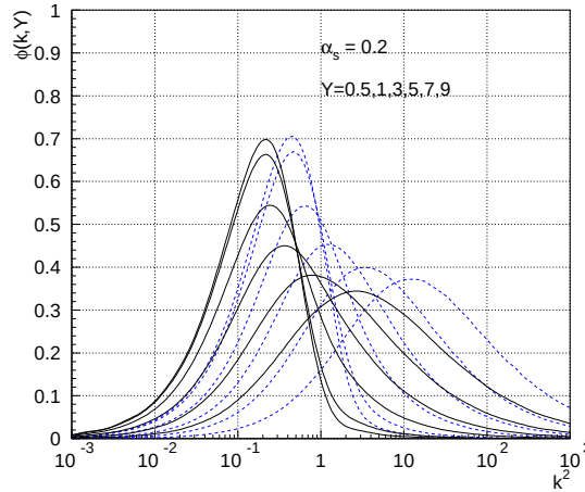
Fig. 1. Solution to the BK equation in the form of the unintegrated distribution \phi(x, k_\perp) for different values of the rapidity.
