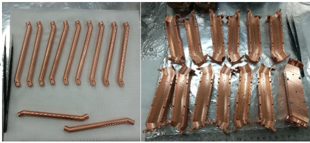
Figure 8: Coaxial bend transition parts.
