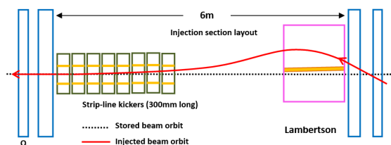
Figure 1: Injection section layout.
