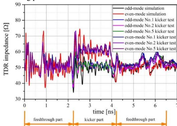
Figure 10: Time-domain reflectometer of prototype kicker.
