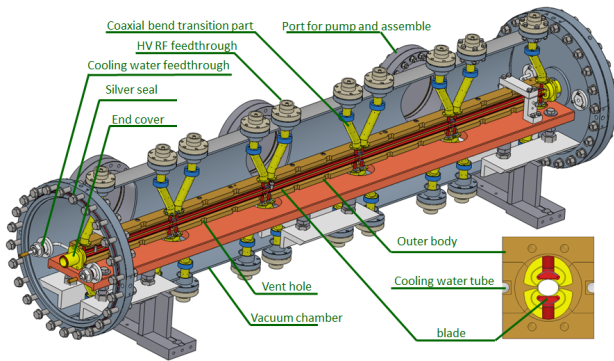
Figure 3: 3D mechanical assembly drawing of kickers.
