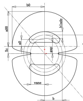
Figure 2: The cross shape of the strip-line kicker.
