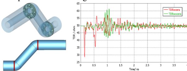
Figure 4: Simulation result of coaxial bend transition part.
