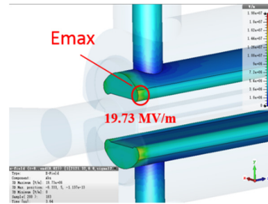
Figure 5: Maximum local electric field intensity distribution.
