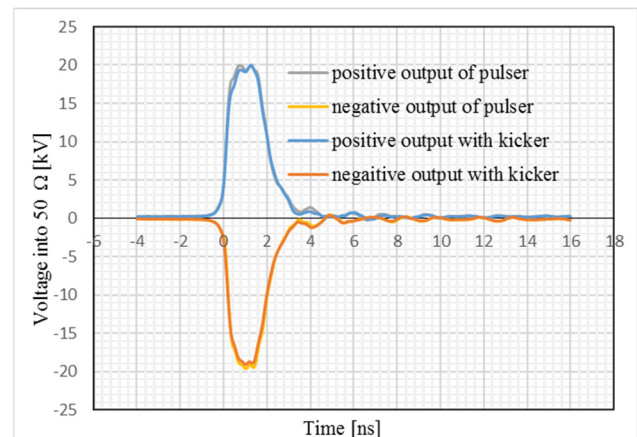
Figure 12: The HV test pulse waveform.
