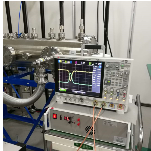
Figure 11: The prototype kicker HV test setup.
