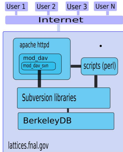
Figure 1: The Lattice Repository Architecture.
