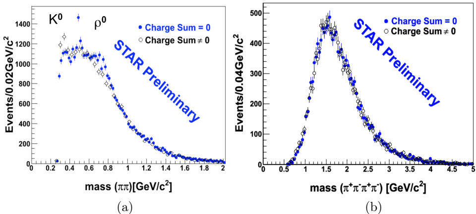
Fig. 4. (a) Reconstructed mass distributions for two; and (b) four charged pions in the inclusive central diffraction at \sqrt{s} = 200 GeV. Reconstructed particles are assumed to be pions. Solid circles are for neutral states and open circles represents charged states. Errors are statistical only.
