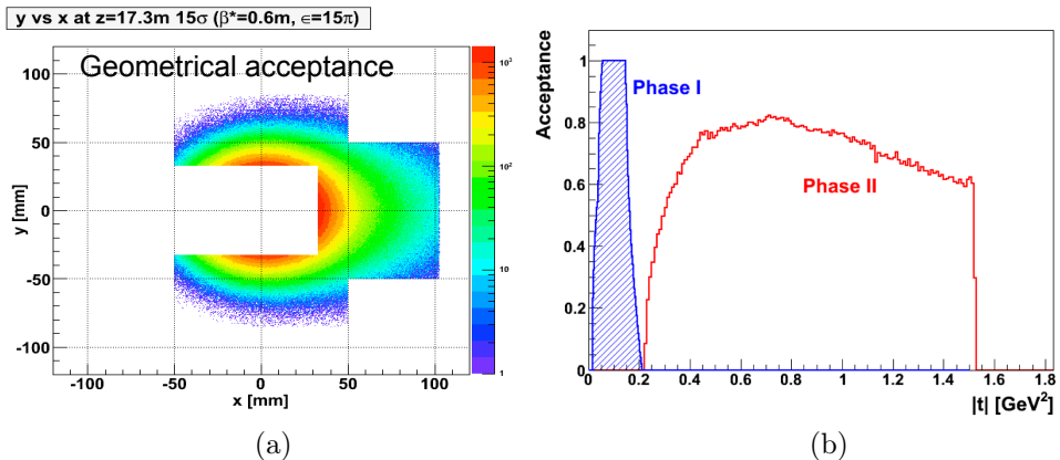
Fig. 5. (a) Geometrical acceptance of Phase II setup for RPs at z = 17.3 m calculated by the beam transport simulator HECTOR [28]; and (b) Acceptance as a function of t for Phase I Roman Pots and Phase II Roman Pots at \sqrt{s} = 500 GeV.
