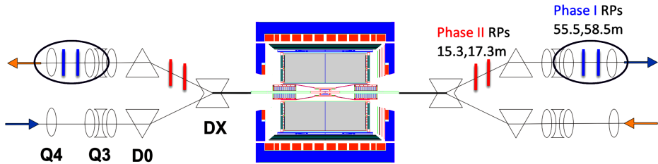
Fig. 2. The layout of the RPs with the STAR detector (not to scale). The Phase I setup, designed to detect scattered protons with low- t , are located after two dipole magnets (DX, D0) and three quadrupoles at 55.5 m and 58.5 m from the interaction point (IP), respectively. For measuring protons with high- t (Phase II), sets of RPs will be positioned between DX and D0 magnets, at 15.3 m and 17.3 m from IP.
