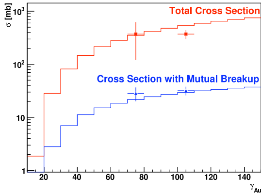
Fig. 7. The \rho^0(770) production cross-section measured by STAR in heavy ion UPC collisions.
