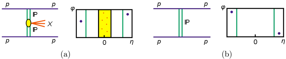
Fig. 1. (a) Central Production diagram in DPE and (b) elastic scattering.
