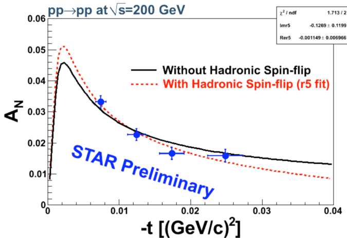
Fig. 3. The single spin asymmetry A_N as a function of -t . The solid curve corresponds to theoretical calculations without hadronic spin-flip and the dashed one represents the r_5 fit. Vertical bars are for statistical errors. Systematic uncertainties (10%) in t -scale is shown as horizontal error bars.
