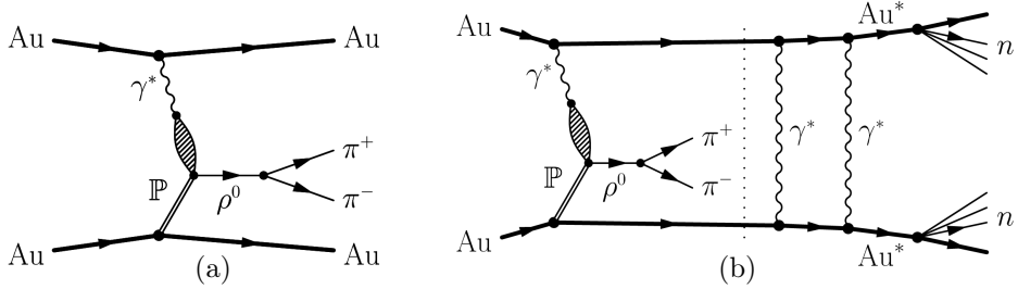
Fig. 6. A diagram of the photonuclear production of a \rho^0(770) meson in a UPC AuAu collision and its decay into two charged pions. (a) shows the exclusive reaction, and (b) one with mutual Coulomb excitation of the beam ions and following neutron emission.
