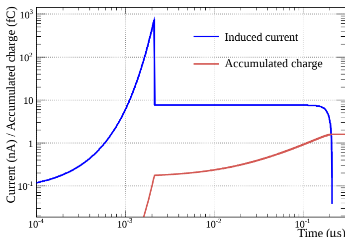
Figure 3.5: Plots of the MICROMEAS induced current and accumulated charge versus time.
