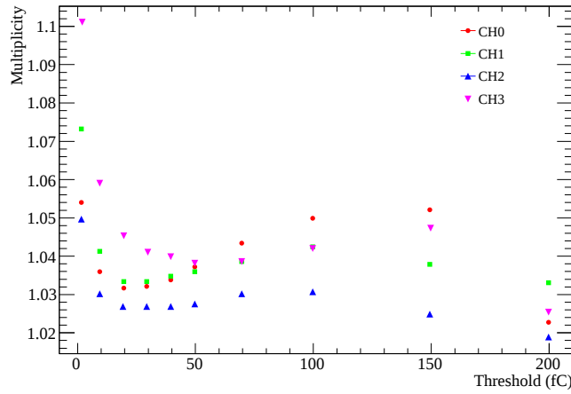
Figure 5.16: Multiplicity versus threshold for the four chambers.
