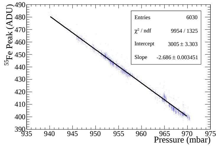
Figure 4.4: ^{55}\text{Fe} peak value versus atmospheric pressure at constant temperature ( T=298 \text{ K} ).
