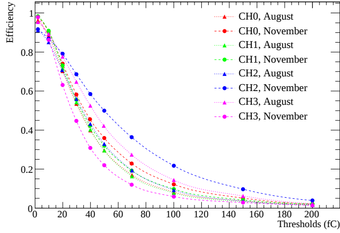
Figure 5.14: Efficiency versus threshold (CH1).
