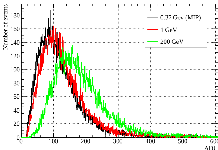
Figure 5.17: GEANT4 simulation of distribution of energy loss for muons crossing 3 mm of Ar/ i\text{C}_4\text{H}_{10} (95/5)
