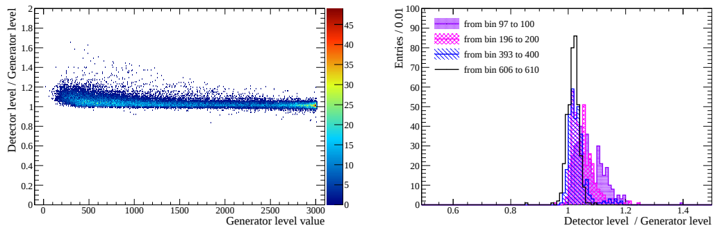
(a) Smearing map for the total event invariant mass. (b) Example of slice histograms from the total event invariant mass smearing map.
