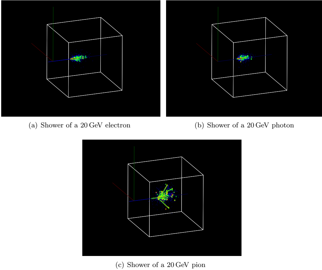
Figure 2.5: Display of particle showers in a 1\text{ m}^3 Fe Calorimeter (40 layers of 2 cm thick Fe absorber, gaseous active medium with 1\text{ cm}^2 lateral segmentation).
