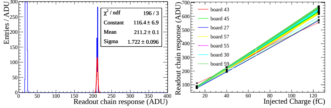
(a) Response of the readout chain to an injected charge of 40 fC. (b) Calibration peak versus injected charge.
