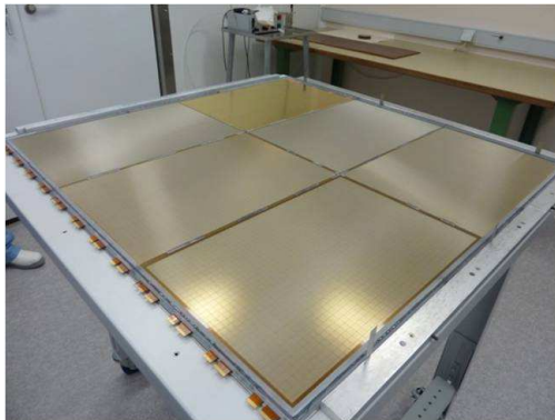
Figure 6.7: Square meter prototype assembled.
