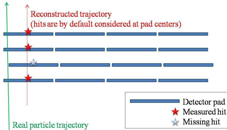
Figure 5.8: Geometrical inefficiency
