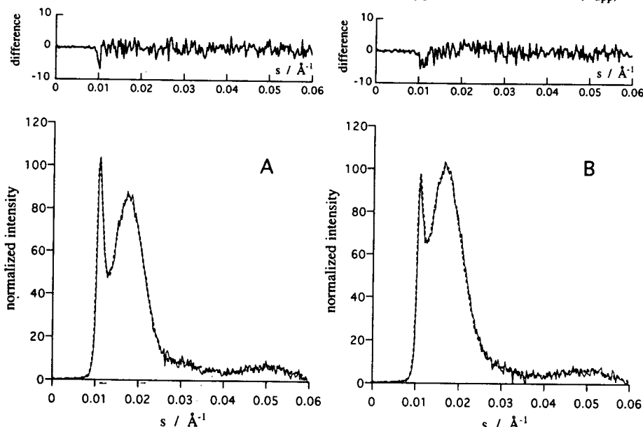
FIGURE 3: Time-resolved patterns along with corresponding linear combination patterns: Solid curve, time-resolved pattern; broken curve, best least-squares fit using a linear combination of T and R patterns. The difference between the two curves is shown in the upper part of the figure. The fraction of the R structure, \bar{R} , was determined to be 0.392 \pm 0.006 for A (at 8–12 s) and 0.799 \pm 0.004 for B (at 44–48 s) by a nonlinear least-squares fit in the s range 0.012 – 0.04 \text{ \AA}^{-1} .
