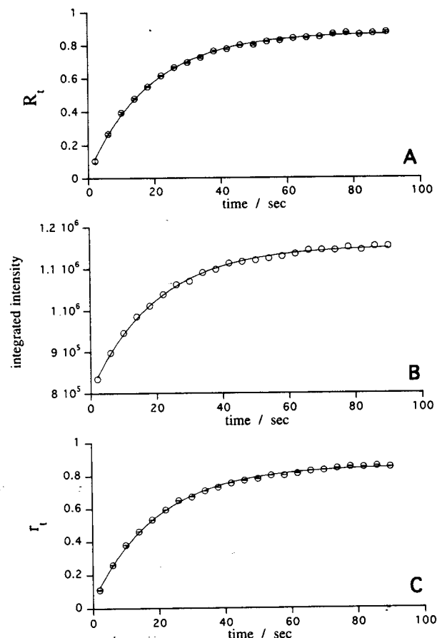
FIGURE 4: Evolution of the structural change shown for the different quantities: A, \bar{R} ; B, integrated intensity over the s range 0.012–0.026 Å -1 ; C, \bar{r} . Evaluated apparent rate constants are (5.25 \pm 0.10) \times 10^{-2} \text{ s}^{-1} (A), (4.99 \pm 0.11) \times 10^{-2} \text{ s}^{-1} (B), and (5.05 \pm 0.11) \times 10^{-2} \text{ s}^{-1} (C), respectively.
