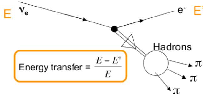
Figure 7.2: A typical \text{CC}\nu_e interaction which produces an e-like multi-ring event in SK.
