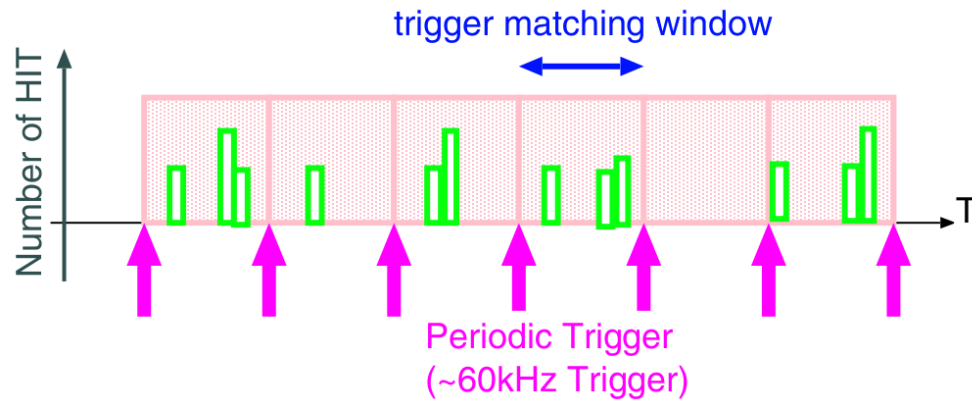
Figure 2.8: A schematic of the new periodic software trigger. Taken from Ref. [33]
