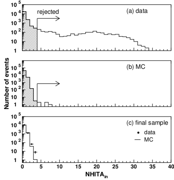
Figure 5.7: The removal of stopping muons in FC5. \text{NHITA}_{in} is shown for (a) data, (b) MC and (c) final FC sample with normalized MC. Taken from [88].
