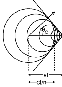
Figure 2.3: A schematic of the Cerenkov radiation emission angle relative to the charged particle's track. Taken from Ref. [112]
