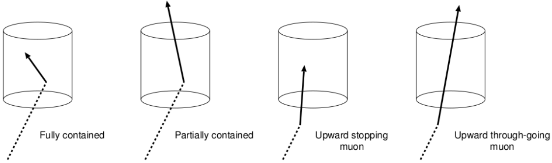
Figure 5.1: Typical neutrino (dashed) and resulting charged lepton (solid) tracks for the fully contained (FC), partially contained (PC), upward-going stopping (Up-Stop) and upward through-going (Up-thru) event types, shown left to right.
