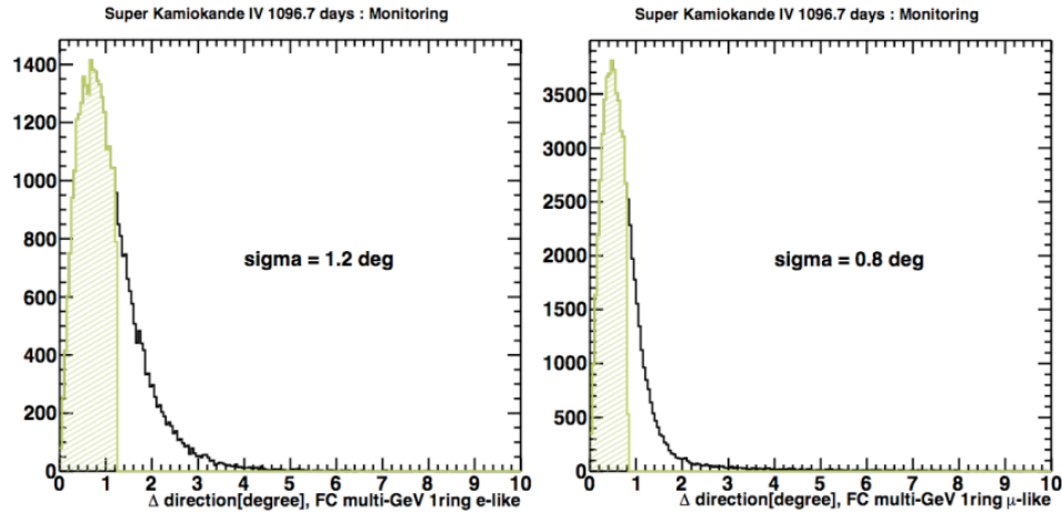
Figure 6.10: Angle between true and reconstructed direction for SK-IV FC MC e-like (left) and \mu -like (right) samples. Sigma (shaded region) represents 68% of the full area.
