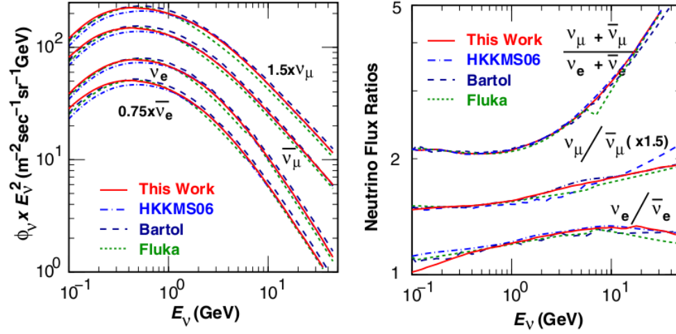
Figure 4.2: The energy dependence of flux for each neutrino type (left) and important flux ratios (right). HHKMS06 is the Honda 2006 flux[48], and Bartol[3] and Fluka[4] are existing alternative flux calculations. Taken from [49].
