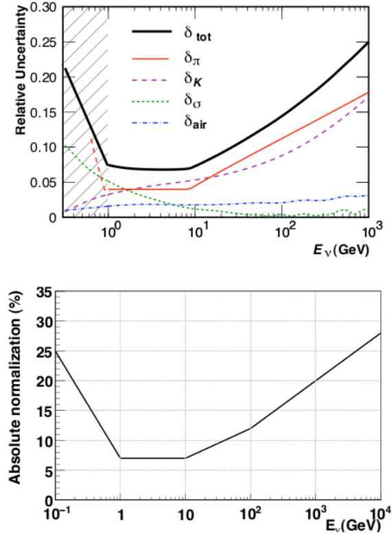
Figure 7.4: The components entering the absolute normalization uncertainty (top) and the overall uncertainty (bottom) as functions of energy[48].
