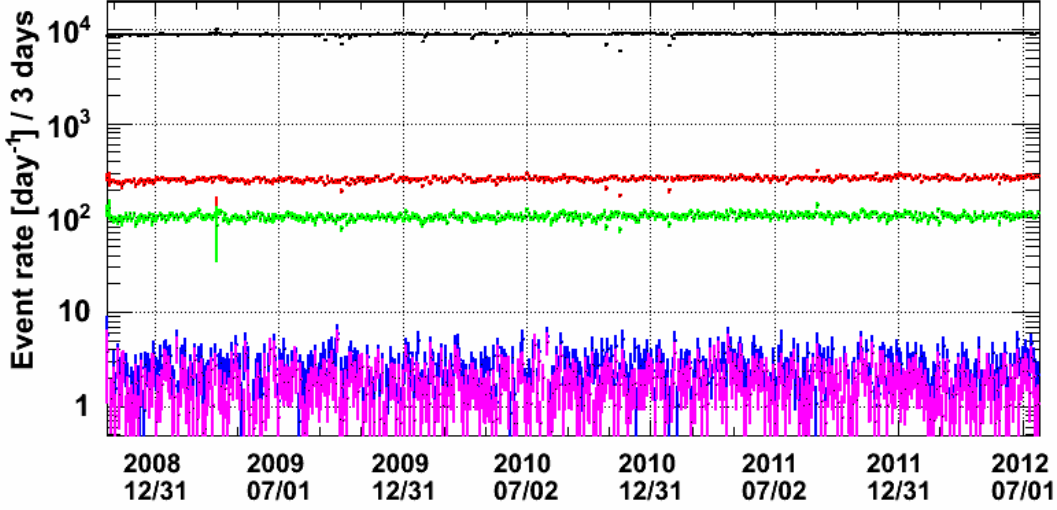
Figure 5.19: The event rate output of umred1st (black), umred2nd (red), precisefit (green), umred3rd (blue) and umred4th (magenta) for SK-IV from the automated upmu reduction software.
