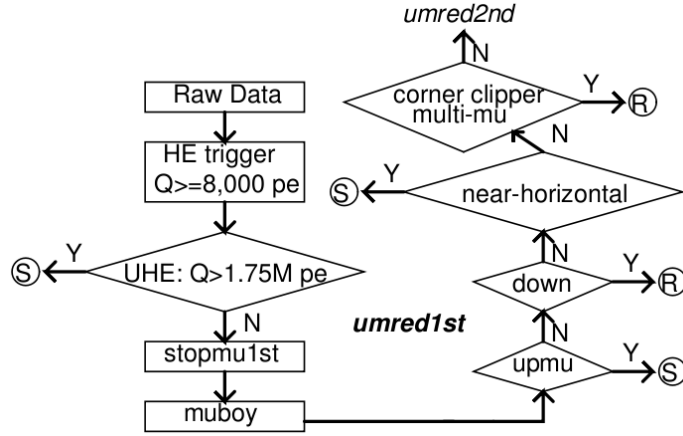
Figure 5.13: A flow chart describing the umred1st selection and rejection steps. Taken from [111].
