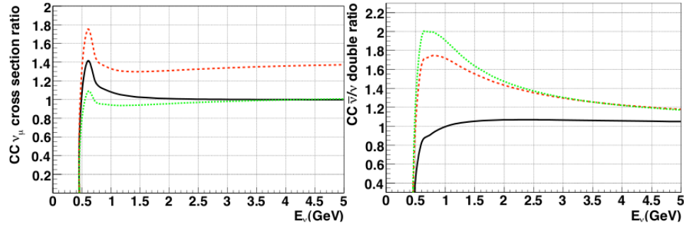
Figure 7.6: Predicted cross-sections (left) and \bar{\nu}/\nu cross-section ratio for \nu_\mu p \rightarrow \mu^- p \pi^+ (solid), \nu_\mu n \rightarrow \mu^- p \pi^0 (dashed) and \nu_\mu n \rightarrow \mu^- p \pi^+ (dotted) for the Hernandez model[85] normalized to the Rein-Sehgal model[101].
