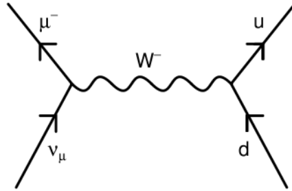
Figure 5.11: Charged-current weak interaction which produces can produce an upmu. Taken from [111].
