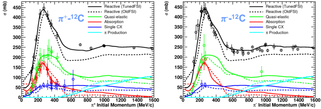
Figure 4.6: The cross-sections from old and new pion interaction models in NEUT compared to data as a function of pion momentum.
