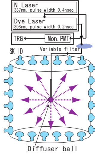
Figure 3.17: The setup used for the timing calibration measurement.
