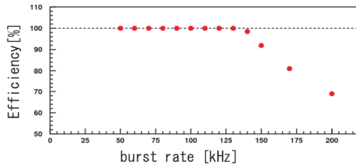
Figure 2.11: The high-speed processing rate of the QBEEs. Frequency of the input signal is on the horizontal axis. Taken from Ref. [33]
