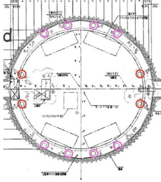
Figure 5.2: Location of the cable holes in the top of the tank. Red circles indicate holes with veto counters and pink circles those without. Taken from [92].
