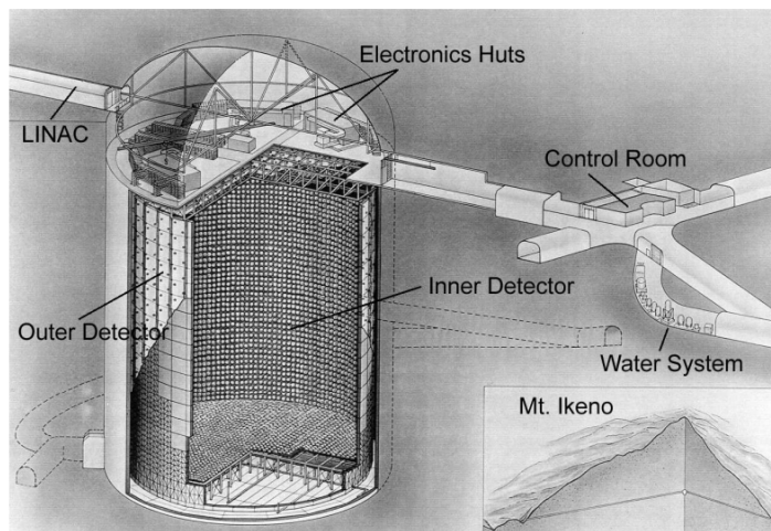
Figure 2.2: An overview of the SK detector and its location within Mt. Ikenoyama. Taken from Ref. [12]
