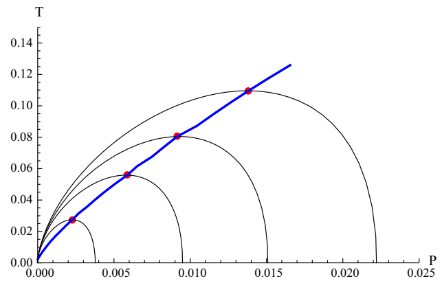
Fig. 5 The isenthalpy process in P - T graph with fixed M = 15, 18, 20, 22 from bottom to top (black lines). We set q = 10 and \alpha = 1 . The red points in each process denote the transition points of the cooling and heating regions for the related M , satisfying \mu_J = 0 . The blue line is P_i - T_i border
