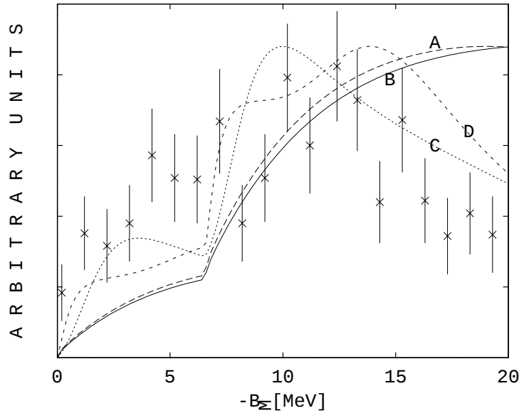
Fig.1. Pion spectrum from (K^-, \pi^+) reaction on ^{16}\text{O} at \theta = 0^\circ at p_K = 450 MeV/c. See text for explanation.
