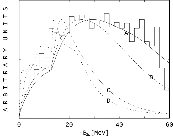
Fig. 2. Pion spectrum from (K^-, \pi^+) reaction on {}^9\text{Be} at \theta = 4^\circ at p_K = 600 MeV/c. See text for explanation.
