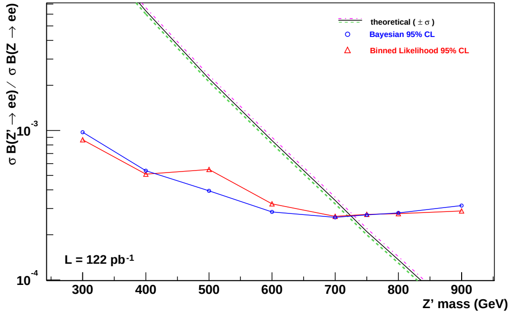
Figure 9.4: 95% CL limit as a function of m_{Z'} for (\sigma B)_{Z'}/(\sigma B)_Z as well as the theoretical value.
