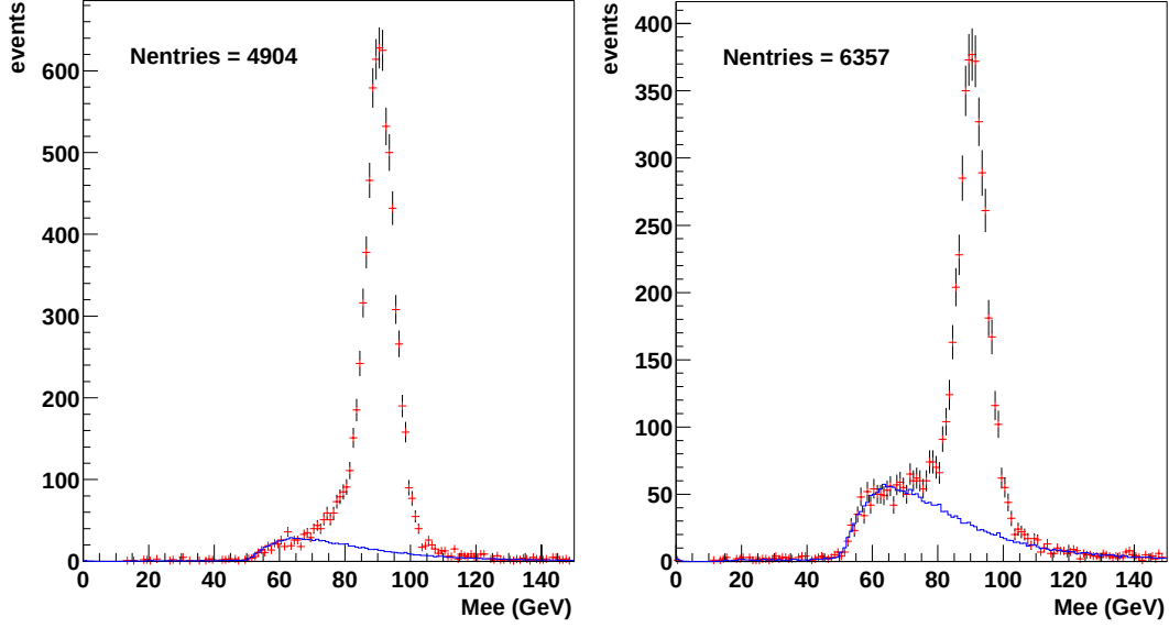
Figure 7.6: The N_1 + 2N_2 (left) and N_0 + N_1 + N_2 (right) distributions for CCCC events. The points are data. The line is the expected non-Z background.
