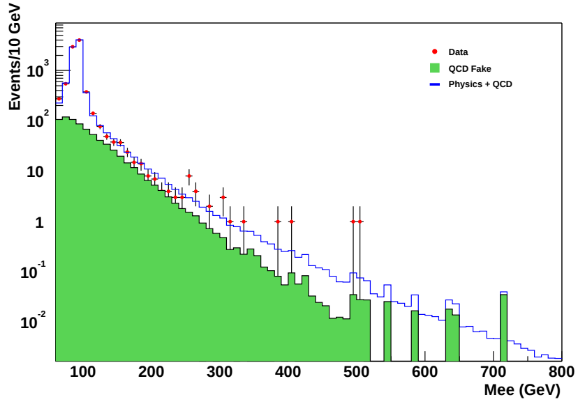
Figure 9.2: The invariant mass distribution of data (points) and expected background (the line is the Physics+QCD background, whereas the shaded region is for the QCD fake background alone).
