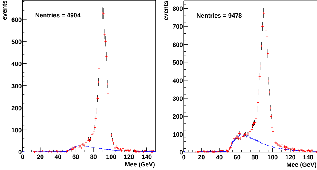
Figure 7.4: The 2(tt)+(tp) (left) and 2(tt)+(tp)+(tf) (right) distributions for CCCC events. The points are data. The line is the expected non-Z background.
