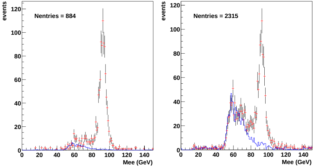
Figure 7.7: The N_1 + 2N_2 (left) and N_0 + N_1 + N_2 (right) distributions for ECEC events. The points are data. The line is the expected non-Z background.
