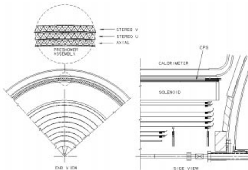
Figure 4.13: Cross-sectional end view (left) and side view (right) of the Central Preshower detector.
