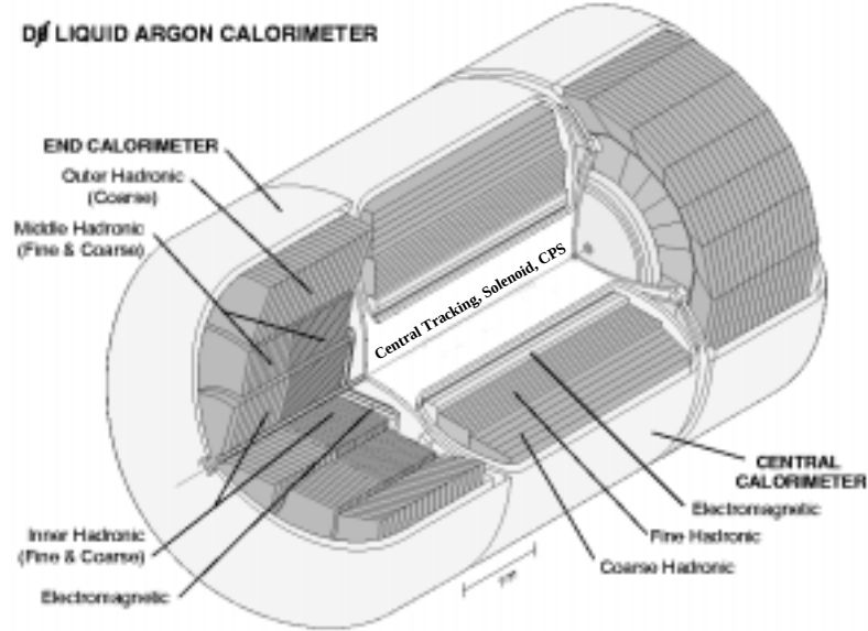
Figure 4.15: The D\bar{O} calorimeter.
