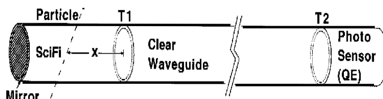
Figure 4.10: Schematic of a fiber-tracking element. T1 and T2 are the optical interfaces between scintillating fiber, clear waveguide and the VLPC.
