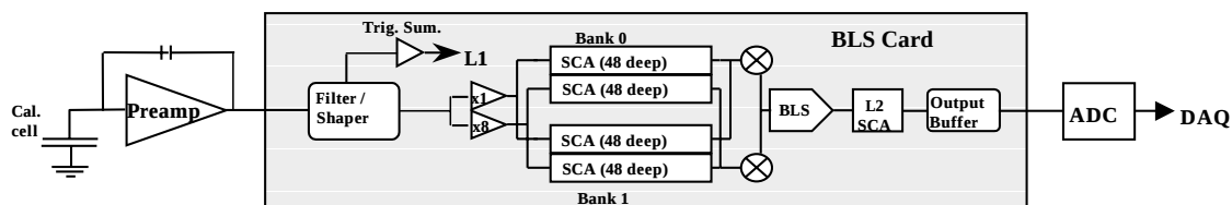
Figure 4.18: Schematic of the calorimeter readout electronics.
