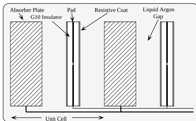
Figure 4.16: Schematic view of a calorimeter cell.
