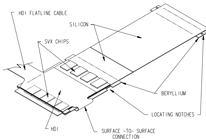
Figure 4.8: Layout of the ladder.
