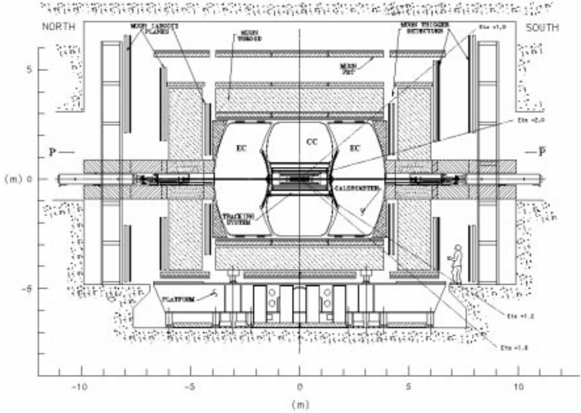
Figure 4.5: Side view of the DØ upgraded detector in Run II.
