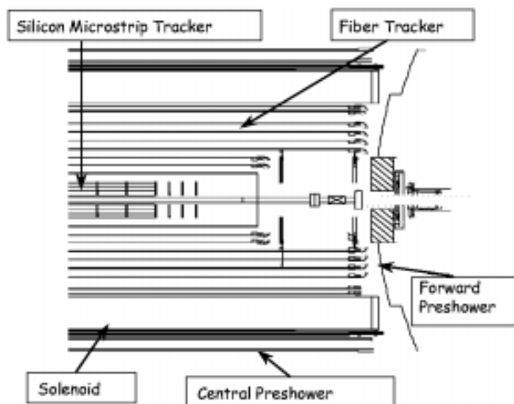
Figure 4.6: One-half side view of the central tracking system.
