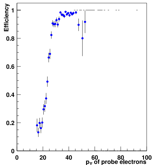
Figure 7.2: Trigger turn-on curve for EM_HL_SH or EM_MX_SH triggers.
