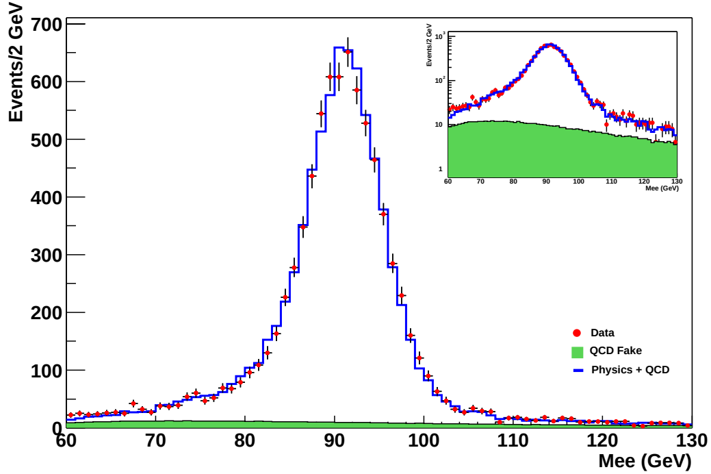
Figure 9.1: The invariant mass distribution of data (points) and expected background (line) for the Z peak region. The shading represents the QCD fake background. The insert is the same plot in log scale.
