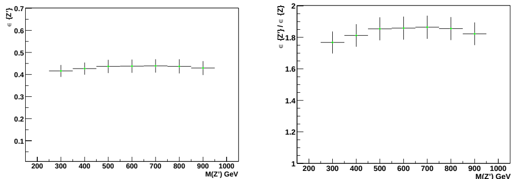
Figure 7.8: Overall efficiency \epsilon_{Z'} (left) and efficiency ratio \epsilon_{Z'}/\epsilon_Z (right) for Z' of various masses.
