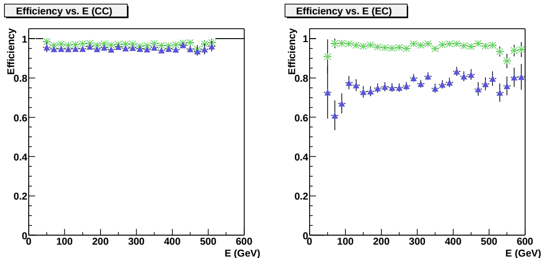
Figure 6.5: Efficiency (Monte Carlo based) of electron selection cuts as a function of electron energy for loose electrons (star) and tight electrons (triangle). The left plot is for CC electrons, and the right plot is for EC electrons.
