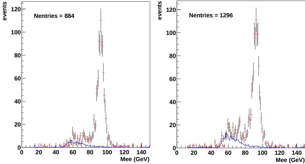
Figure 7.5: The 2(tt)+(tp) (left) and 2(tt)+(tp)+(tf) (right) distributions for ECEC events. The points are data. The line is the expected non-Z background.
