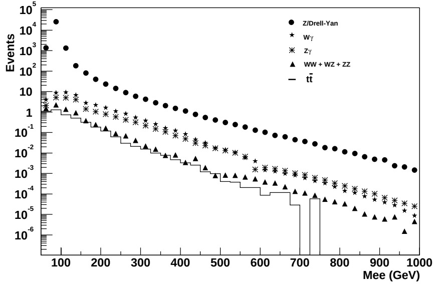
Figure 8.2: The invariant mass distribution from various physics processes.
