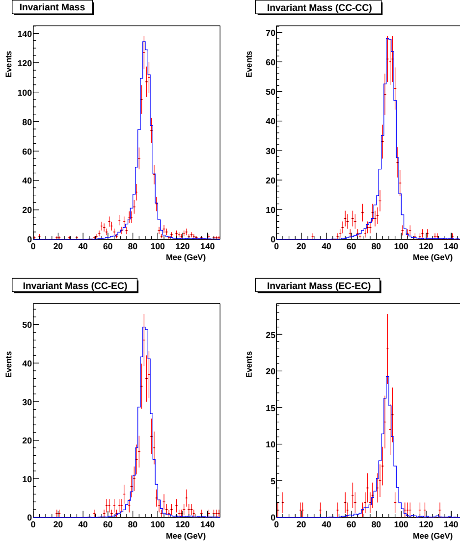
Figure 6.1: Comparison between PMCS (line) and data (dot) of the di-electron invariant mass distributions of Z \rightarrow ee events in various topologies: CC-CC (top right), CC-EC (bottom left), EC-EC (bottom right), and all three (top left).
