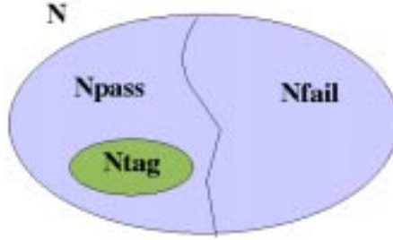
Figure 7.3: Illustration of sample sets used to measure the EMID efficiency.
