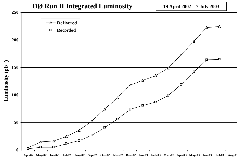
Figure 4.3: Integrated luminosity delivered to D\bar{O} and recorded by the D\bar{O} detector.
