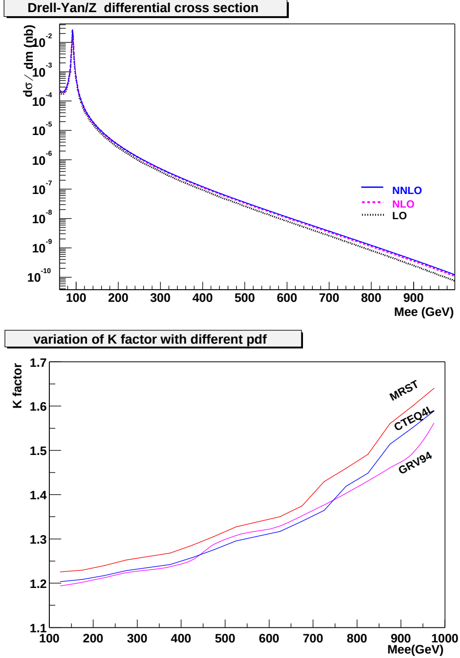
Figure 8.1: (upper) Z/Drell-Yan differential cross section at \sqrt{s} = 1.96 GeV; (lower) K-factor as a function of dielectron mass for various parton distribution functions: CTEQ4L, MRST, GRV94.
