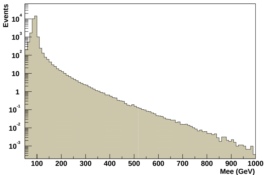
Figure 8.3: Expected dielectron mass spectrum from all physics processes.
