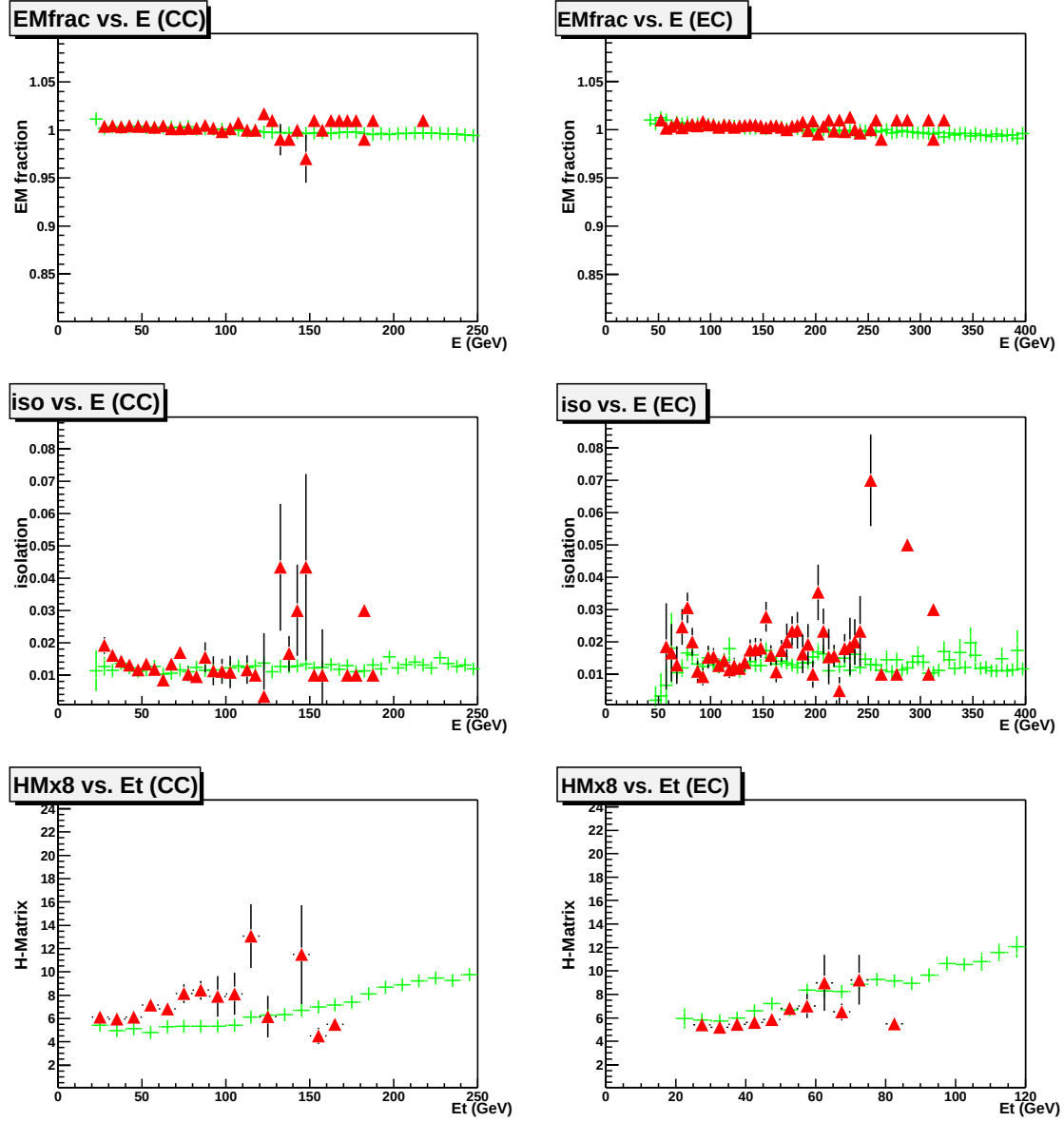
Figure 6.4: Comparison of the distribution of electron identification variables between electrons from Monte Carlo (plus sign) and electrons from data (triangle) for CC (left) and EC (right). Top to bottom: EM fraction, isolation and H-Matrix.
