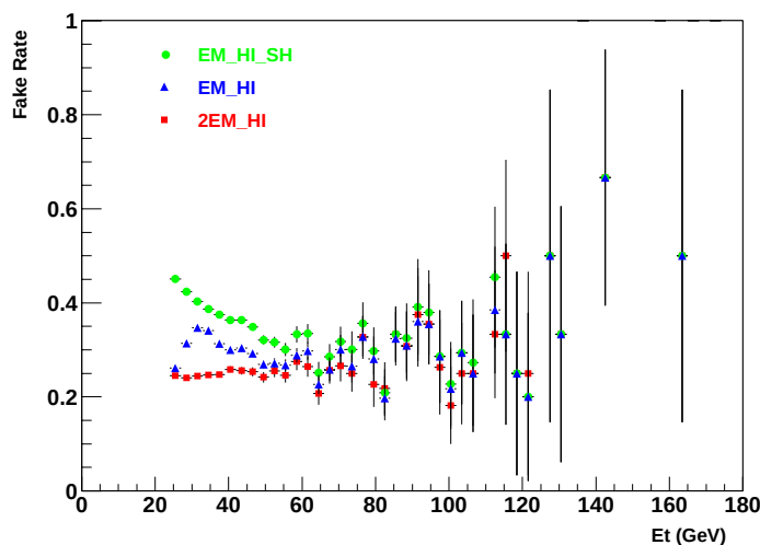
Figure 8.5: Fake rate using different triggers: EM\_HI\_SH (top), EM\_HI (middle) and 2EM\_HI (bottom)
