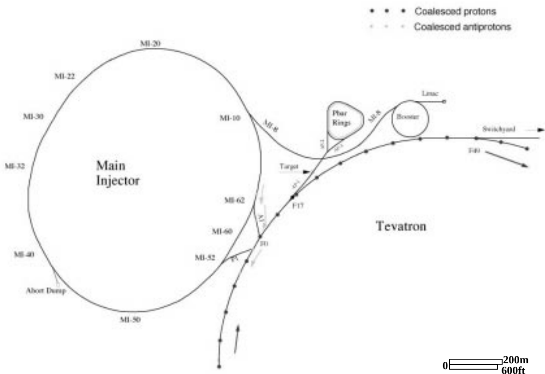
Figure 4.1: Fermilab Tevatron Collider complex.
