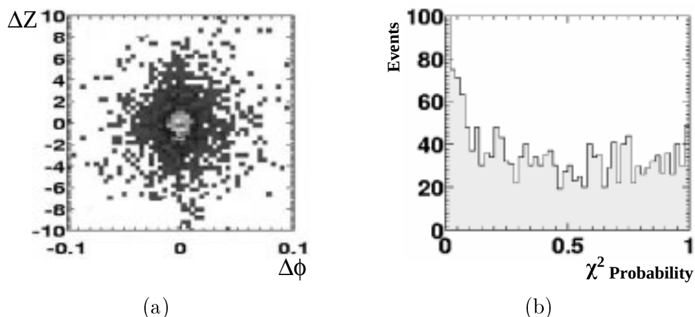
Figure 5.2: Distributions of track matching variables ( \Delta z vs. \Delta\phi ) (a) and distribution of the track match significance \chi^2 probability for electrons from Z \rightarrow e^+e^- decays (b).
