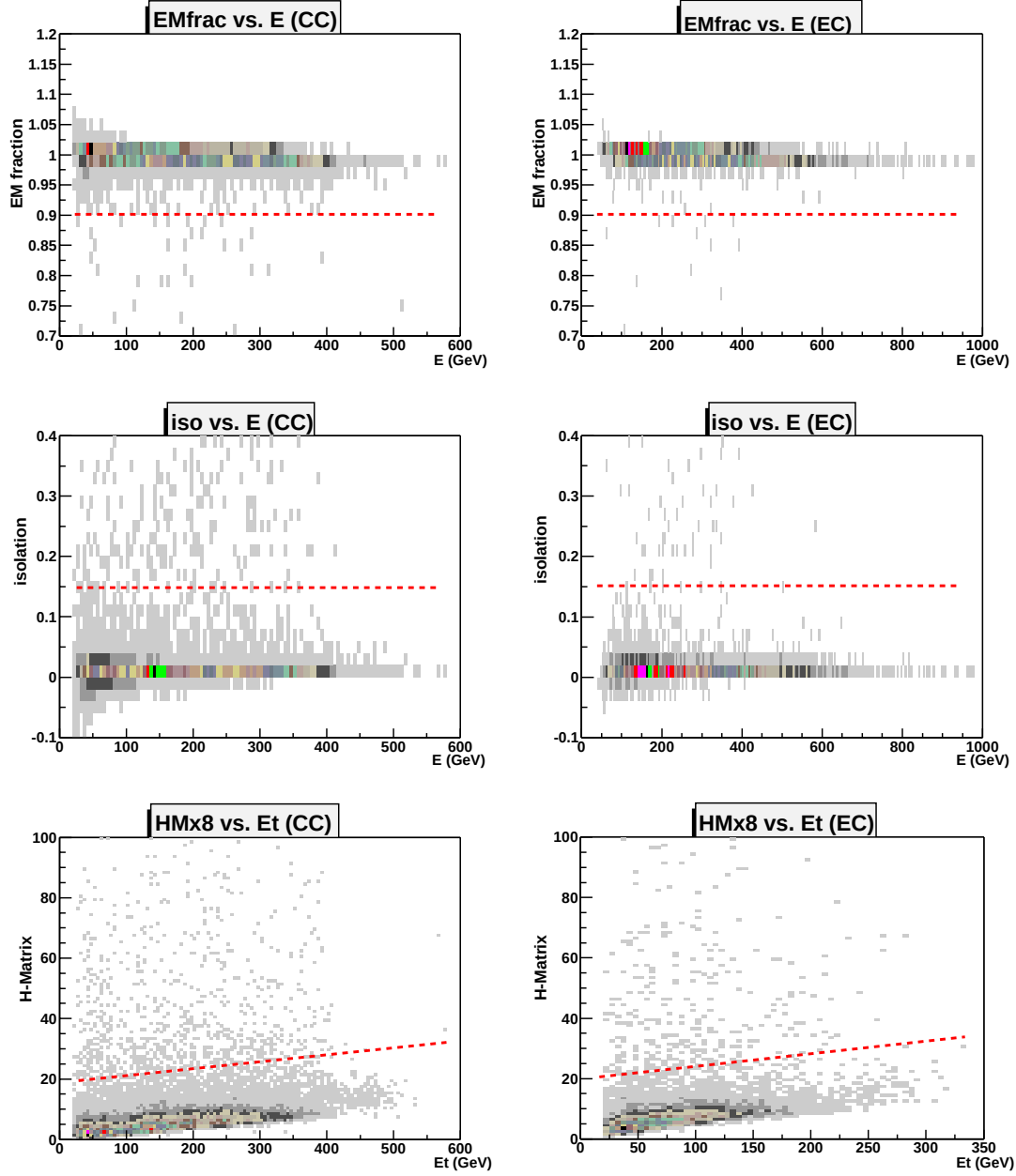
Figure 6.3: The distribution of electron identification variables (top to bottom: EM fraction, isolation and H-Matrix) as a function of electron energy for CC (left) and EC (right). The cuts used in this analysis are also shown.
