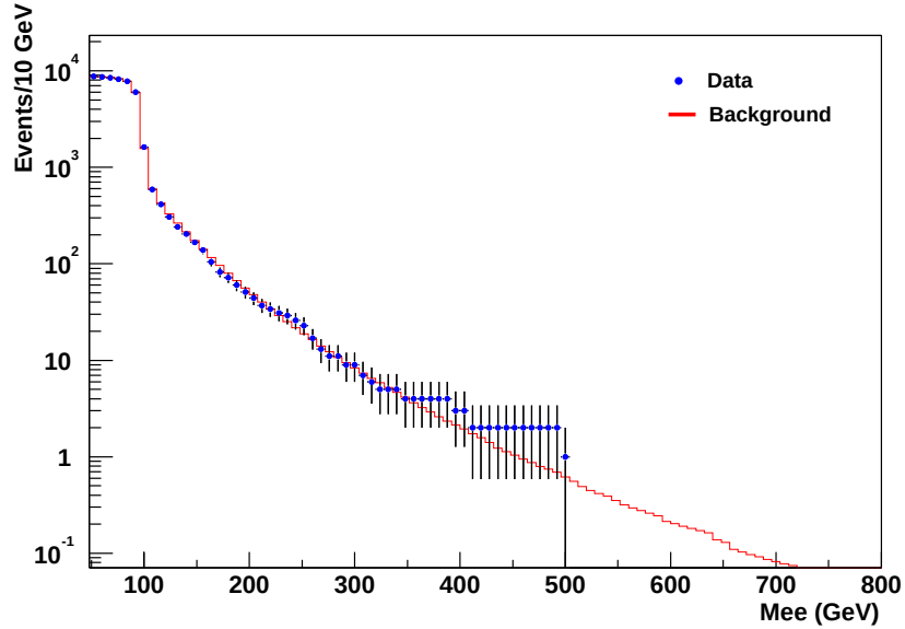
Figure 9.3: The integrated spectrum of data (points) and the expected background (line). At each mass value, the vertical axis corresponds to the total number of events with M_{ee} above that mass.
