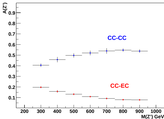
Figure 7.1: Acceptance \mathcal{A}_{Z'} for Z' of various masses.
