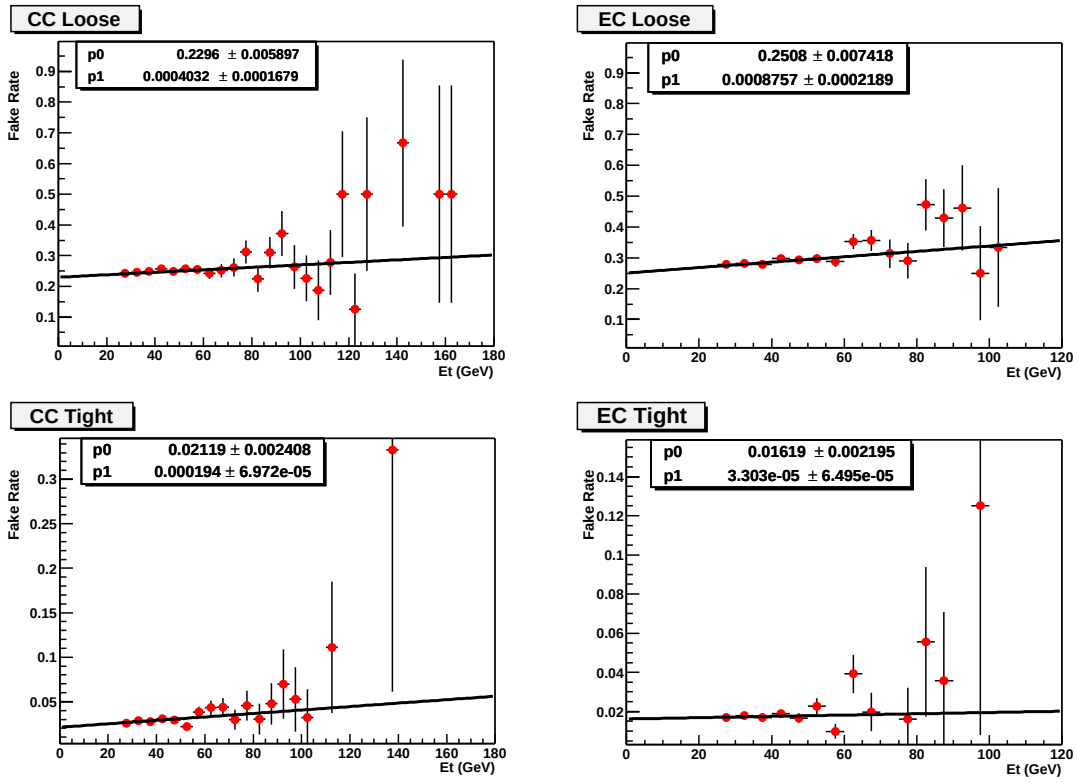
Figure 8.4: Fake rate as a function of EM object's E_T for passing “loose” cuts in CC (top left), “loose” cuts in EC (top right), “tight” cuts in CC (bottom left), and “tight” cuts in EC (bottom right).
