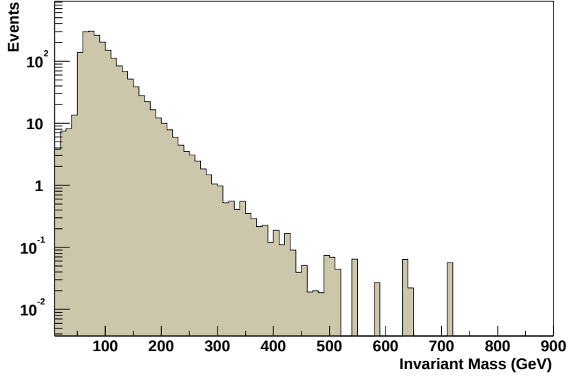
Figure 8.6: Invariant mass spectrum of QCD fake background.
