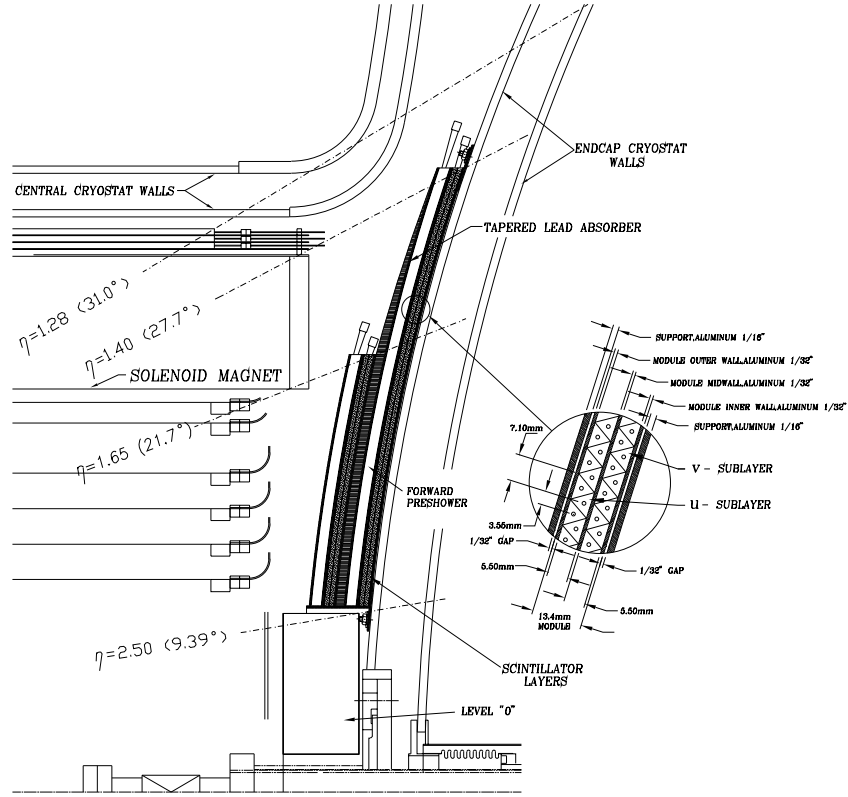
Figure 4.14: One quarter view of the Forward Preshower detector.
