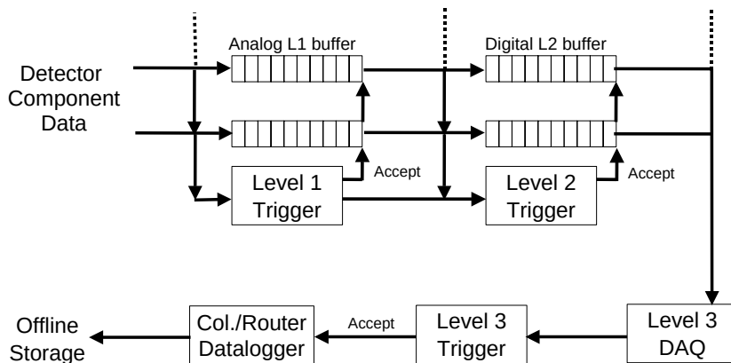
Figure 4.19: Schematic of the trigger and data acquisition system.
