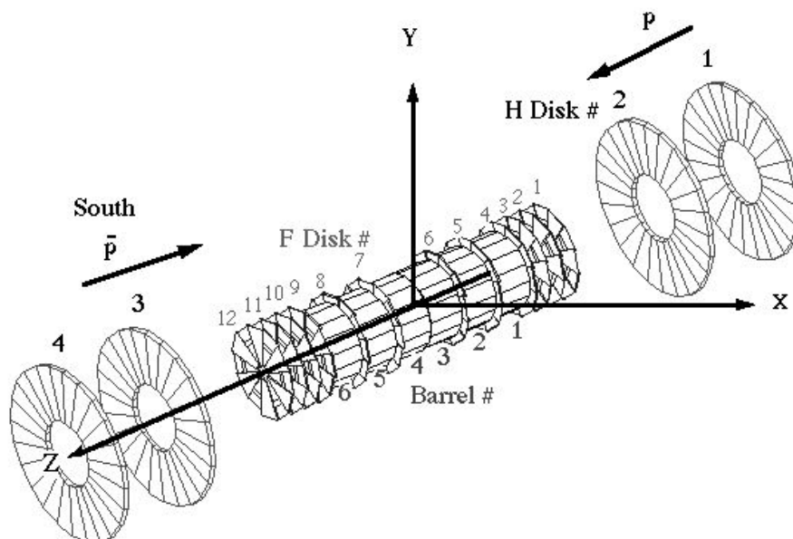
Figure 4.7: The silicon microstrip tracker.
