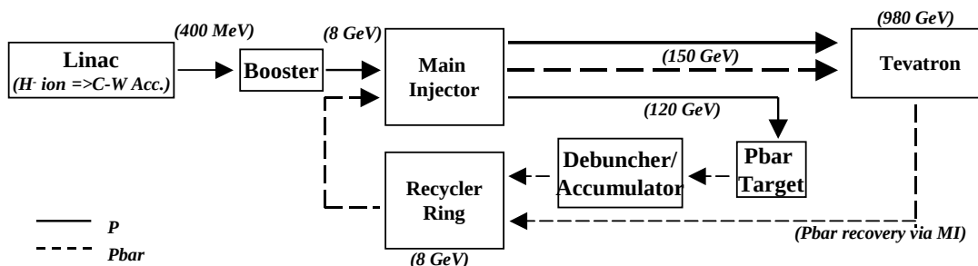
Figure 4.2: A schematic view of the Tevatron operation.
