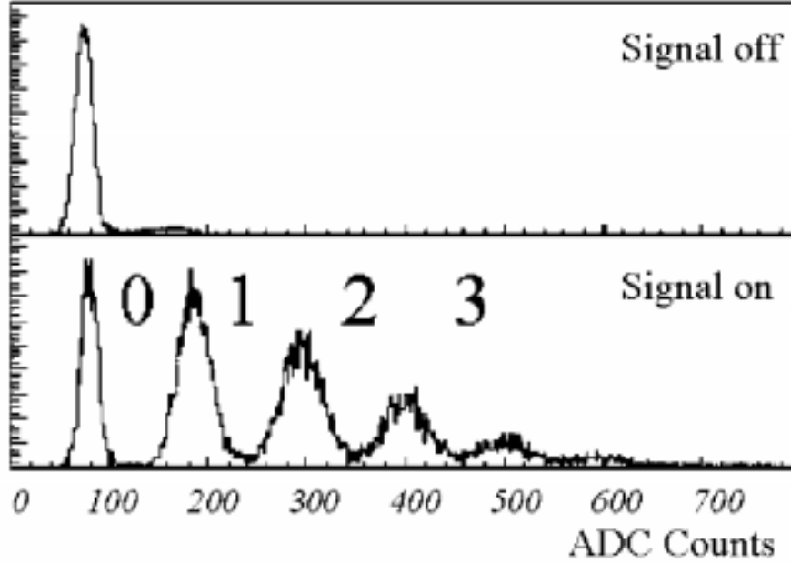
Figure 4.11: Spectrum from a VLPC when there is no signal and when there are signals.
