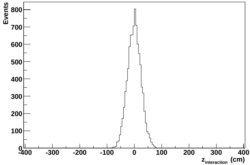
Figure 4.4: Distribution of the interaction point in z -axis.
