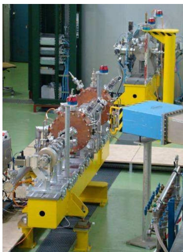
From left, clockwise: the chopper beam line installed at CERN, the 1 MW test stand for superconducting cavities at CEA Saclay, a chopper structure
