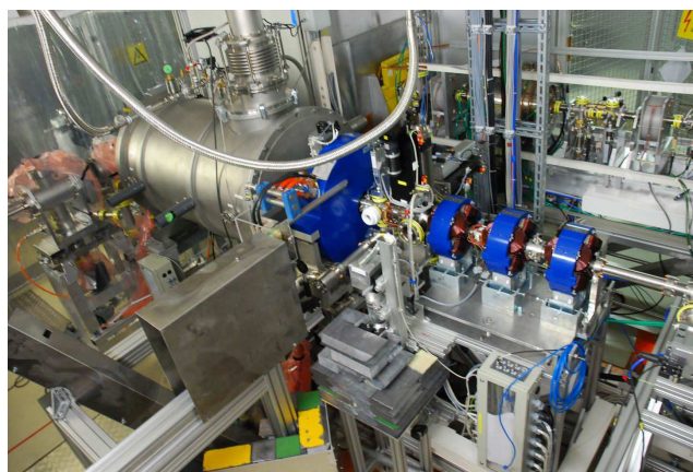
Figure 5: SRF photoinjector in the ELBE accelerator hall.
