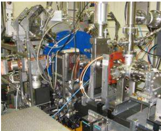
Figure 1: Layout of the PHIN CTF3 line
