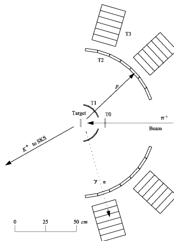
Fig. 7. The schematic view of the neutral particle detection system of the experiment E369 is shown. Neutron energy is measured with the time of flight between T0 and T3.
