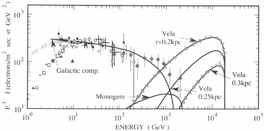
Fig. 4. Compiled cosmic ray electron data and predictions for two nearby sources (adapted from [40]).
