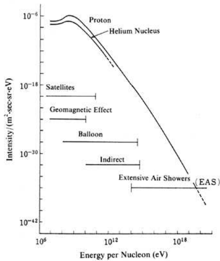
Fig. 1. Schematic representation of the cosmic ray energy spectrum and modes of measurement. (Adapted from [3].)
