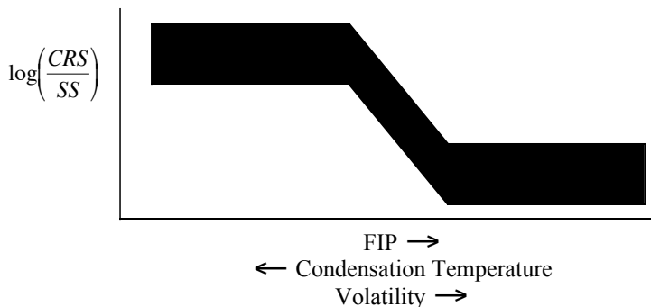
Fig.3. Schematic representation of the First Ionization Potential dependence of the cosmic ray source to solar system relative abundance ratio. Other parameters that correlate with FIP are indicated.
