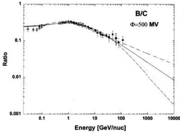
Fig. 2. Compilation of measurements of the B/C ratio as a function of kinetic energy. Curves are fits from different propagation models extrapolated to high energy.
