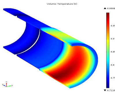
Figure 3: Peak PS coil temperature.
