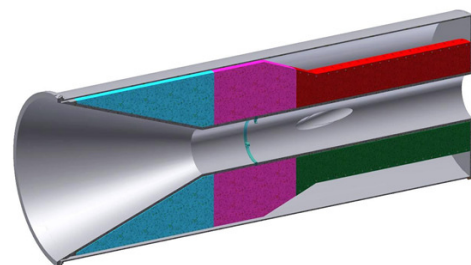
Figure 5: Section view of HRS. Bronze pieces are shown in light blue, purple and red. A stainless steel liner surrounds the bronze on all sides and the vessel holds 600 gallons of water.
