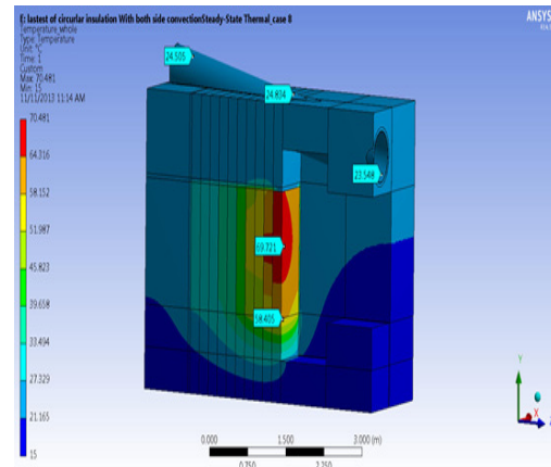
Figure 6: Temperature distribution in the absorber steel and shielding concrete for normal operation.
