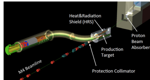
Figure 1: Target station layout.
