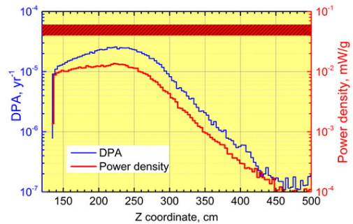
Figure 4: The MARS results for the peak DPA and peak power density at the PS coils.
