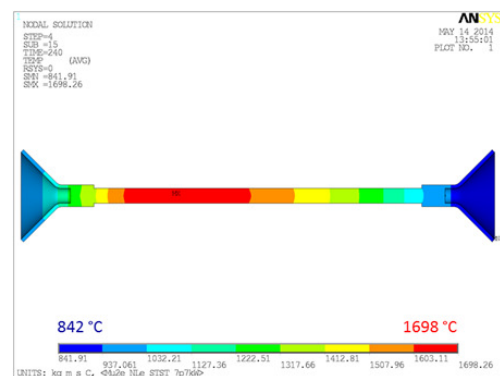
Figure 2: Target steady-state operating temperature assuming a heat load of 560 W and temperature dependent literature values for thermal emissivity.
