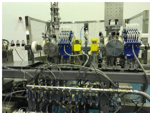
Figure 8: Assembled XiPAF LEBT at site.
