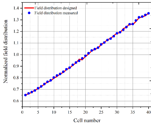
Figure 3: Field distribution of the CPHS DTL after the final tuning.
