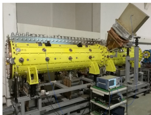
Figure 2: Assembled CPHS DTL for RF measurement.
