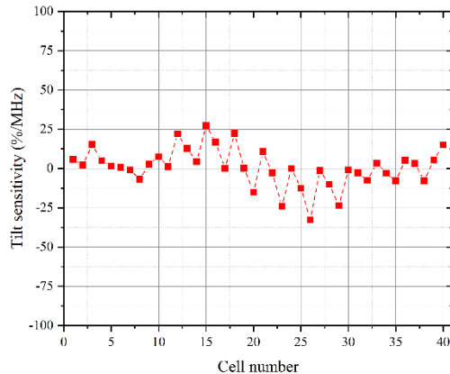
Figure 4: Tilt sensitivity of the CPHS DTL after the final tuning.
