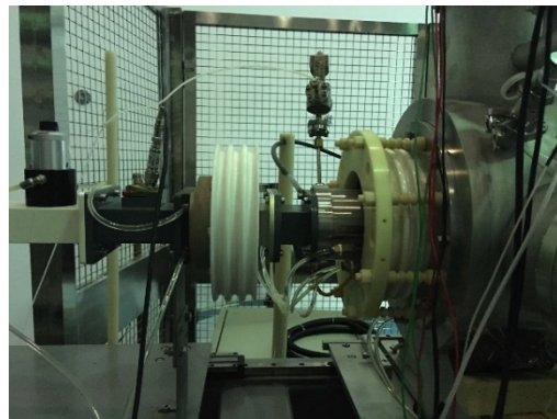
Figure 6: Assembled H - ECR source at site for XiPAF.
