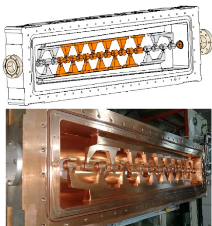
Figure 11: Central frame of the IH-DTL cavity.
