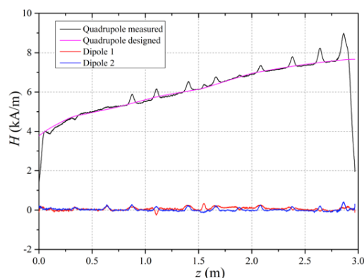
Figure 10: Field distribution of the quadrupole and dipole modes after the tuning.
