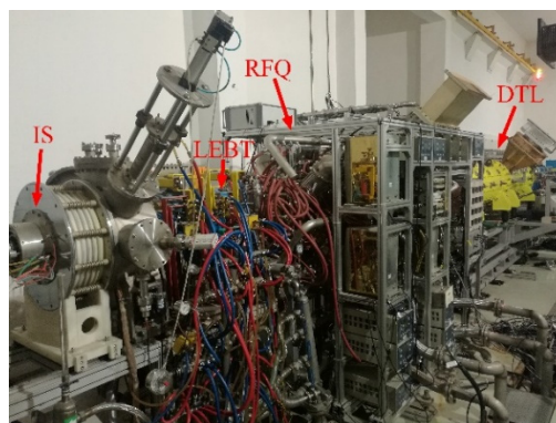
Figure 1: Layout of the linac of the compact pulsed hadron source.
