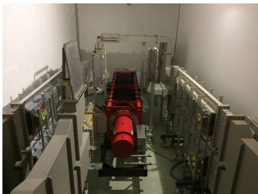
Figure 5: RF power system for the CPHS RFQ and DTL.
