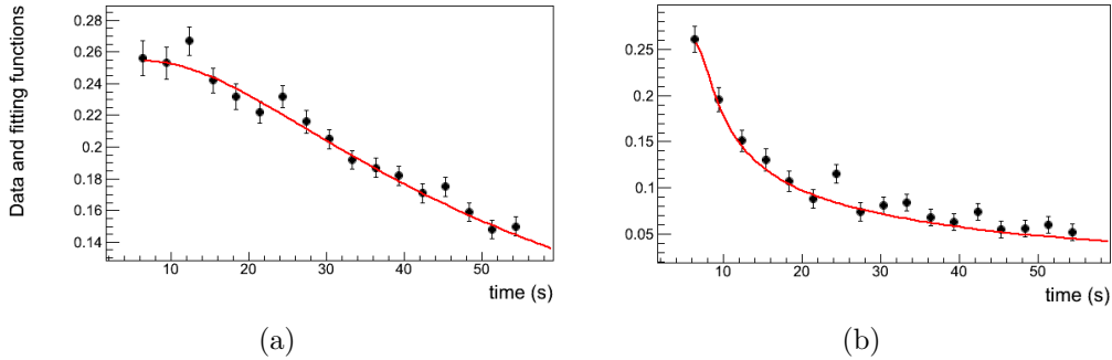
Figure 5.7: Comparison of the horizontal polarization as a function of time for a narrow beam (see Fig. 5.7(a)) and a wide beam (see Fig. 5.7(b)) for MXS=0%. It is evident how emittance affects the spin coherence time, which is 50.0 \pm 2.5 s in the first case and 5.5 \pm 0.6 s in the second one.
