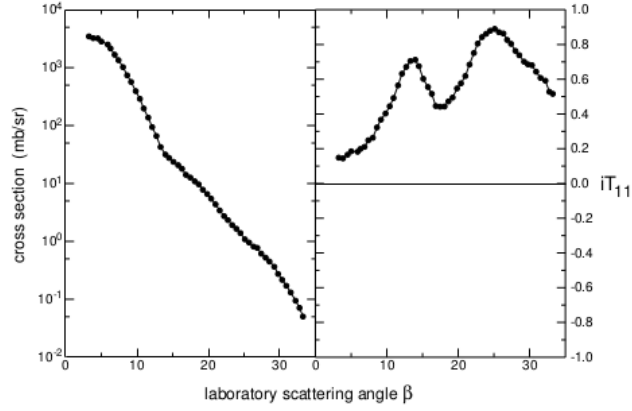
Figure 3.6: Deuteron elastic scattering cross section and vector analyzing power iT_{11} at 270 MeV [22].
