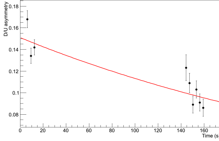
Figure 5.9: Measurements of the spin coherence time for a electron cooled beam. Due to the lack of polarization values in the gap, the polarization lifetime is defined as the time required for the polarization to fall to 1/e of its initial value and corresponds to 316 \pm 40 s.
