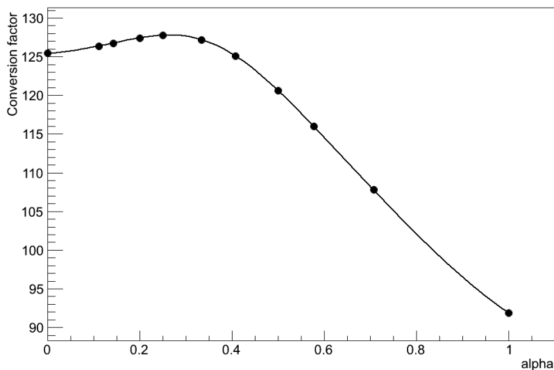
Figure 5.3: This plot shows the conversion factor for a_2 into seconds as a function of the template curve shape \alpha and for a particular choice of the fixed array t_{\text{tab}} . For our choice of the definition of the spin coherence time, it is desirable that a_2 should be independent from \alpha and all the template curves should cross p=0.606 at the same time. As is clear from this graph this is not the case, in particular for value above \alpha = 0.3 . So the conversion factor becomes a slowly varying function of \alpha .
