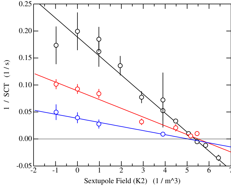
Figure 5.8: Measurements of the reciprocal of spin coherence time. The horizontal scale is the MXS sextupole magnetic field strength. The three lines correspond to three different beam profile widths, starting from a narrow (bottom, blue) to a wide (top, black) profile. In order to determine whether this behavior is linear, all the points above the zero crossing at 5.4 \pm 0.1 \text{ m}^{-3} were reversed in sign.
