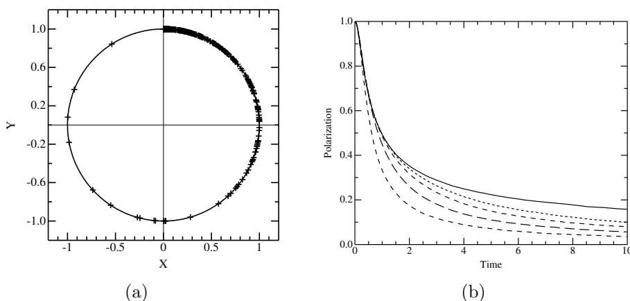
Figure 5.2: Figure 5.2(a) shows the unit circle in the xy plane where the spins are distributed following the square of a Gaussian distribution. It represents the spin positions in the plane at one time. Figure 5.2(b) shows five example of the numerical function used to describe the horizontal polarization as a function of time. These curves have the same properties except for the \alpha value which is equal to 1, 1/2, 1/3, 1/4 and 0 (starting from the bottom). \alpha = 0 means that the beam is horizontal and flat because the vertical size is zero. \alpha = 1 is a round beam, the case in which the beam emittance effect on polarization is the largest with a fixed \sigma_x .
