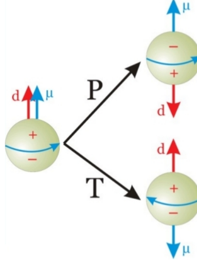
Figure 1.1: A particle with an EDM \vec{d} parallel to its spin \vec{\mu} is shown on the left side. An inversion through the origin, parity ( P ) reverses the EDM sign and leaves the spin direction unchanged. A time reversal operation T transforms the original particle into one with the same EDM but opposite spin direction. A rotation of 180^\circ illustrates that the particles depicted on right side are the same and unlike the particle on the left. Thus, violation of P and T can be seen as changing a particle with an EDM parallel to the spin direction into one whose EDM direction is antiparallel.
