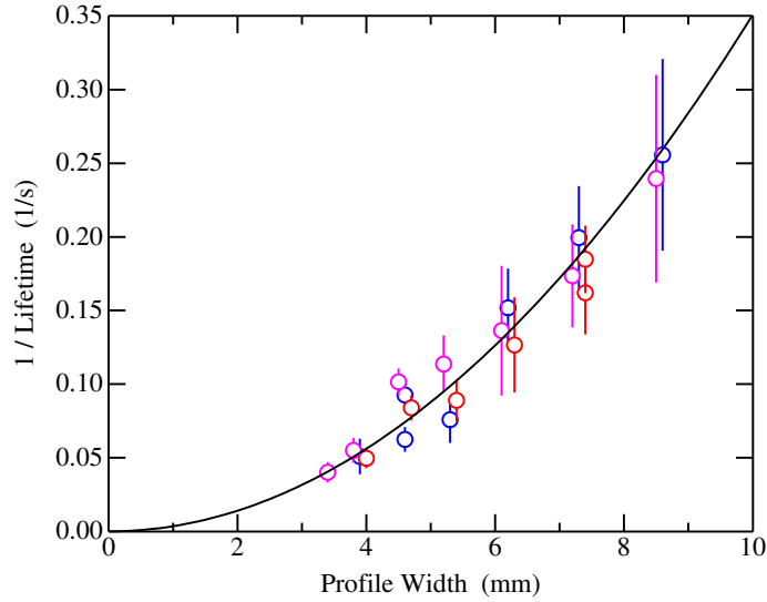
Figure 5.6: This figure shows part of the data recorded for several horizontal profile widths. All the data points were taken with electron cooling off, following a period with cooling on to reduce the phase space size with another short period of heating to expand the space horizontally. The blue circles are the data recorded without sextupole field corrections (MXS=0%, see next section), the red circles with MXS=5%, and the magenta circles with MXS=-5%. The position is staggered horizontally so that all these points do not overlap (5% and -5% appear at profiles +0.1 mm and -0.1 mm). The black line through the data is only a guide to the eye to suggest that a quadratic dependence is reasonable.
