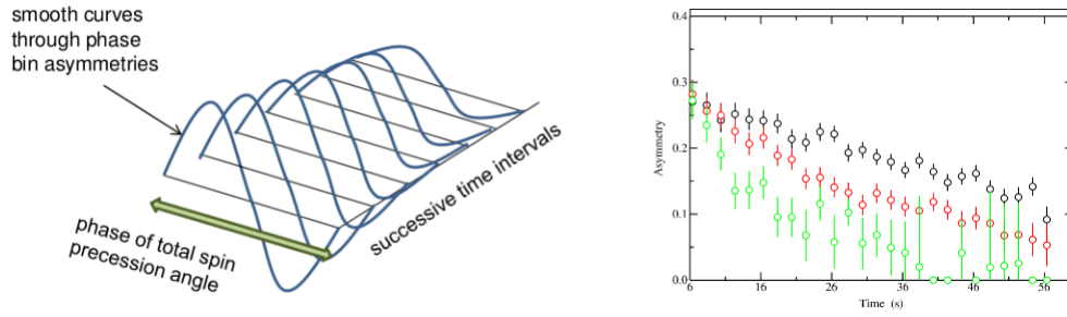
Figure 3.8: Sketch of the procedure to extract the horizontal polarization as a function of time from the total spin precession angle. On the left panel are sine waves that represent the asymmetries in the circle of the total spin precession angle. The circle is divided in 9 bins and collects the events in a 3 second time window, according to the phase of the total precession angle in the horizontal plane. On the right panel there is one example of the horizontal polarization measurement for three different beam emittances from a large (green) to a small (black) size. Each point of these curves corresponds to the amplitude of the sine wave, corrected for the “positivity” effect.
