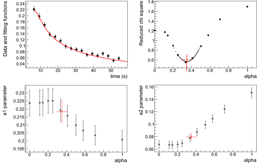
Figure 5.5: The four graphs show an example of the fitting procedure to calculate the spin coherence time. Starting from the top left corner, the experimental data are the black dots and the solid red line is the final result of the analysis. In the upper right panel, the reduced chi square resulting from the fitting procedure of the template curves is plotted against the corresponding \alpha value. The best \alpha (shown by a vertical solid red line) is determined by the minimum of a quadratic curve fitting the smallest reduced chi square points. In the bottom graphs, the values of the fitting parameters a_1 and a_2 are shown for each \alpha . The red stars in these plots are the a_1 and a_2 values corresponding to the best \alpha . For this set of measurement, the best value of \alpha is 0.35 \pm 0.05 and the fitting parameters are a_1 = 0.218 \pm 0.007 and a_2 = 0.080 \pm 0.005 . The conversion factor is 126.86 and the spin coherence time is \tau_{SCT} = 10.15 \pm 0.6 s.
