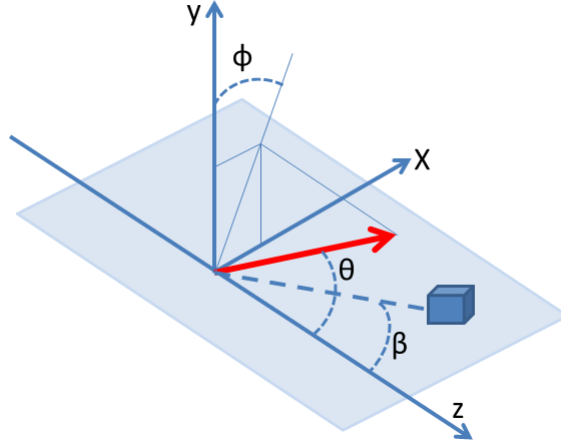
Figure 3.3: The coordinate system for polarization direction (red arrow) based on the observation of a reaction product in a detector (small box). The beam travels along the \hat{z} axis. The detector position at angle \beta defines, along with the beam, the reaction plane and positive \hat{x} . The quantization axis for the polarization (red arrow) lies in a direction given by the polar angles \theta and \phi (as measured from \hat{y} axis).
