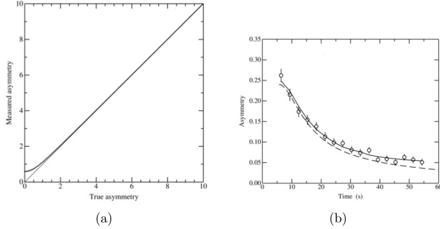
Figure 5.4: Figure 5.4(a) shows a Monte Carlo simulation relating the observed asymmetry to the real asymmetry. The asymmetry scale is adjusted so that one unit represents the size of the statistical error in one angle bin for one time bin in one store. The positive bias problem becomes evident when the real asymmetry goes to zero and the error is about the size of the typical signal. Figure 5.4(b) is an example of the correction for a real case. The empty circles are the uncorrected data. The real polarization which corresponds to the data is represented by the dashed line. The real polarization with the positive bias included is the solid line.
