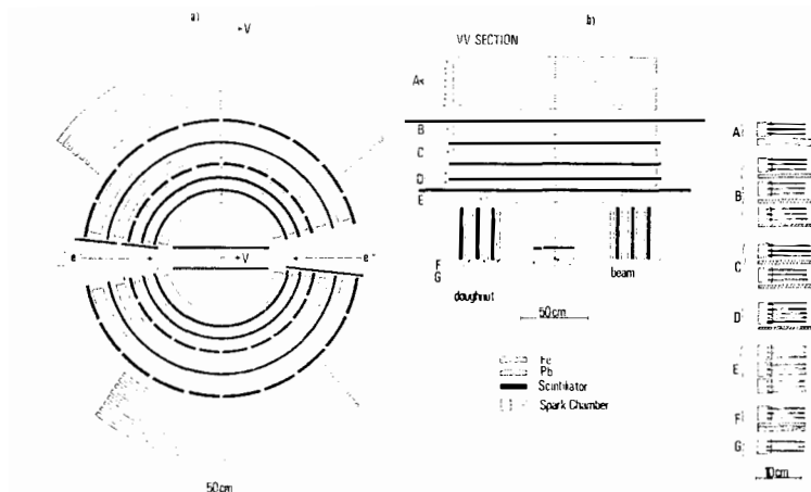
FIG. 1 - \gamma\gamma 2 experimental set-up. a) Front view from the center of Adone; b) vertical section in the plane normal to the beams (For the sake of clearness, the side telescopes are not shown in the front view of the apparatus).
