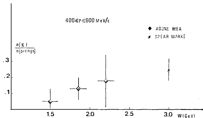
FIG. 7 - Ratio between the numbers of K and prongs whose momentum falls in the range 400 \leq p \leq 600 \text{ MeV}/c .
