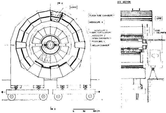
FIG. 4 - BB experimental set-up.
