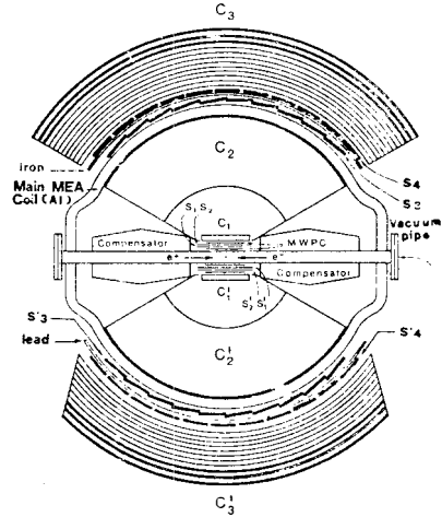
FIG. 3 - MEA experimental set-up (vertical section). C_1 , C_1' are narrow gap spark chambers; C_2 , C_2' are wide gap cylindrical spark chambers for momentum analysis; C_3 , C_3' are thick plate spark chambers for particle identification. MWPC are multiwire proportional chambers; S_1, S_1', \dots, S_4, S_4' are scintillation counters.
