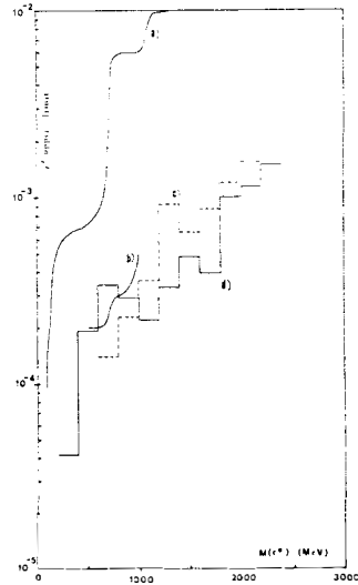
FIG. 6 - Upper limit (95% confidence level) on \sigma^2 versus the e^+e^- mass: a) Ref. (5); b) Ref. (6); c) Due to a trivial error, the results reported in Fig. 4 of Ref. (7) are not correct. Here we report the corrected values; d) Present results.
