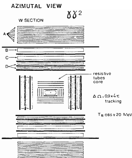
FIG. 2 - Vertical section of the modified \gamma\gamma apparatus.
