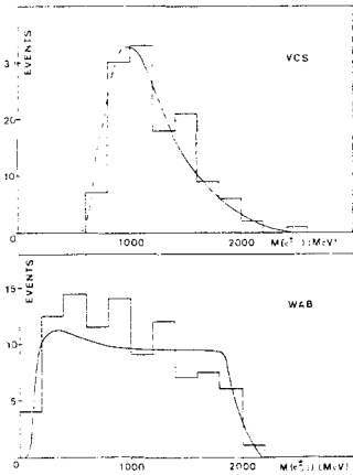
FIG. 5 - Effective mass distribution of the wide-angle ( e^+e^- ) systems: a) for CS events, with the e^\mp in the tagging counters; b) for WAB events, with all the e^+ , e^- , in the wide-angle apparatus. The solid lines are absolute QED predictions.
