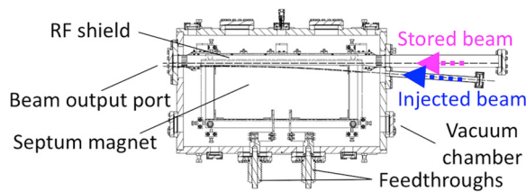
Figure 5: Schematic of in-vacuum pulse septum magnet.
