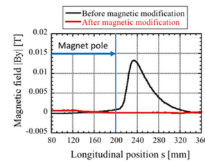
Figure 4: Measured stray magnetic field of the DC septum magnet.
