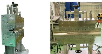
Figure 2: PM-based DC septum magnet.
