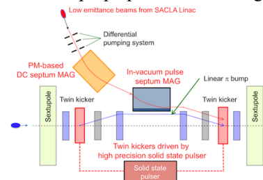
Figure 1: Schematic of in-vacuum transparent off-axis beam injection.
