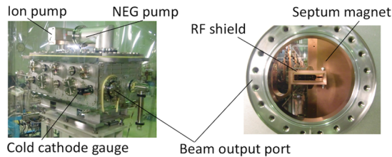
Figure 6: In-vacuum pulse septum magnet.
