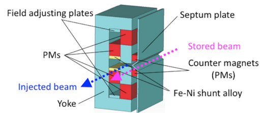
Figure 3: Magnetic circuit of the PM-based DC septum magnet.
