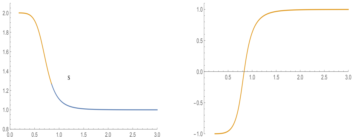
Figure 1. Solutions y(a) for \Omega_0 = \Omega_6 = 1 , \Omega_2 = 0 , \Omega_3 = \Omega_4 = 0 and for \zeta = 6 (left panel) or \zeta = -3 (right panel).
