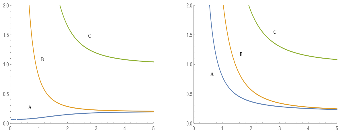
Figure 3. Solutions y(a) for \Omega_0 = \Omega_6 = 1 , \Omega_3 = 5 , \Omega_4 = 0 , \zeta = 0.2 . One has \Omega_2 = 0 (left) and \Omega_2 = 1 (right).
