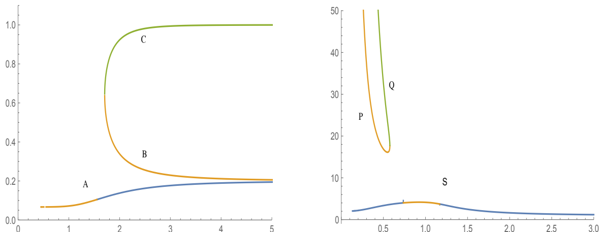
Figure 2. Solutions y(a) for \Omega_0 = \Omega_6 = 1 , \Omega_2 = 0 , \Omega_3 = \Omega_4 = 0 , \zeta = 0.2 (left) and for \Omega_0 = \Omega_6 = 1 , \Omega_2 = 0 , \Omega_3 = 5 , \Omega_4 = 0 , \zeta = 6 (right).
