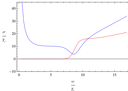
Figure 4. Conductivity for \alpha = 0.1 case.
