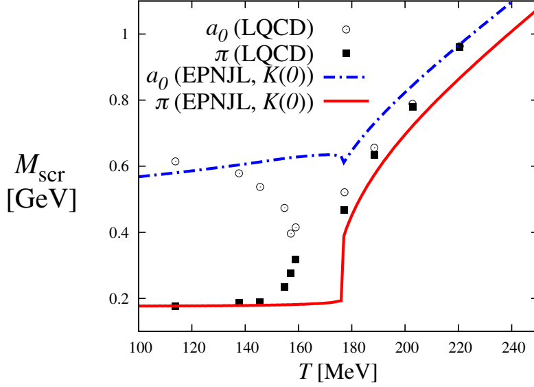
Fig. 3.5: Effects of T -dependent KMT interaction on pion and a_0 -meson screening masses. The solid (dot-dash) line denotes M_\pi^{\text{scr}} ( M_{a_0}^{\text{scr}} ) calculated by the EPNJL model with K(T) = K(0) . See Fig. 3.2 for LQCD data.
