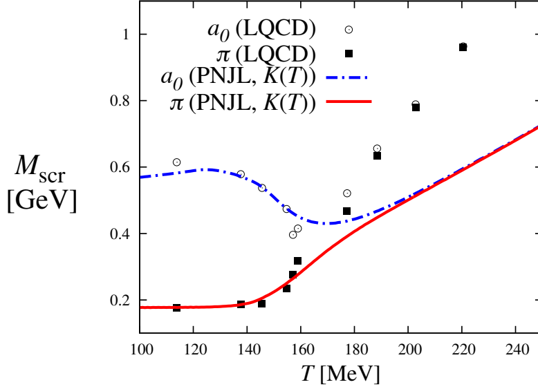
Fig. 3.3: Effects of T -dependent KMT interaction on pion and a_0 -meson screening masses. The solid (dot-dash) line denotes M_\pi^{\text{scr}} ( M_{a_0}^{\text{scr}} ) calculated by the PNJL model with T -dependent coupling K(T) . See Fig. 3.2 for LQCD data.
