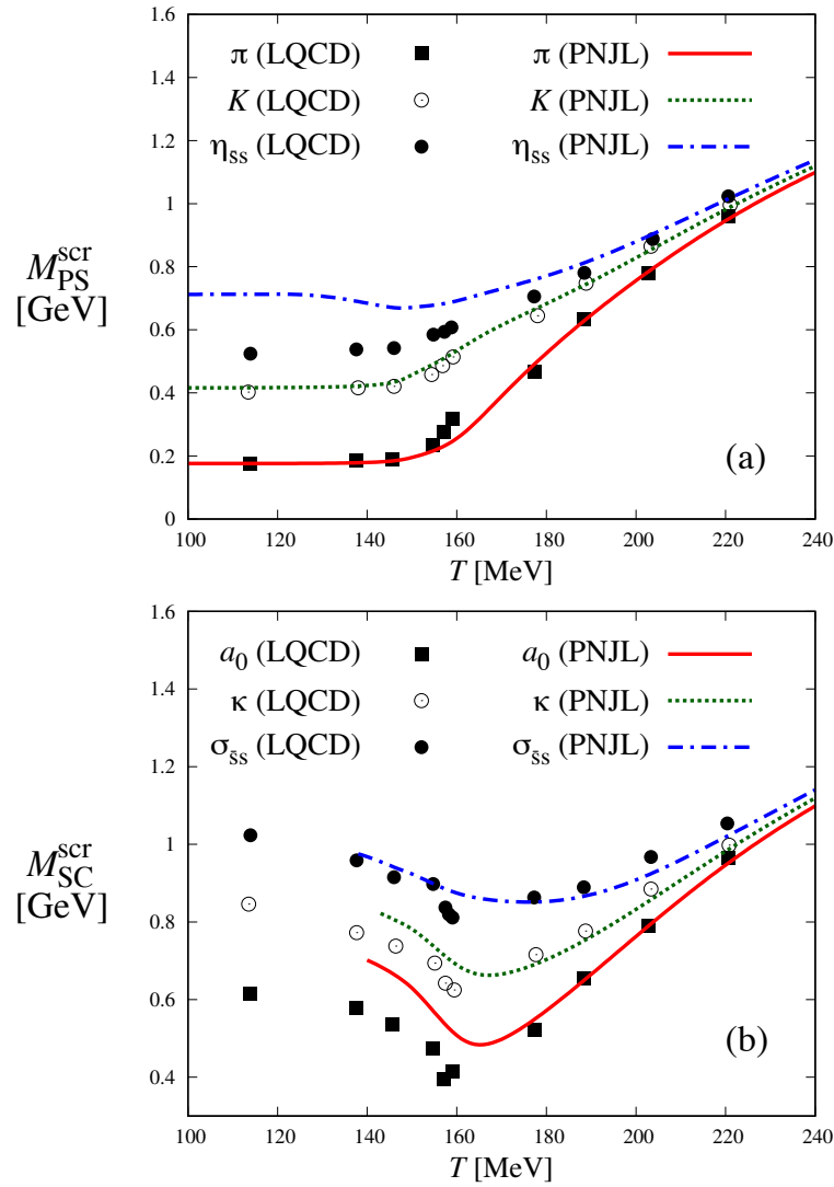
Fig. 4.2: T dependence of meson screening masses for (a) pseudoscalar mesons \pi, K, \eta_{ss} and (b) scalar mesons a_0, \kappa, \sigma_{ss} . Model results are denoted by lines and LQCD data are by symbols. The parameter set (B) is taken in model calculations. LQCD data are taken from Ref. [30].
