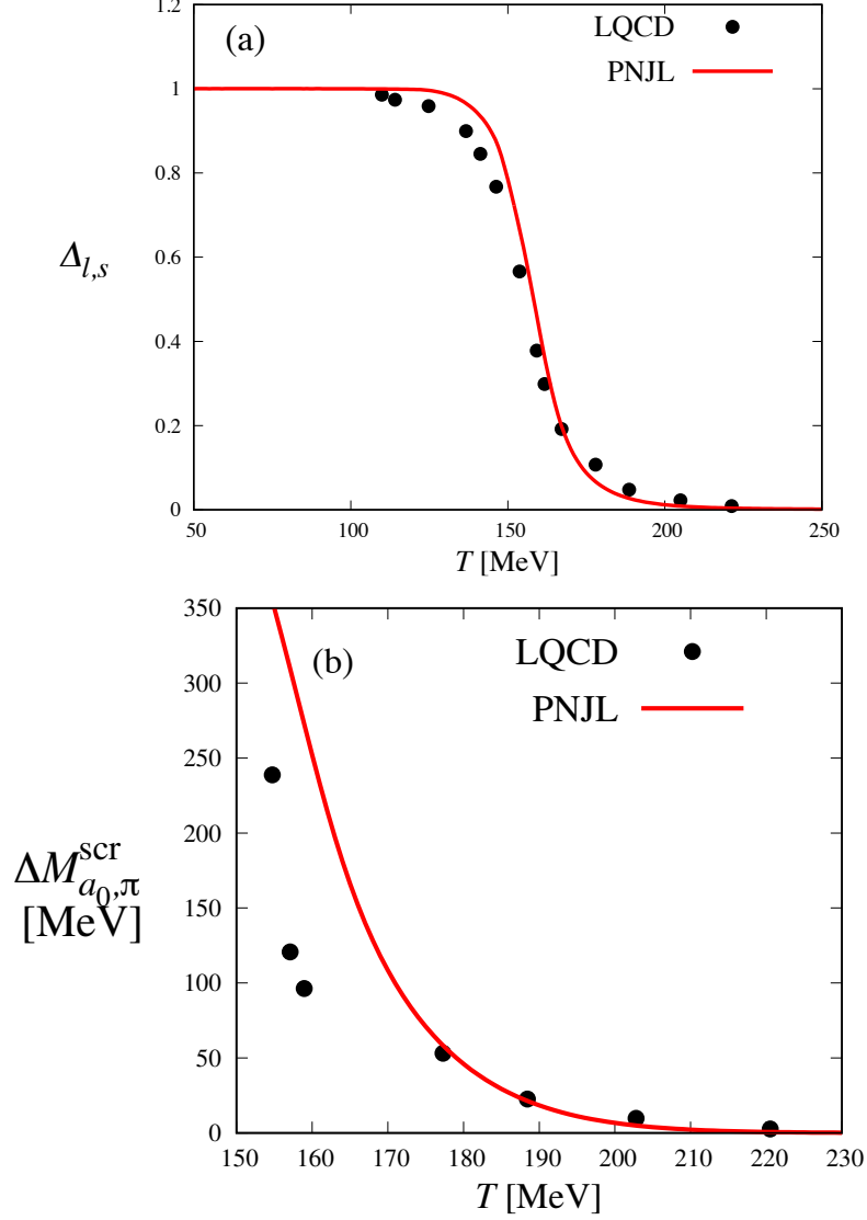
Fig. 4.1: T dependence of (a) \Delta_{l,s} and (b) \Delta M_{a_0,\pi}^{\text{scr}} . Model results are shown by solid lines, while LQCD data are denoted by closed circles. The parameter set (B) is taken in model calculations. LQCD data are taken from Refs. [30, 70].
