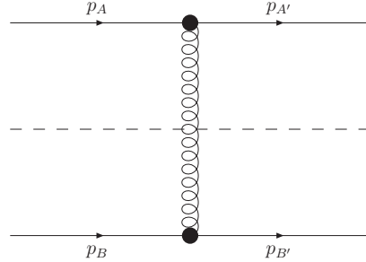
Fig. 3. The t -channel discontinuity of the amplitude of the process A + B \rightarrow A' + B' .
