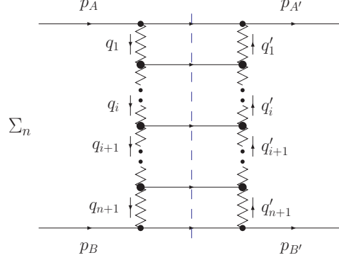
Fig. 5. The s -channel discontinuity of the amplitude of the process A+B \rightarrow A'+B' .
