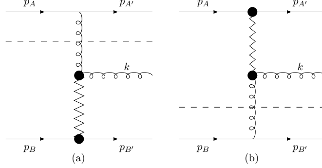
Fig. 4. Schematic representation of the discontinuities of the A + B \rightarrow A' + G + B' amplitude in the t_1 (a) and t_2 (b) channels.
