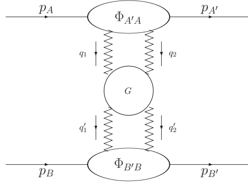
Fig. 6. Schematic representation of the process A + B \rightarrow A' + A' .
