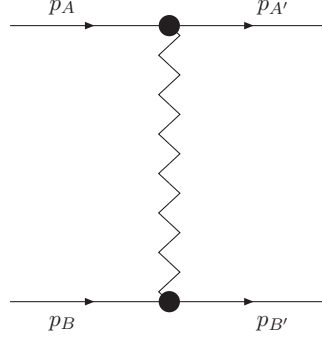
Fig. 1. The process A + B \rightarrow A' + B' with the gluon quantum numbers and negative signature. The zig-zag line represents reggeized gluon exchange.
