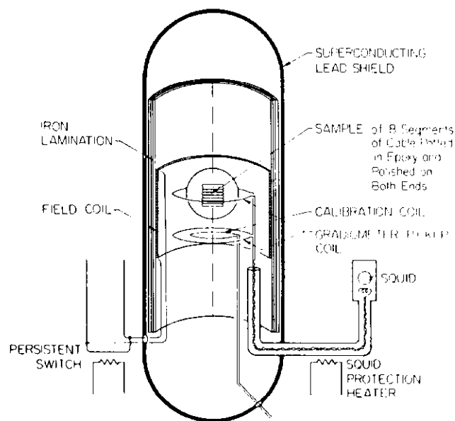
Figure 1. Schematic of measuring apparatus.
