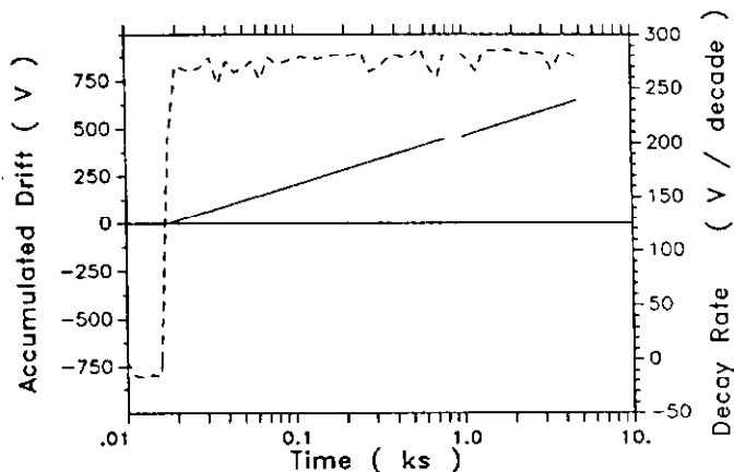
Figure 2. A typical flux creep data point. The solid lines are the processed pickup signal, and the dashed lines their slope.
