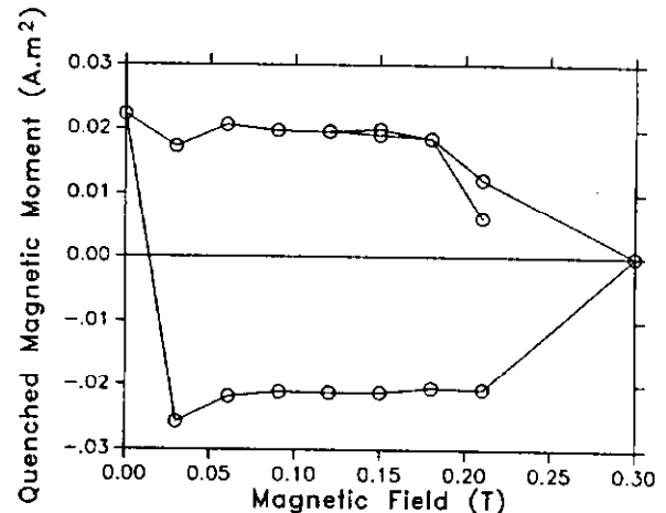
Figure 5. Total magnetic moment change corresponding to pulses in figure 4.
