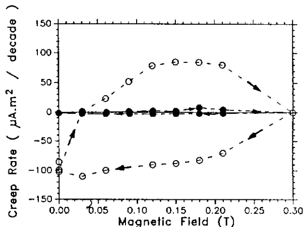
Figure 3. Magnetic Moment creep rate data in a systematic sequence of magnetic fields with (open circles) and without (closed circles) a sample of Tevatron cable.
