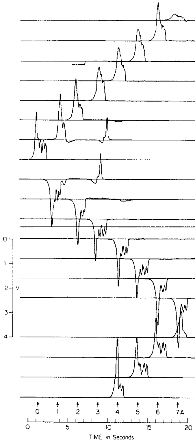
Figure 4. Pulses due to heating the sample above the critical temperature. Two additional pulses are due to the sample cooling back in fields below H_{c1} .
