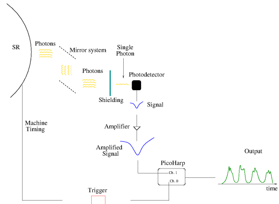
Figure 1: Sketch of the TCSPC set-up.
