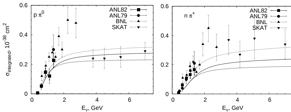
Fig. 5. Integrated cross section for the \mu^- p \pi^0 and \mu^- n \pi^+ final states.
