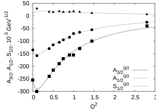
Fig. 4. Helicity amplitudes for the P_{33}(1232) resonance, calculated with the form-factors from Eq. (3.14).
