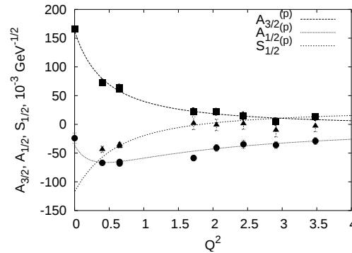
Fig. 3. Helicity amplitudes for the D_{13}(1520) resonance, calculated with the form-factors from Eq. (3.12).
