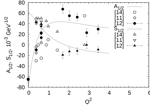
Fig. 2. Helicity amplitudes for the P_{11}(1440) resonance, calculated with the form-factors from Eq. (3.10).
