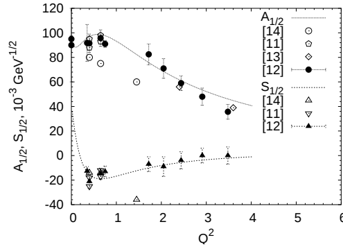
Fig. 1. Helicity amplitudes for the S_{11}(1535) resonance, calculated with the form-factors from Eq. (3.5).
