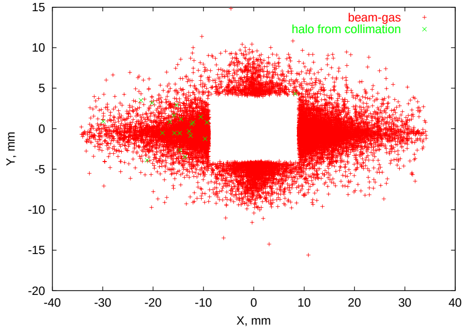
Figure 19: Proton hits at the “double L-shape” A48 collimator from elastic beam-gas interactions in the ring (red pluses) and tails from the main collimators (green crosses).
