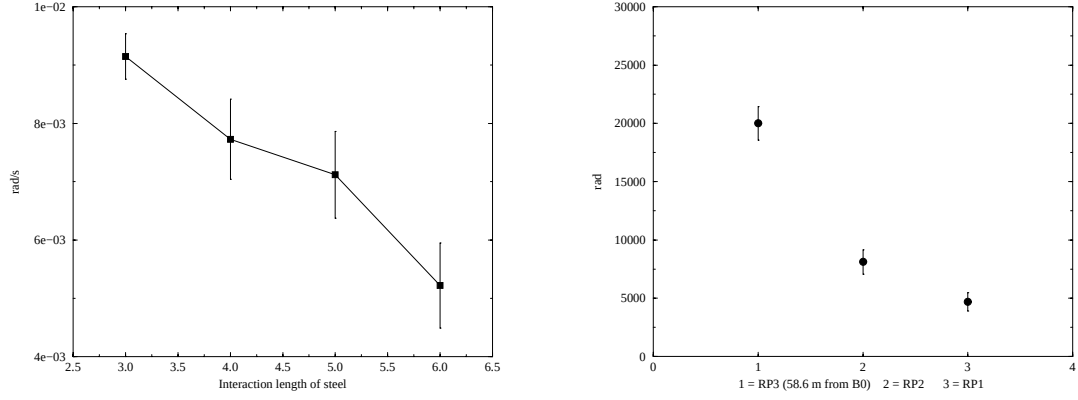
Figure 22: Absorbed dose in RP3 due to beam halo (left) and dose in RP1-RP3 due to AKP (right).
