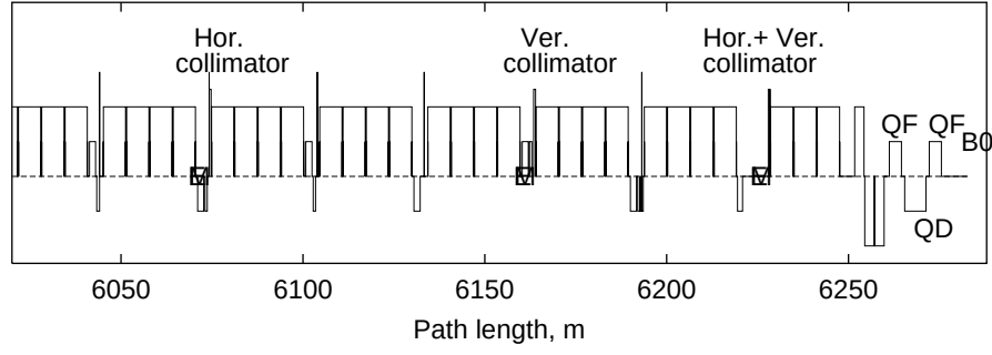
Figure 12: Location of shadow collimators upstream of B0.
