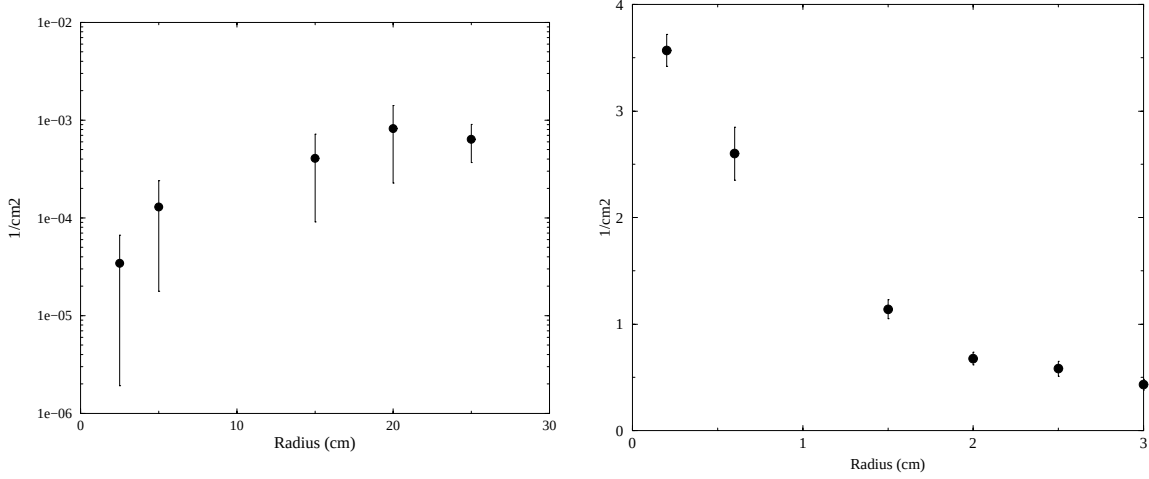
Figure 24: Charged particle albedo (left) and forward (right) flux in RP with a 0.5-m long steel rod.
