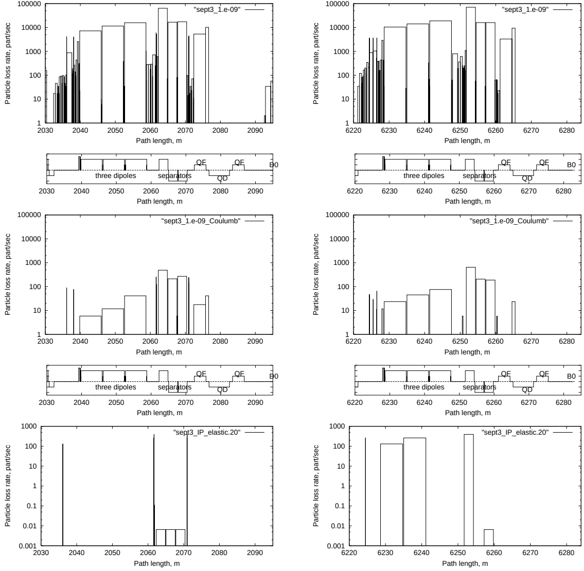
Figure 17: Beam loss distributions upstream of DØ and BØ for nuclear elastic beam-gas scattering at uniform gas pressure distribution 10^{-9} torr (top), large angle Coulomb scattering (middle), elastic p\bar{p} interactions at two IPs (bottom).
