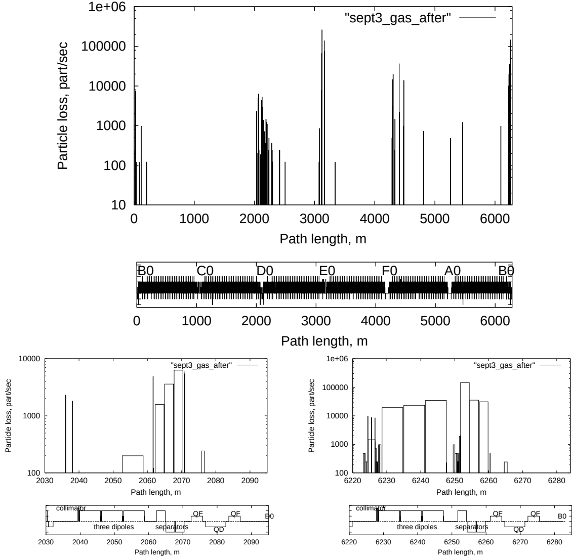
Figure 8: The “pressure bump” induced beam loss distributions in the entire ring (top) and in the DØ and BØ regions (bottom).
