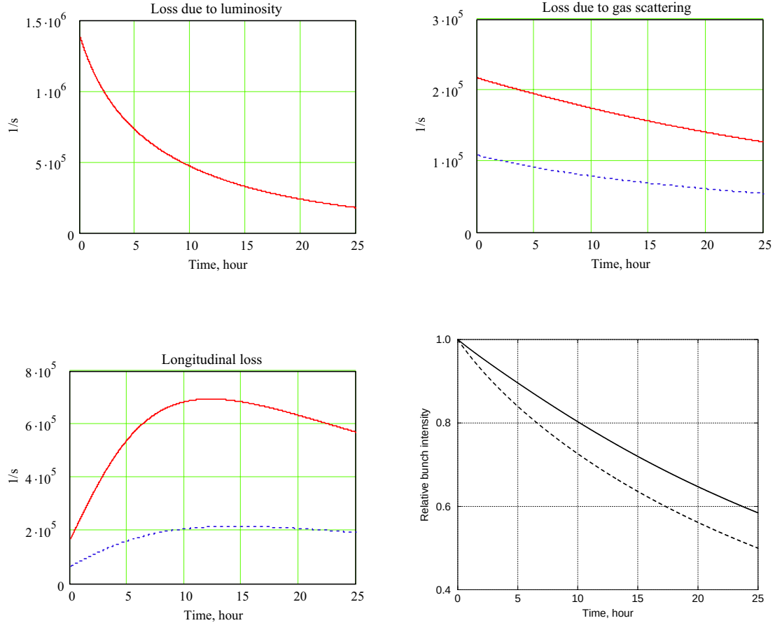
Figure 1: Evolution of proton (solid curves) and antiproton (dashed curves) bunch loss rates – collision (left top), longitudinal (left bottom) and beam-gas (right top) – and relative bunch intensity as evolved in a store (right bottom).
