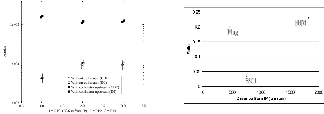
Figure 26: Charged particle flux at the DØ Roman Pots (left) and the main detector absorbed dose ratio with/without “double L-shaped” collimator for the elastic contribution as a function of a distance from the IP (right).
