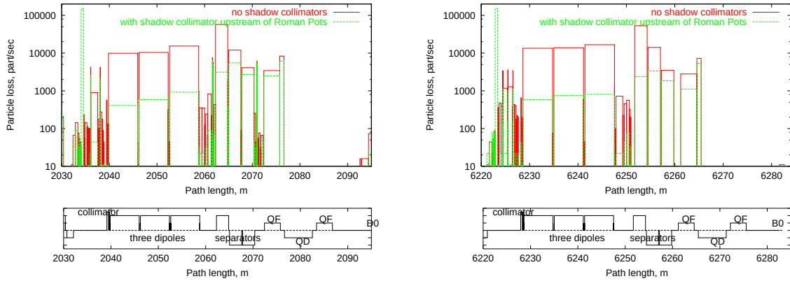
Figure 16: Beam-gas induced loss distributions in the DØ and BØ regions without (solid (red)) and with (dashed (green)) a shadow collimator at 13\sigma_x and 20\sigma_y at the non-IP ends of the RP stations at the measured residual gas pressure [18].
