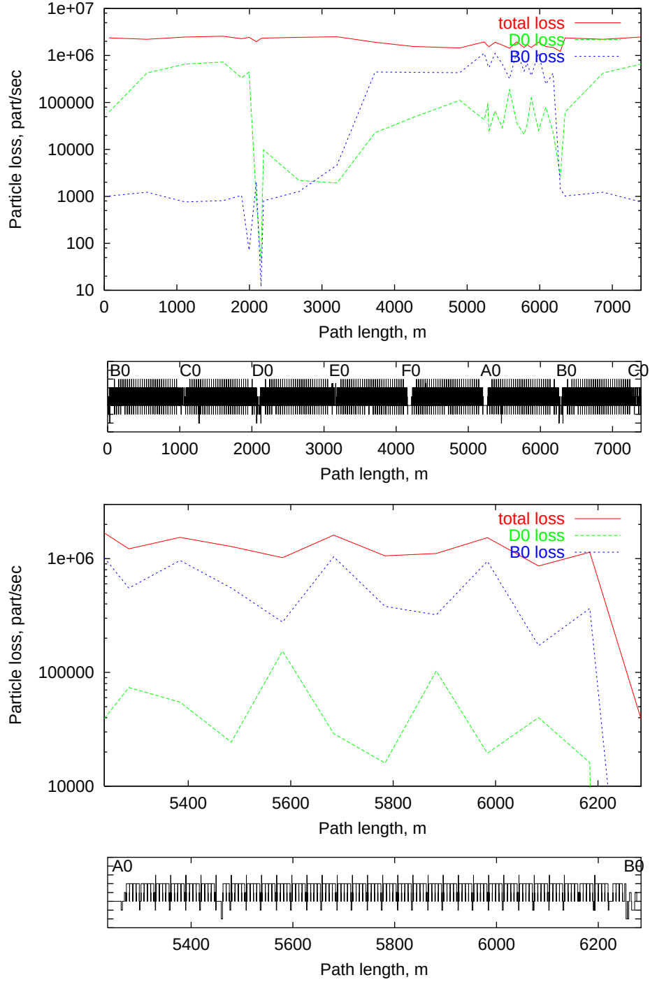
Figure 9: Beam loss at BØ and DØ as a function of a "pressure bump" location for the entire ring (top) and AØ -BØ region (bottom). Solid (red) line is total loss, dashed (green) is DØ loss, and dashed (blue) is BØ loss.
