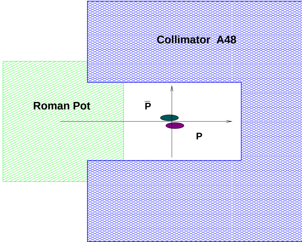
Figure 14: Shadow collimator at the IP end of the Roman Pots station.
