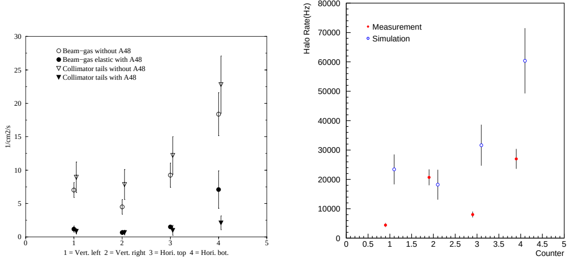
Figure 21: CDF BHM hit rate with and without A48 collimator (left) and corresponding comparison of MARS calculations with data [19] without the collimator (right).
