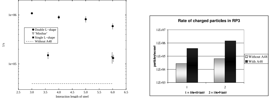
Figure 25: Rates of charged particles at RP3 as a function of the mask length for three shapes at the 10^{-9} torr average pressure (left) and their sensitivity to the gas pressure (right). The dashed line corresponds to a case without the mask.
