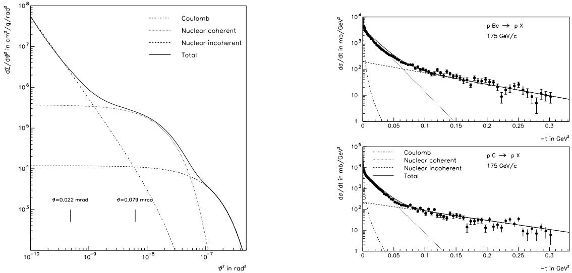
Figure 7: Components of the proton-nitrogen elastic differential cross section at 1 TeV (left) and comparison to experimental data [15] at 175 GeV/c (right).
