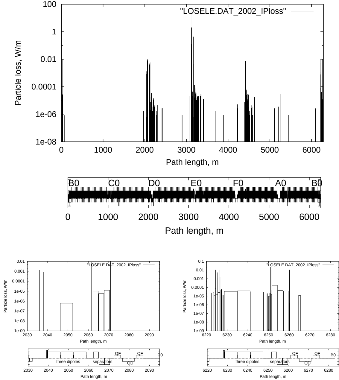
Figure 6: Beam loss distribution in the entire ring (top) and in the DØ and BØ regions (bottom).
