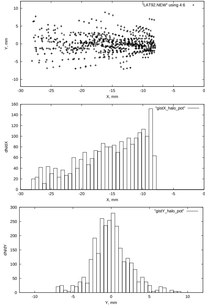
Figure 23: Halo hit distributions in the CDF Roman Pots without shadow collimators.
