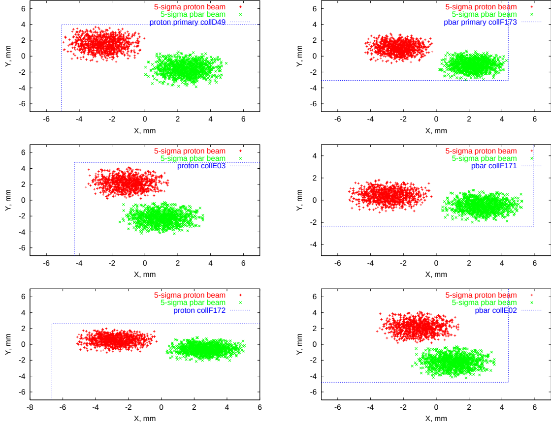
Figure 4: The 5- \sigma proton (red (black)) and antiproton (green (grey)) spatial distributions. Left : at proton primary collimator D49 (top) and secondary collimators E03 (middle) and F172 (bottom). Right : at antiproton primary collimator F173 (top) and secondary collimators F171 (middle) and E02 (bottom).
