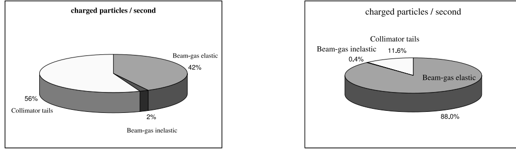
Figure 18: Contribution to BHM backgrounds at average pressure in Tevatron of 10^{-10} (left) and 10^{-9} (right) torr.
