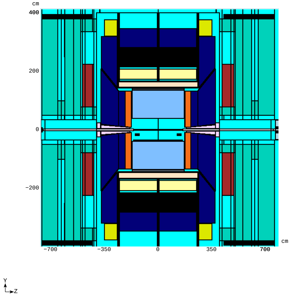
Figure 20: The CDF MARS model.
