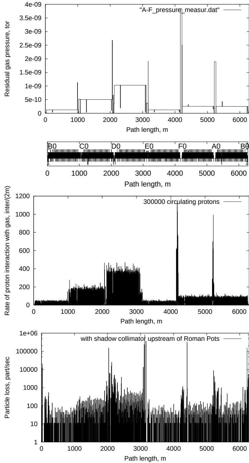
Figure 15: Measured [18] residual gas pressure (top), rate of proton interactions with gas (middle) and beam loss distribution in the Tevatron ring from nuclear elastic beam-gas scattering (bottom).
