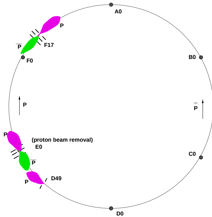
Figure 3: Tevatron Run-II beam collimation system.
