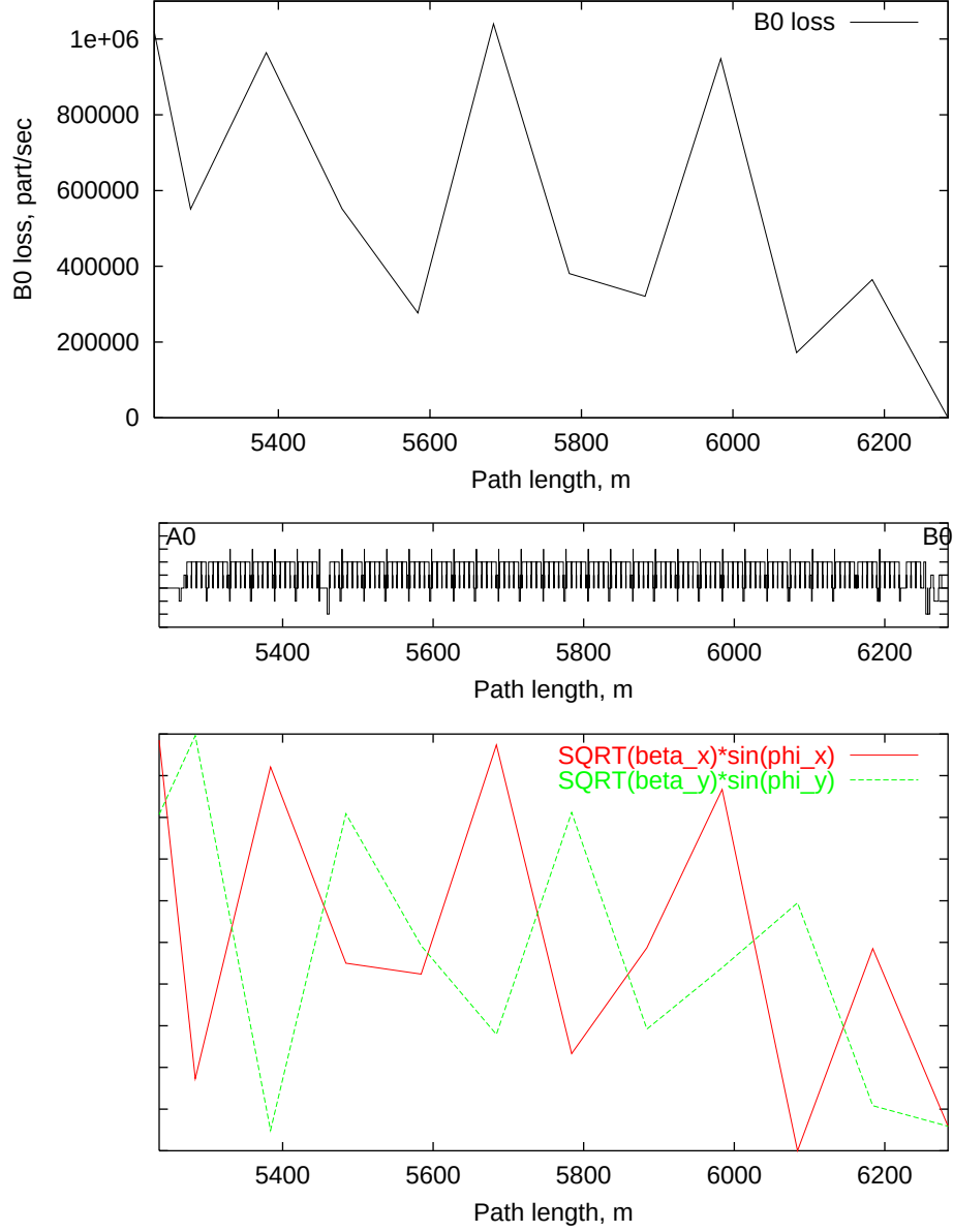
Figure 10: Beam loss at BØ as a function of a “pressure bump” location in the AØ-BØ region (top) and \|\beta^{1/2} \cdot \sin\phi\| at the locations of a “pressure bump” (bottom, with solid (red) line for horizontal and dashed (green) for vertical planes).
