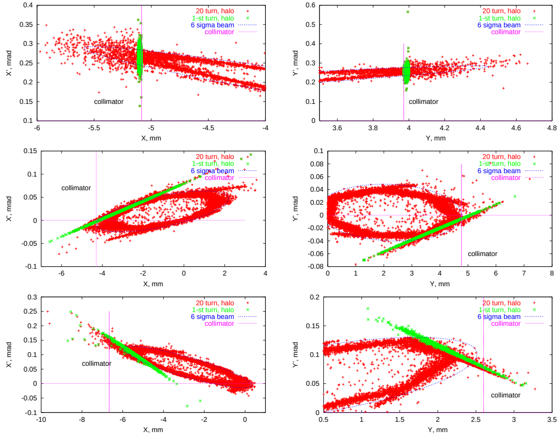
Figure 5: Horizontal (left) and vertical (right) phase space at primary proton collimator D49 (top), and secondary collimators E03 (middle) and F172 (bottom). Green (grey) – halo particles at the first turn after interaction with the primary collimator, red (black) – secondary halo, blue (black line) – 6\sigma envelope.
