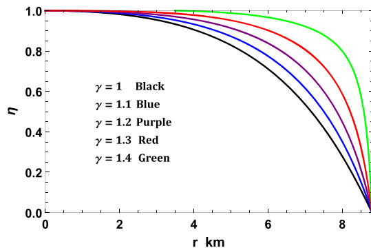
Fig. 7 The parameter \eta(r) is plotted with respect to the radial coordinate r for the compact star EXO 1785-248 corresponding to values of constants given in Table 2
