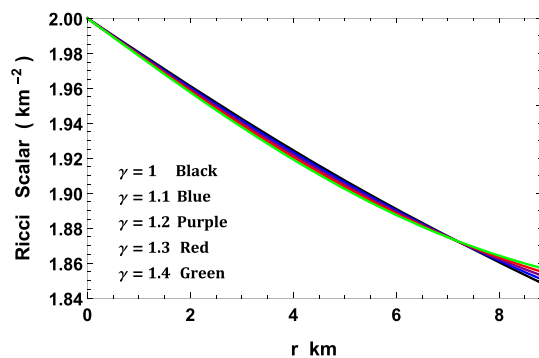
Fig. 8 The scalar curvature is plotted with respect to the radial coordinate r for the compact star EXO 1785-248 corresponding to values of constants given in Table 2
