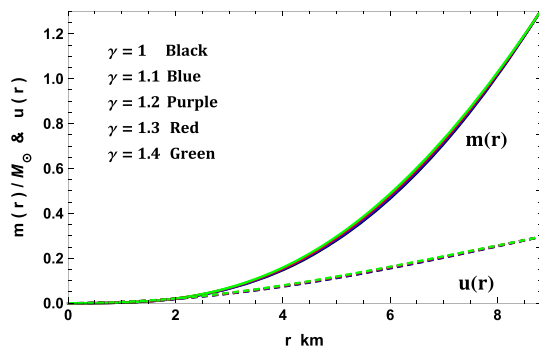
Fig. 6 The mass and compactness parameter are plotted with respect to the radial coordinate r for the compact star EXO 1785-248 corresponding to values of constants given in Table 2
