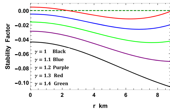
Fig. 12 The stability factor is plotted with respect to the radial coordinate r for the compact star EXO 1785-248 corresponding to values of constants given in Table 2
