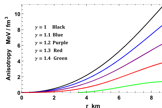
Fig. 5 The anisotropic factor is plotted with respect to the radial coordinate r for the compact star EXO 1785-248 corresponding to values of constants given in Table 2
