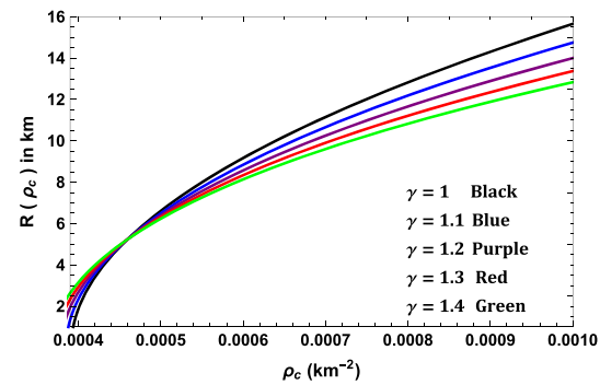
Fig. 15 The surface radius is plotted with respect to the central density \rho_c for the compact star EXO 1785-248 corresponding to values of constants given in Table 2
