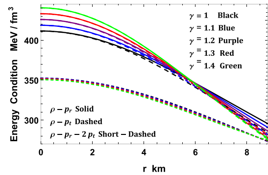
Fig. 9 The energy conditions are plotted with respect to the radial coordinate r for the compact star EXO 1785-248 corresponding to values of constants given in Table 2
