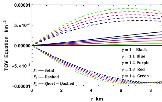
Fig. 10 The acting forces are plotted with respect to the radial coordinate r for the compact star EXO 1785-248 corresponding to values of constants given in Table 2
