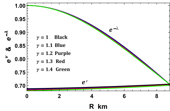
Fig. 1 e^{v(r)} and e^{-\lambda(r)} are plotted with respect to the radial coordinate r for the compact star EXO 1785-248 corresponding to values of constants given in Table 2
