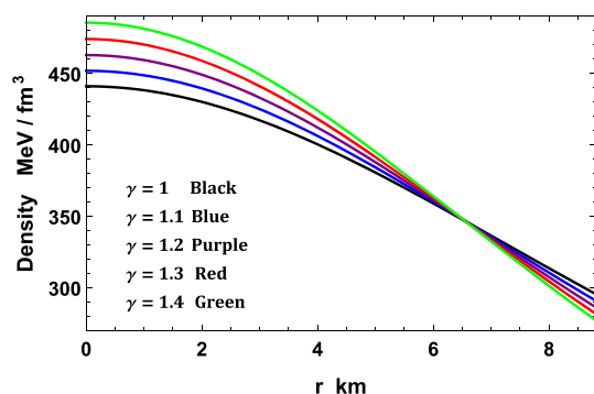
Fig. 2 The energy density is plotted with respect to the radial coordinate r for the compact star EXO 1785-248 corresponding to values of constants given in Table 2
