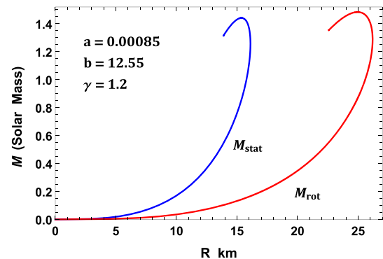
Fig. 18 The static mass and rotating mass are plotted with respect to the surface radius R for the compact star EXO 1785-248 corresponding to b = 12.55 km and B_g = 60 MeV/fm 3
