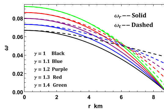
Fig. 4 The equation of state parameters are plotted with respect to the radial coordinate r for the compact star EXO 1785-248 corresponding to values of constants given in Table 2
