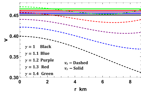
Fig. 11 The sound speeds are plotted with respect to the radial coordinate r for the compact star EXO 1785-248 corresponding to values of constants given in Table 2
