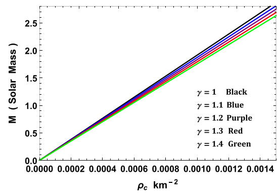
Fig. 14 The mass function is plotted with respect to the central density \rho_c for the compact star EXO 1785-248 corresponding to values of constants given in Table 2
