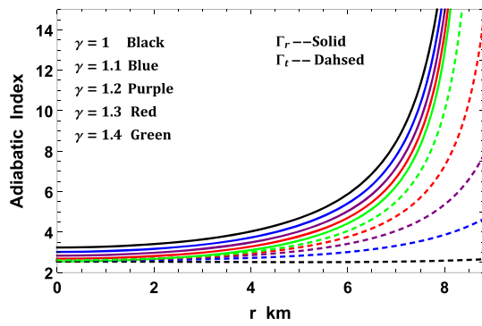
Fig. 13 The adiabatic indexes are plotted with respect to the radial coordinate r for the compact star EXO 1785-248 corresponding to values of constants given in Table 2
