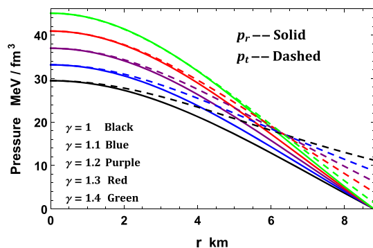
Fig. 3 The radial and transverse pressures are plotted with respect to the radial coordinate r for the compact star EXO 1785-248 corresponding to values of constants given in Table 2
