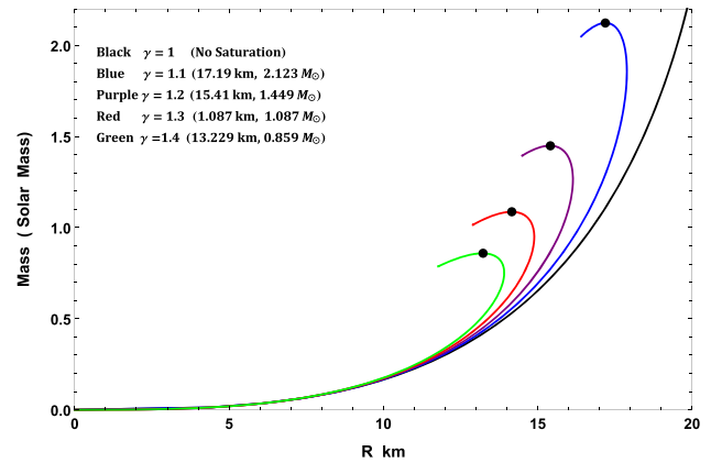
Fig. 17 The mass is potted with respect to the surface radius R for the compact star EXO 1785-248 corresponding to values of constants given in Table 2
