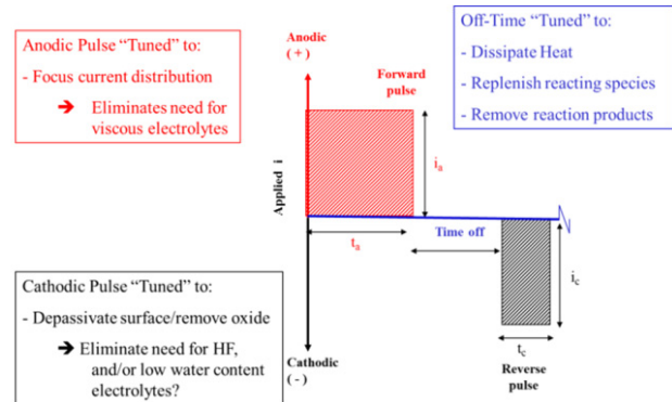
Figure 1: Illustration of the principle of Bipolar EP.
