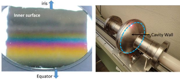
Figure 4: Optical inspection image of cavity wall showing discoloration generated during the salt EP.
