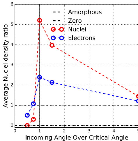
Fig. 1. Geant4 simulation of the modification of the nuclear interaction rate as a function of the particle incoming angle interacting with a Si (220) crystal. The particles impinge at 0.48 Å from the Si (220) planes.
