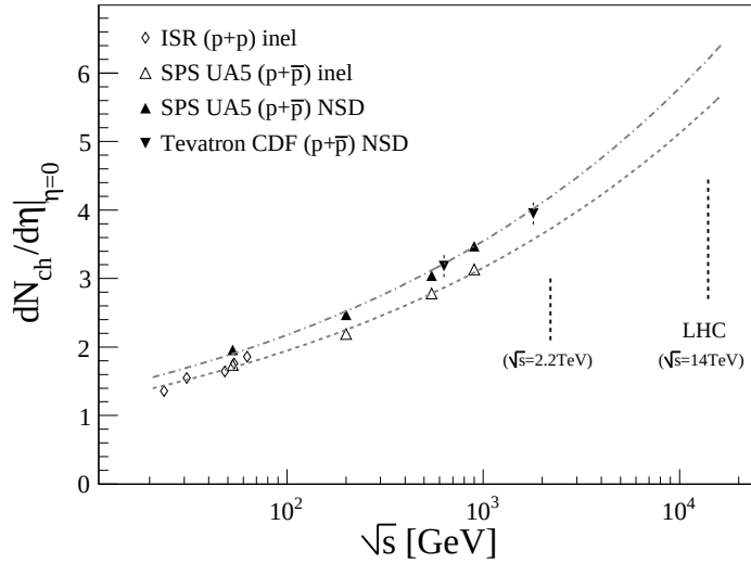
Fig. 1. Center of mass dependence of the pseudorapidity density at midrapidity. Data points are from Ref. [5–7]. The dashed lines show the \ln^2(s) extrapolation to higher energies. The vertical bars indicate the possible LHC energy \sqrt{s} = 2.2 TeV and the maximum energy \sqrt{s} = 14 TeV
