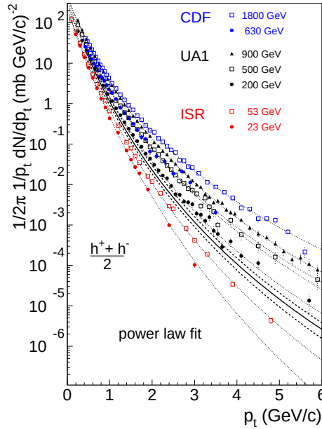
Fig. 2. Midrapidity transverse momentum spectra of unidentified hadrons at different energies. The plot is from Ref. [14].
