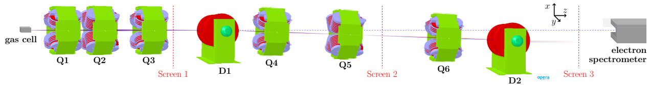
Figure 1: Sketch of the setup with six quadrupoles and two dipoles. The beam profile was measured with scintillating screen 1 to 3, the energy distribution with the electron spectrometer.
