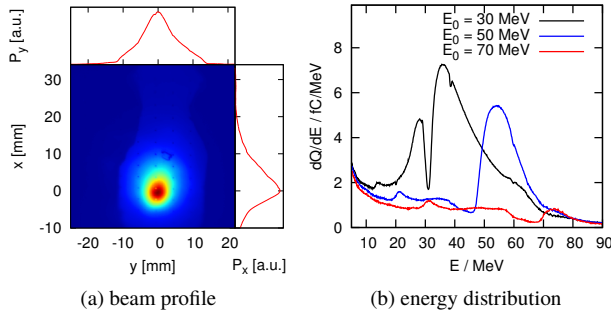
Figure 2: (a) Beam profile of the unfocused beam measured on screen 1 with the projection P on both axes. (b) Spectra of the electrons for three different configurations of Q1 to Q3 focusing a certain energy range to the spectrometer.
