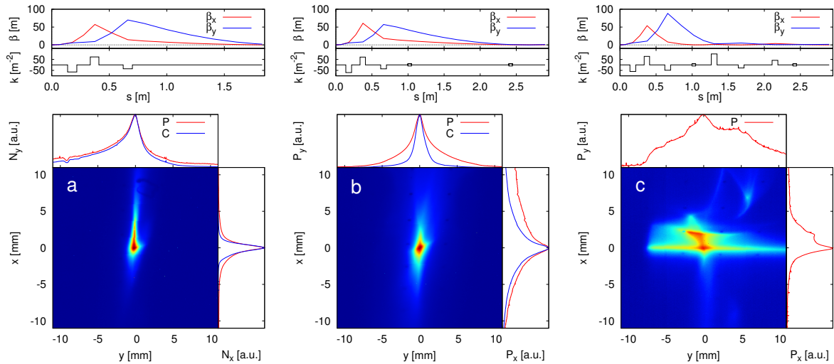
Figure 3: Measured beam profiles with a projection P on and a cut C along each axis. The quadrupole strength k the position of the dipoles and the betafuncions are depicted for each setup with \beta_0 = 0.005 m and \alpha_0 = 0 . (a) Focus of 60 MeV on the second screen; (b) focus of 40 MeV on the third screen with deflection by the dipoles; (c) parameters necessary for the operation of the undulator at 40 MeV.
