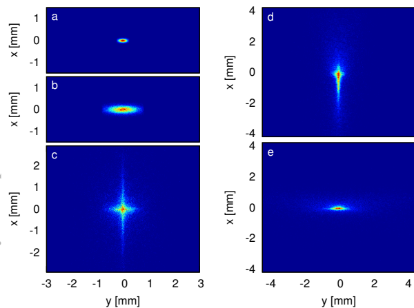
Figure 4: left: Simulated beam profiles at the position of screen 2 with (a) \sigma_{x',y'} = 1 mrad, (b) the measured source divergence and (c) additionally an energy spread of \sigma_E = 5\% ; right: simulated beam profiles on screen 3 with the measured divergence and 5% energy spread with (d) setup of Fig. 3b and (e) setup of Fig. 3c.
