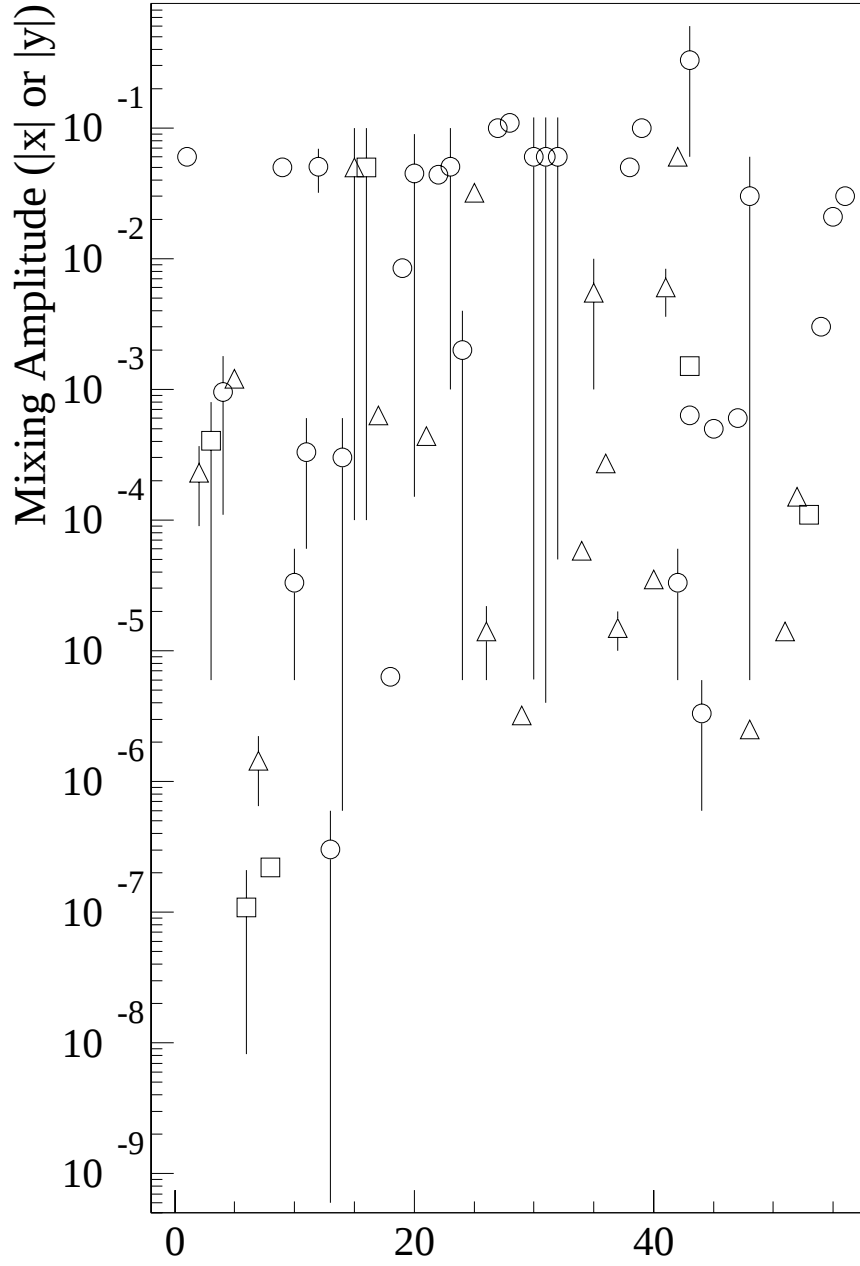
Figure 1.5: A collection of 56 theoretical predictions for D^0 - \overline{D}^0 mixing based on the compilation of Harry Nelson [21]. The triangles are SM based predictions of x , the squares are SM predictions of y and the circles are non-SM predictions of x .
