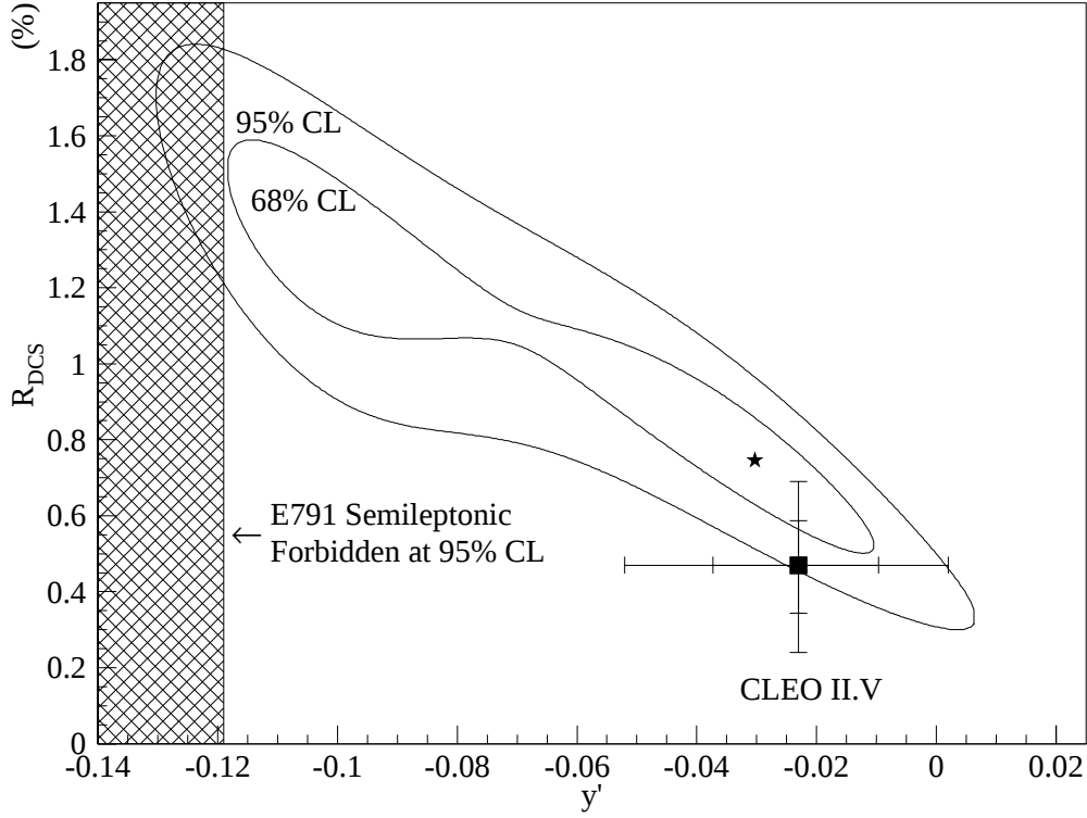
Figure 8.2: A comparison of the R_{DCS} and y' CL regions to the CLEO II.V and E791 results.
