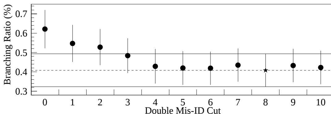
Figure 6.11: R_{\text{WS}} versus the strength of the double mis-ID cut. Note that the branching ratio is constant above a cut of four, well below the value of eight (indicated by a star) used in the analysis.
