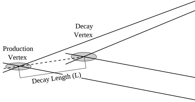
Figure 4.1: Schematic of the charm production and decay vertices. The ellipses represent the vertex resolution and the decay length is a measure of the production and decay vertex separation.
