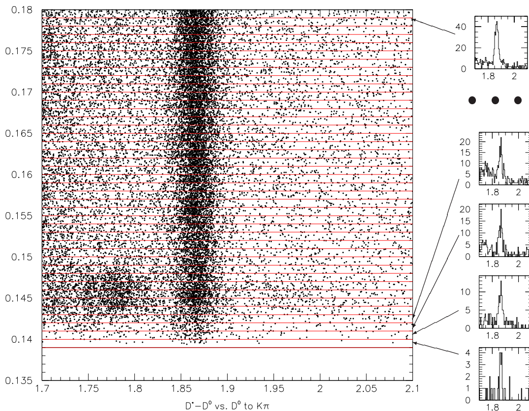
Figure 6.6: On the left is the WS D^* - D mass difference plotted against the K\pi mass. In the new method, this plot is sliced into 1 \text{ MeV}/c^2 bins in mass difference. The K\pi mass is plotted and fit in each bin. The resulting fitted D^0 yields are plotted at the appropriate mass difference (see Figure 6.9).
