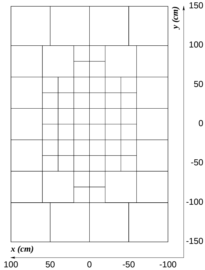
Figure 3.7: Schematic of the Hadron Calorimeter showing the configuration of the tiles.
