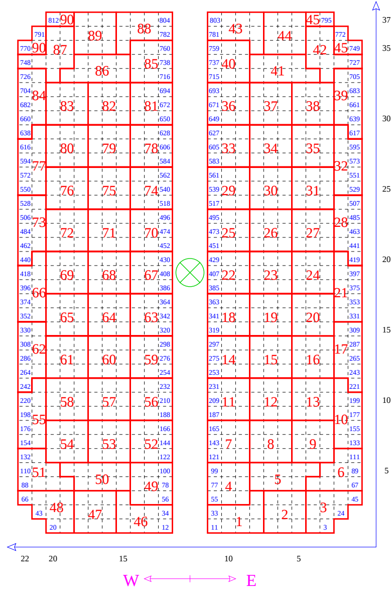
Figure 3.6: Schematic of the Inner Electromagnetic Calorimeter showing block layout (dashed lines) and trigger summer groupings (heavy lines).
