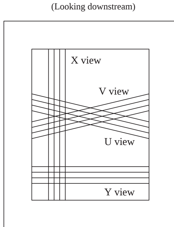
Figure 3.3: Signal wire layout of the proportional wire chambers.
