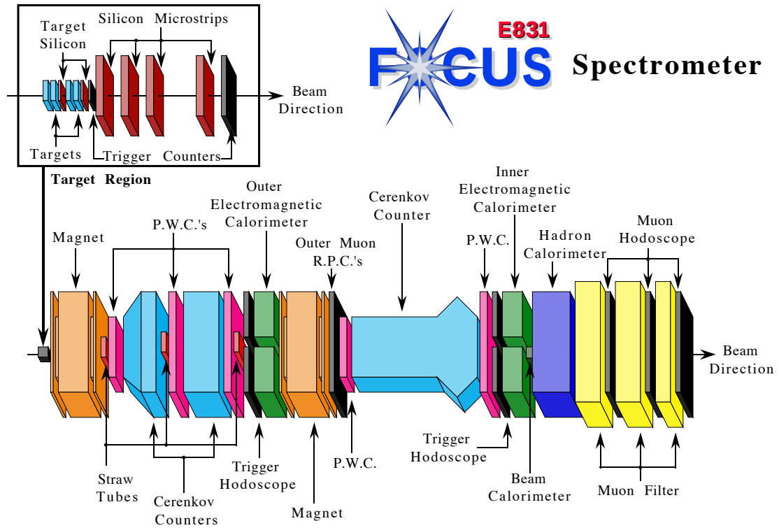
Figure 3.1: Schematic of the FOCUS Spectrometer.
