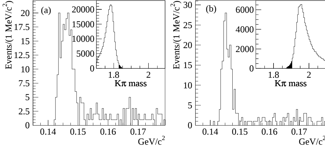
Figure 6.4: D^0 Monte Carlo events generated as decays to a) KK and b) \pi\pi , reconstructed and selected as K\pi . The inset plots show K\pi mass distributions and the large plots show the mass difference distribution for events in the D^0 mass window (shaded area of inset plot).
