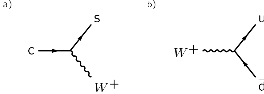
Figure 1.1: The Cabibbo favored weak vertices relevant for charm quark decays. a) The charm decay vertex and b) the W decay vertex.
