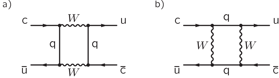
Figure 1.4: The box diagrams that give the lowest order contribution to D^0 - \bar{D}^0 mixing.
