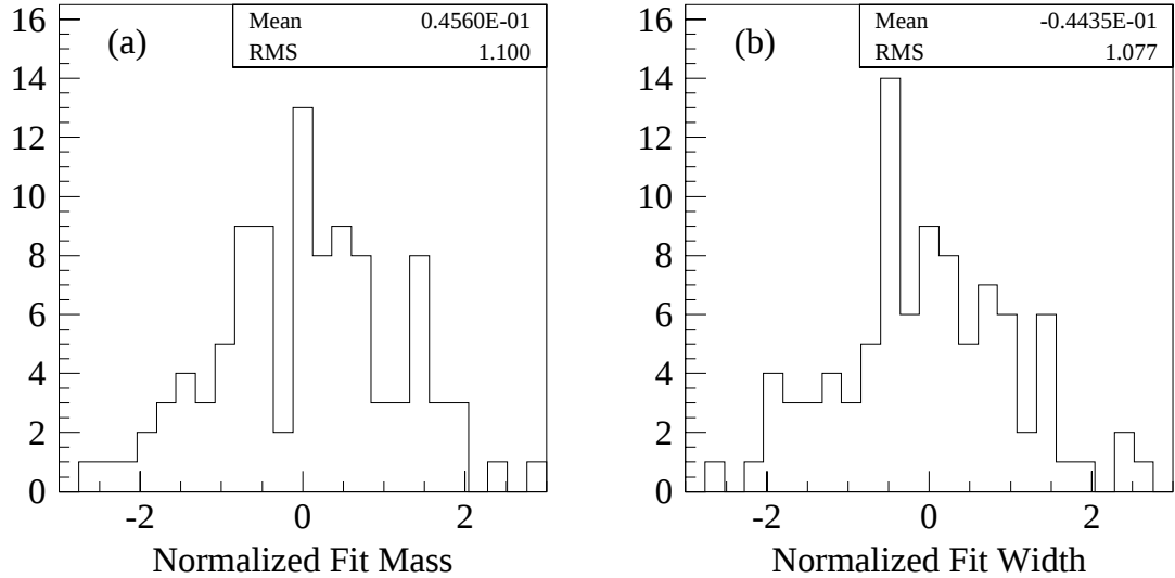
Figure 6.7: Distributions of the D^0 a) mass and b) width fit parameters normalized to errors. These plots show that the Gaussian fit to the D^0 signal is well behaved across the 80 fits.
