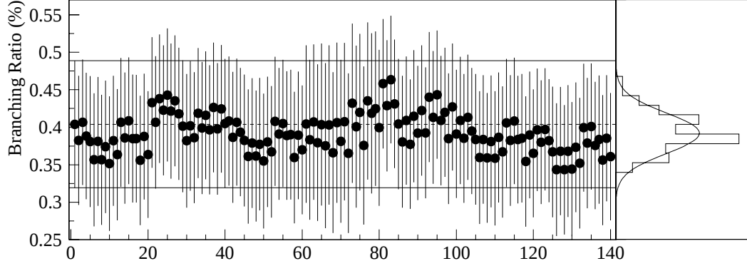
Figure 6.12: The spread of R_{\text{WS}} measurements. The systematic error is taken to be the statistical variance of the points in the distribution ( \sigma_{\text{sys}} = 0.025\% ). The horizontal lines are the value of R_{\text{WS}} and its error for the baseline measurement.
