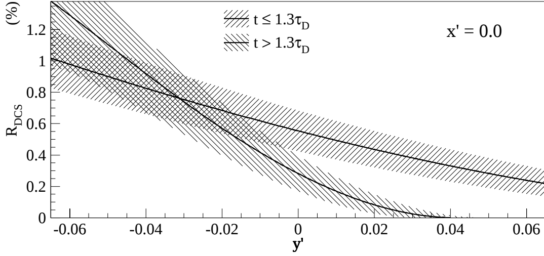
Figure 7.3: The intersection of R_{\text{DCS}} curves for high and low lifetime bins split at 1.3\tau_{D^0} .
