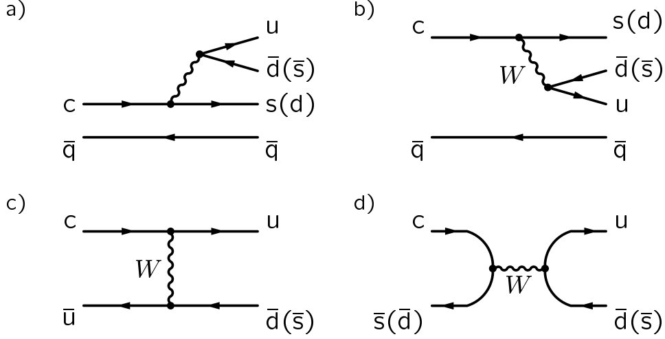
Figure 1.3: The lowest order Feynman diagrams for charm meson decay processes: a) external W boson emission, b) internal W emission, c) W boson exchange, and d) quark annihilation. Quarks associated with the Cabibbo suppressed processes are shown in parentheses.
