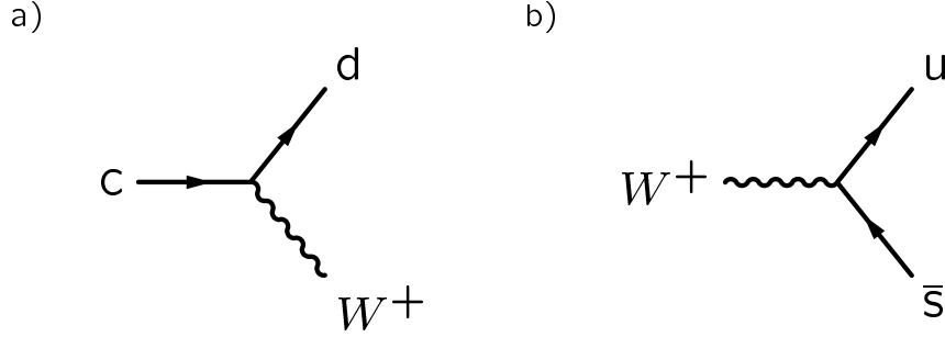
Figure 1.2: The Cabibbo suppressed weak vertices relevant for charm quark decays. a) The charm decay vertex and b) the W decay vertex.
