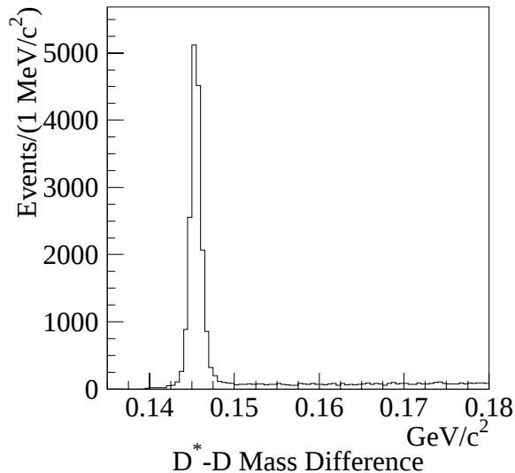
Figure 6.1: The D^* - D mass difference for RS tagged D^0 \rightarrow K^-\pi^+ events.
