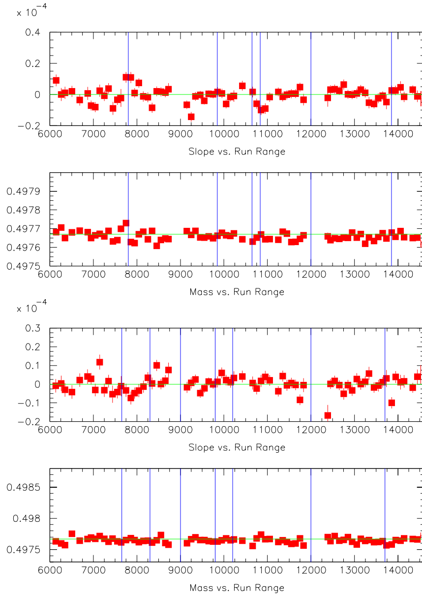
Figure 5.3: Corrected mass scale and asymmetry plots (compare to Figure 5.2).
