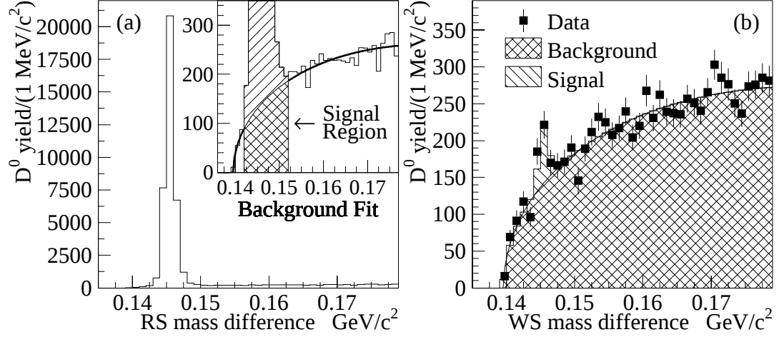
Figure 6.9: The a) right sign and b) wrong sign mass difference plots generated by fitting D^0 peak in 1 \text{ MeV}/c^2 bins of D^*-D mass difference. The inset to (a) is a close up of the RS background. The RS background fit is shown as a solid curve.
