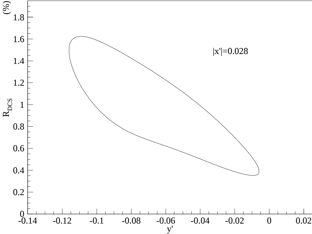
Figure 7.6: The confidence level region for y' and R_{\text{DCS}} with |x'| = 0.028 and the lifetime split at 1.3 \tau_{D^0} .
