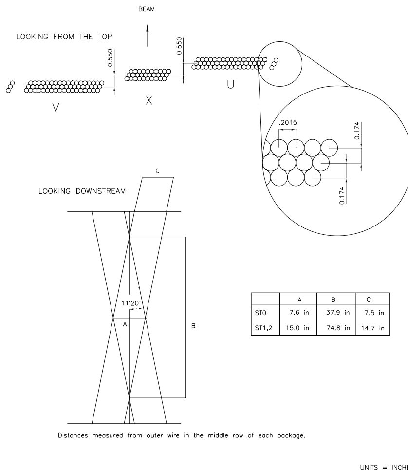
Figure 3.4: Schematic of the straw tube detectors showing basic layout and dimensions.
