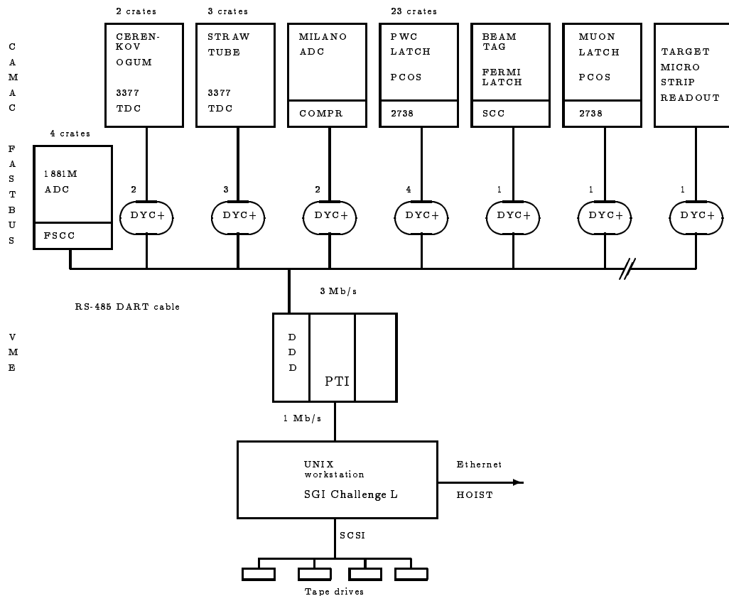
Figure 3.8: Overview of the DAQ layout.
