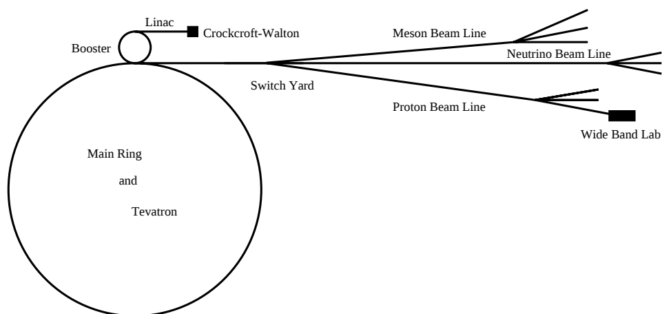
Figure 2.1: Schematic of the Fermilab accelerator complex and fixed target beam lines.
