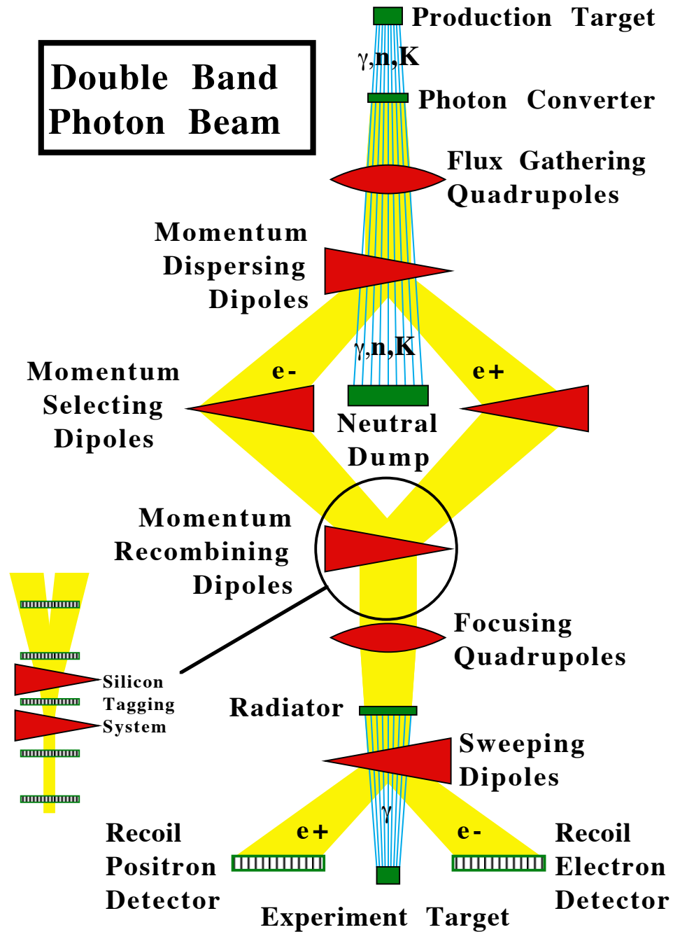
Figure 2.2: Schematic of Wideband photon beam line.
