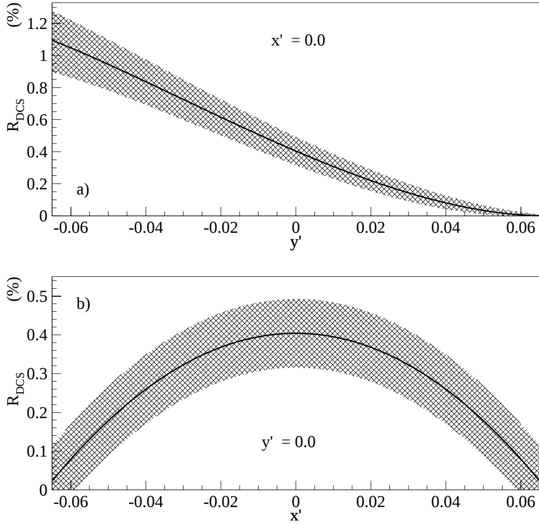
Figure 7.1: R_{\text{DCS}} plotted as a function of a) y' with x' = 0 and b) x' with y' = 0 .
