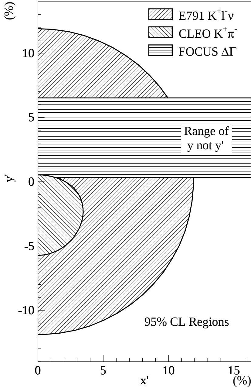
Figure 1.8: Comparison of the best experimental limits on x' and y' from the three methods discussed in Section 1.5. The FOCUS \Delta\Gamma band is only directly comparable to the other experiments in the case of \delta = 0 .
