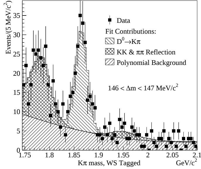
Figure 6.8: A typical fit of the K\pi mass from the WS mass difference signal region, where the reflections are most prominent.
