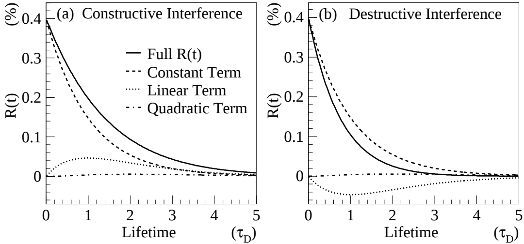
Figure 1.6: Time evolution of the decay D^0 \rightarrow K^+\pi^- with a) constructive interference and b) destructive interference. A value of y' = 2\% is used in this illustration.
