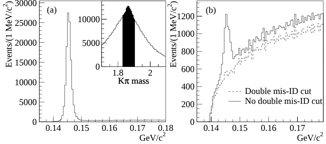
Figure 6.3: a) The K\pi mass distribution (inset) and mass difference distribution for events in the D^0 signal region (shaded area of inset) for Monte Carlo events generated and selected as D^0 \rightarrow K^-\pi^+ , but reconstructed as K^+\pi^- . b) The WS distribution from the same Monte Carlo events (reconstructed as selected) with and without the double mis-ID cut. No WS decays were generated.
