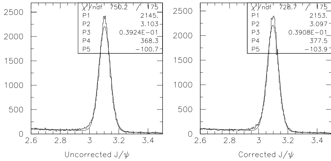
Figure 5.4: J/\psi mass (parameter P2) before and after the correction.
