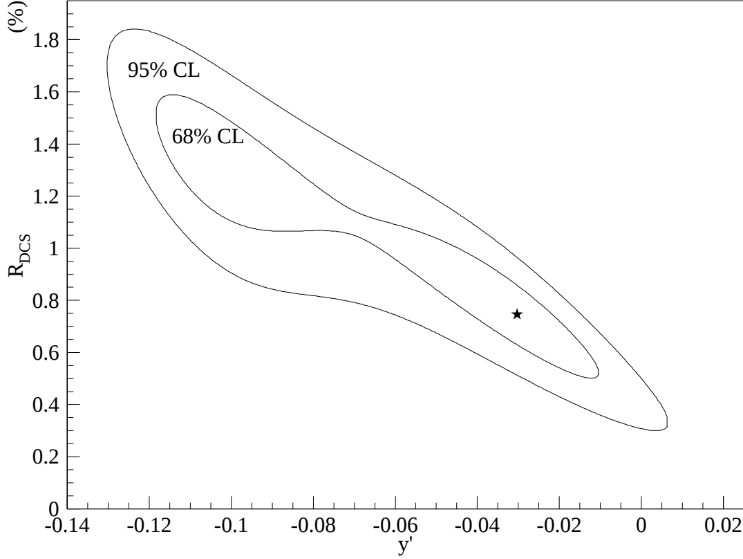
Figure 7.4: The 95% and 68% (or 1\sigma ) confidence level regions for y' and R_{\text{DCS}} from a lifetime split at 1.3\tau_{D^0} .
