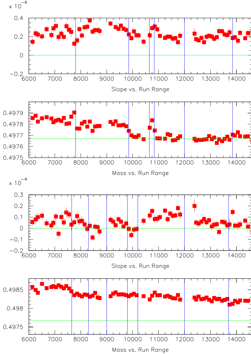
Figure 5.2: Run dependent mass scale and momentum asymmetry slope for M1 (top) and M2 (bottom). The vertical lines delineate the run periods where different correction constants were applied and the horizontal lines are the expected mass or slope.
