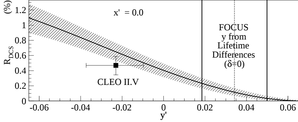
Figure 8.1: R_{\text{DCS}} contour compared to the CLEO II.V and FOCUS mixing results. A direct comparison to the FOCUS result requires \delta = 0 .
