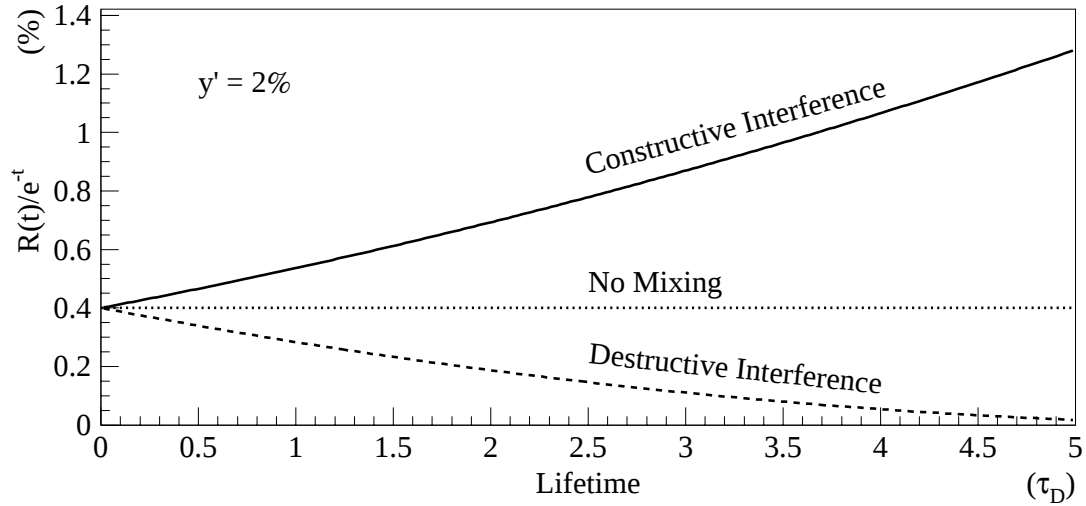
Figure 1.7: The lifetime dependence of D^0 \rightarrow K^+ \pi^- rate with y' = 2\% for the cases of constructive interference, destructive interference and no mixing.
