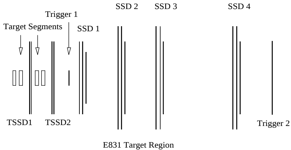
Figure 3.2: Layout of the FOCUS target region, showing the four target segments, the four target silicon planes (TSSD), the 12 E687 SSD planes and the trigger elements TR1 and TR2 (described in Section 3.11.1).
