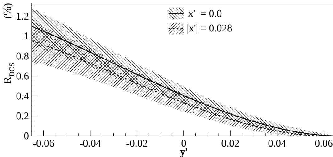
Figure 7.2: R_{\text{DCS}} plotted as a function of y' . The bands are given for x' = 0.0 and |x'| = 0.028 , which cover the 95% CL from CLEO II.V.
