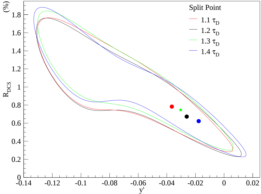
Figure 7.5: The confidence level regions and crossing points for y' and R_{\text{DCS}} from several splits in the range of 1.1 to 1.4\tau_{D^0} .
