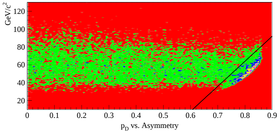
Figure 6.2: The D^0 momentum vs. K\pi asymmetry. Events below and to the right of the solid line are rejected by the asymmetry cut.
