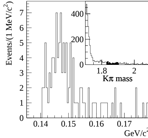
Figure 6.5: D^0 Monte Carlo events generated for all decay mode except K\pi , KK and \pi\pi , reconstructed and selected as K\pi . The inset shows the K\pi mass distribution. The only structure is the reflection from partially reconstructed K\pi\pi^0 below 1.75 \text{ GeV}/c^2 . The large plot shows the mass difference distribution for events in the D^0 mass window.
