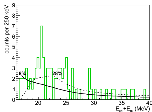
Figure 2. ^{16}\text{C} invariant mass spectrum ( E_{\text{rel}} + E_{\text{thr}} ) for the ^{10}\text{Be} + ^6\text{He} break-up channel. The dashed and solid lines represent, respectively, the simulated detection efficiency for inelastic scattering on proton, peaking at 28%, or carbon, peaking at 8%.
