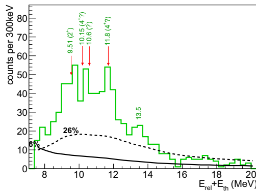
Figure 1. ^{10}\text{Be} invariant mass spectrum ( E_{\text{rel}} + E_{\text{thr}} ) for the ^4\text{He} + ^6\text{He} break-up channel. The dashed and solid lines represent, respectively, the simulated detection efficiency for inelastic scattering on proton, peaking at 26%, or carbon, peaking at 6%. Arrows indicate the position of known states in the literature.
