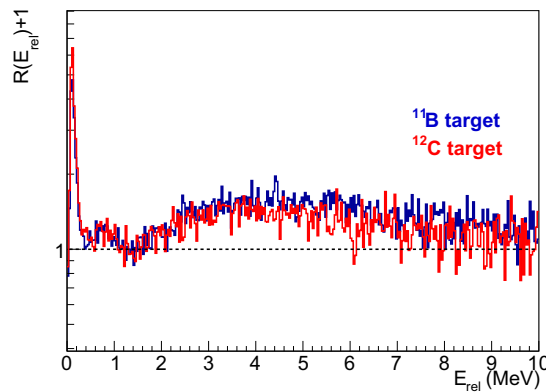
Figure 3. \alpha - \alpha correlation function ( R(E_{\text{rel}} + 1) ) in logarithmic scale for two different nuclear collisions ^{16}\text{O}+^{11}\text{B} (blue line) and ^{16}\text{O}+^{12}\text{C} (red line) at 55 MeV/u. The dashed line represents the line R(E_{\text{rel}}) = 1 .
