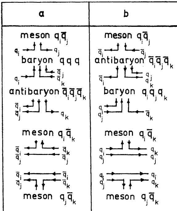
Fig. 6. All possible vertices for meson, baryon and antibaryon production in our chain decay model. a) in the jet of the primary quark q_0 ; b) in the jet of the primary antiquark \bar{q}_0 . i, j, k are the flavour indices
