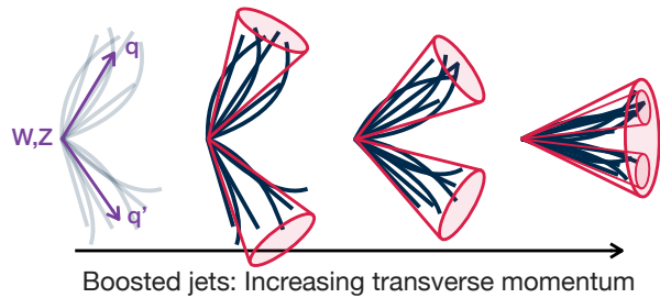
Figure 1: Illustration of the effect of increased transverse momentum on the angular separation of a two-pronged hadronic system (lines), e.g. one originating from the hadronic decay of a vector boson W/Z into two quarks, qq' . At low W/Z p_{\perp} , the quarks can be resolved by reconstructing the vector boson with a small-radius jet algorithm (small cones). At high p_{\perp} the quarks become too collimated to be resolved and are reconstructed as a single, large-radius jet (large cone).
