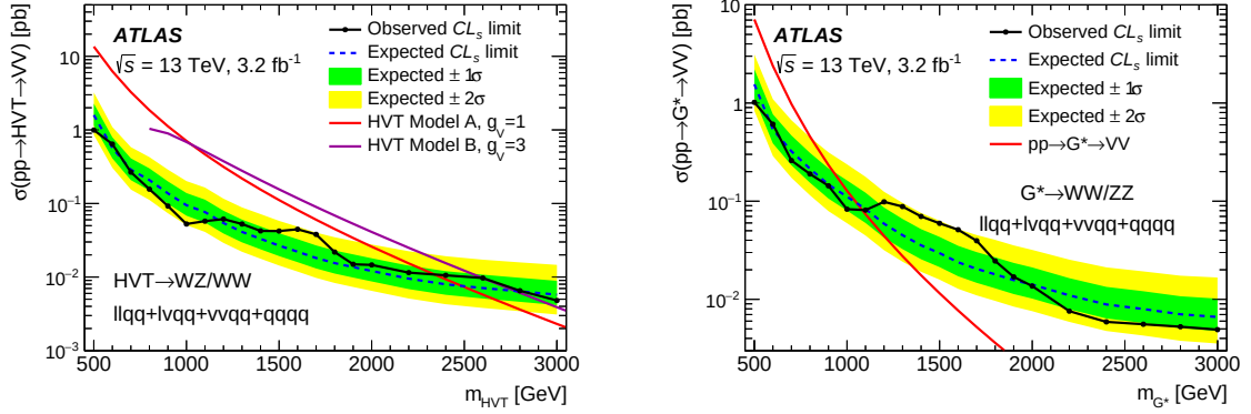
(a) HVT decays W' \rightarrow WZ and Z' \rightarrow WW , with predicted cross section times branching fraction overlaid.
