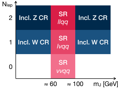
(a) Signal (SR) and inclusive vector boson control (CR) regions for the semi-leptonic channels, partitioned by leading jet mass m_J and number of signal leptons N_{\text{lep}} .
