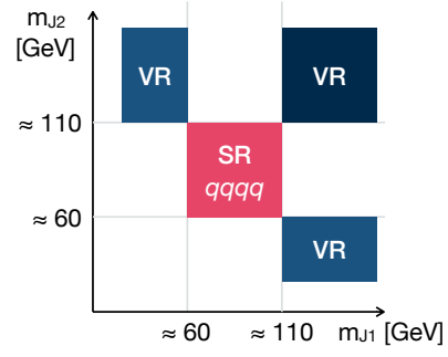
(b) Signal (SR) and non-resonant validation (VR) regions for the fully hadronic channel, partitioned by leading- and subleading jet mass m_{J1} and m_{J2} .
