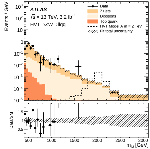
(b) Invariant mass of two signal leptons and large radius jet J in the \ell\ell J channel.
