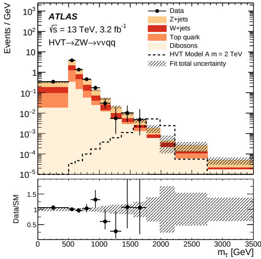
(a) Transverse mass of E_{\perp}^{\text{miss}} and large radius jet J in the vvJ channel.
