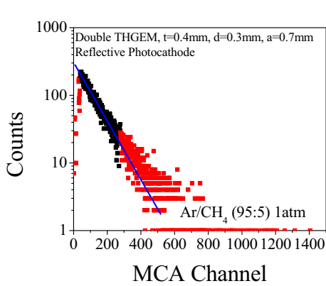
Figure 4.27: Single photoelectron pulse height; the result of the exponential best fit is superimposed. The red data points are excluded from the fitting procedure. The detector gain is set to \sim 10^4 [92].
