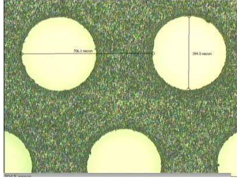
Figure 7.5: Picture of THGEM #2: d=0.4 mm, p=0.7 t=0.6 mm, rim=0.
