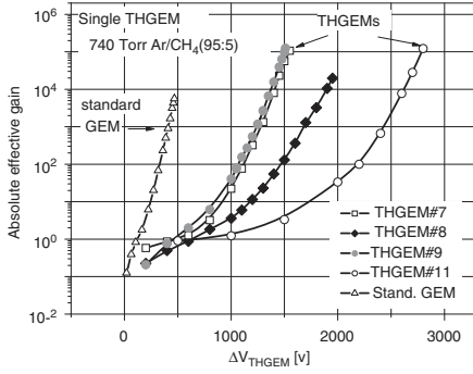
Figure 4.10: Gain measurement versus \Delta V_{THGEM} for detectors based on THGEMs with different geometries (Table 4.1); gas mixture: Ar/CH 4 (95:5). UV photons are detected [80].
