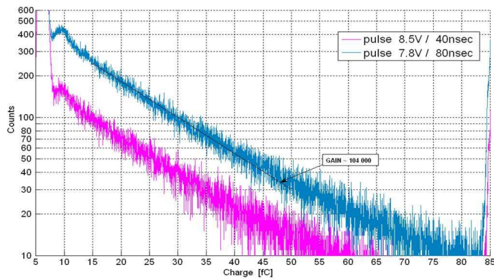
Figure 5.13: Amplitude spectra collected in single photoelectron mode at two two different light intensities.
