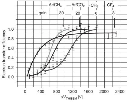
Figure 4.17: Electron Transfer Efficiency versus \Delta V_{THGEM} in a Ref photocathode detector, in several gases for a THGEM with geometrical parameters: d=0.3 mm, p=0.7 mm, t=0.4 mm and rim=0.1 mm [80].
