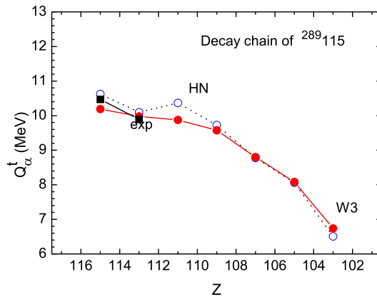
Fig. 1. (Color on-line) The \alpha -transition energies Q_\alpha^t calculated within the models HN and WS3+, as compared with the experimental values.
