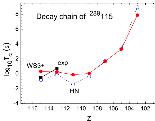
Fig. 2. (Color on-line) Logarithm of the \alpha -transition half-lives T_\alpha (given in seconds) calculated with the use of HN and WS3+ masses, as compared with the measured values.
