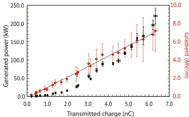
Figure 4: Power in the downstream coupling waveguide of the PBG structure as a function of the transmitted charge. The gradient in the structure computed from the measured power is also shown.
