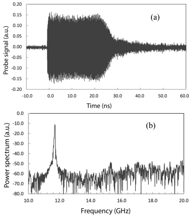
Figure 3: The rf signal in the downstream coupling waveguide of the PBG structure: (a) time-domain; (b) Fourier transform.
