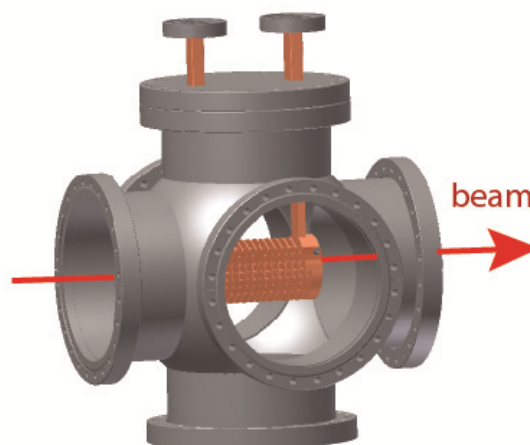
Figure 1: A 16-cell traveling-wave PBG accelerator structure with two waveguide couplers installed in a vacuum chamber for the wakefield tests.
