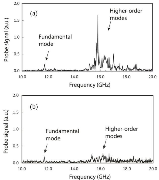
Figure 5: The rf spectrum of the signal picked up by a loop antenna at the periphery of the PBG structure: (a) the structure wrapped in foil; (b) the structure with 6 SiC absorbers.
