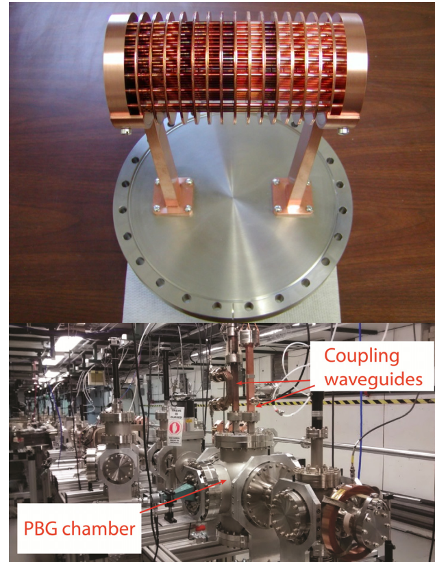
Figure 2: Photographs of the electroformed 11.7 GHz PBG cells installed on the 10 inch flange of a SS chamber and the beamline at Argonne Wakefield Accelerator with the PBG experimental chamber.
