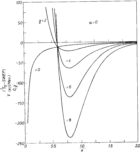
Fig. 2. An ^1S_0 -state \lambda\Phi^6 SWEP (Eq. (4.4)). \alpha = 0 for all the curves. \gamma = 0 is the usual O. P. E. Yukawa potential. The curves show the effect of the \lambda_2 -term when \lambda_1 = 0 . Notice the large values of \gamma used compared to those of Fig. 1
