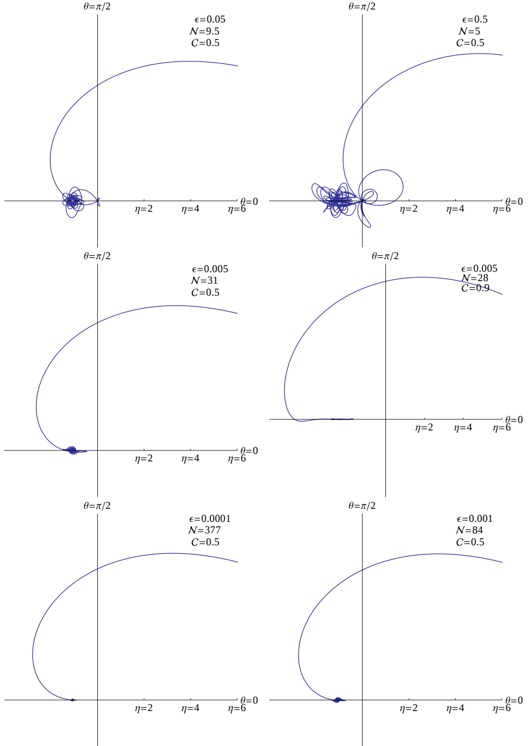
Figure 4.2: Some sample inflationary trajectories with a flux parameter of g_s M = 100 , inflaton mass m_0 = 20 , and a saturated Planck mass from \eta_{UV} = 10 . The values of \epsilon and \mathcal{C} = c_2 \epsilon^{-4/3} , are indicated.
