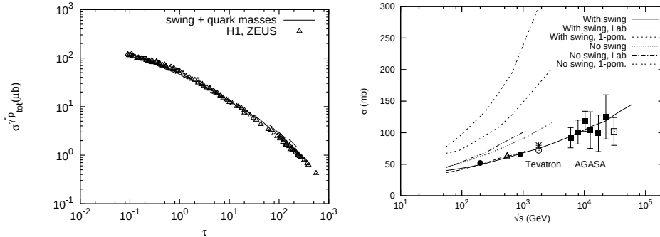
Fig. 8. Results from the dipole cascade model in Refs. [36, 37]. Left: The \gamma p total cross-section plotted as a function of the scaling variable \tau = Q^2/Q_s^2 , where Q_s^2 = Q_0^2(x_0/x)^\lambda with Q_0 = 1\text{GeV} , x_0 = 3 \times 10^{-4} , \lambda = 0.29 . Right: The total pp scattering cross-section. Results are presented for evolution with and without the dipole swing mechanism. The one pomeron result and the result obtained in a frame where one of the protons is almost at rest are also shown.
