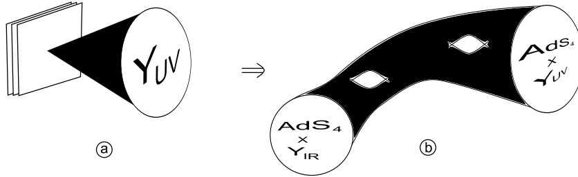
Figure 4.2: (a) A stack of N M2 branes transverse to the CY cone singularity \mathcal{C}(Y_{\text{UV}}) ; (b) the supergravity geometry describing an RG flow dual to a diagonal Higgsing.
