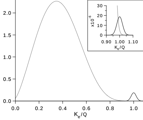
Figure 1: 2\nu\text{DBD} and 0\nu\text{DBD} two electrons sum energy spectra. 2\nu\text{DBD} is a continuum between 0 and Q_{\beta\beta} , while 0\nu\text{DBD} is a peak centered at Q_{\beta\beta} . In the inset is shown that a good energy resolution is needed to disentangle the two spectra. The y-axis scale and the 0\nu\text{DBD} relative peak height are arbitrary.
