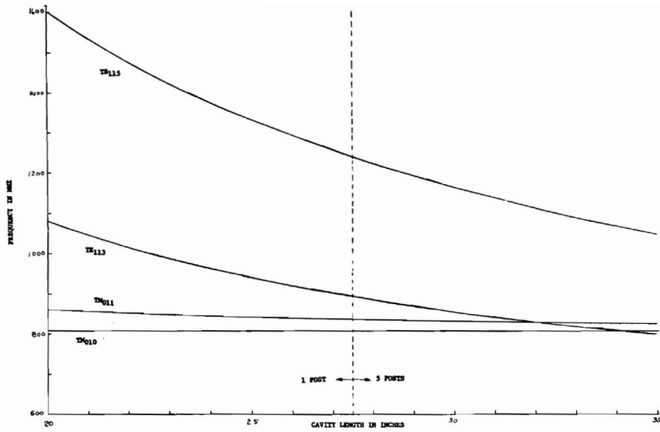
Fig. 6. Mode frequency versus bridge coupler length for the LAMPF bridge couplers.
