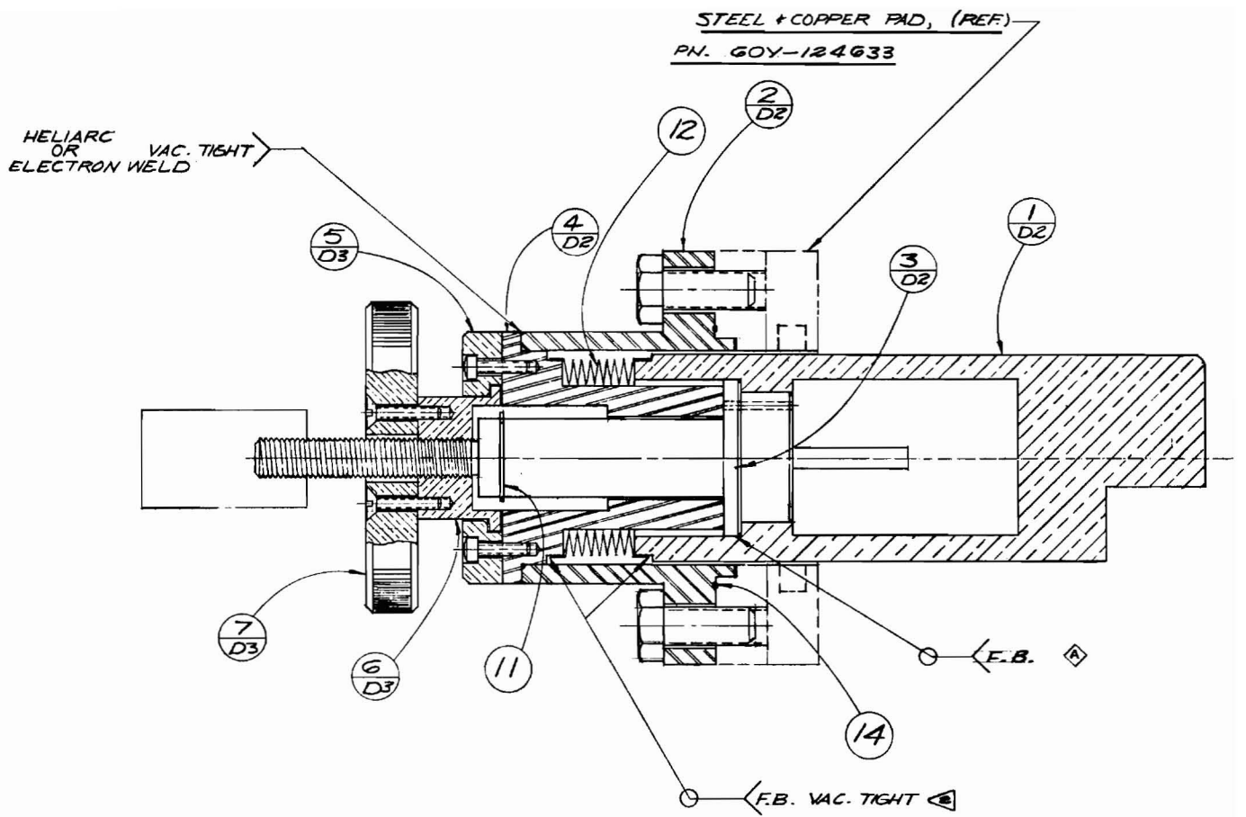
Fig. 4. Cross section of a typical adjustable post coupler.
