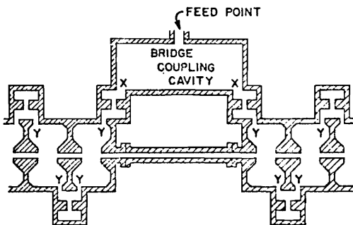
Fig. 2. Sketch of the basic form of a bridge coupler.
