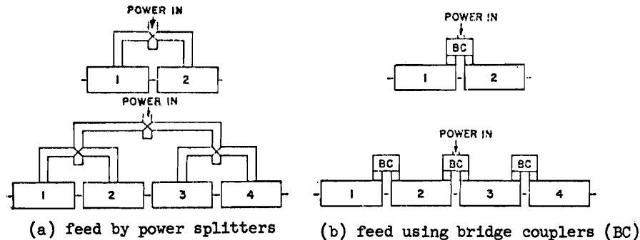
Fig. 1. Method of using bridge couplers to join 2 or 4 accelerator sections.
