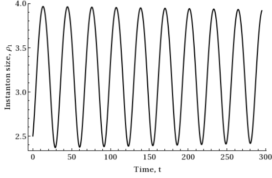
(a) The size of the first instanton, \rho_1 . This is drawing angular momentum away from the second.
