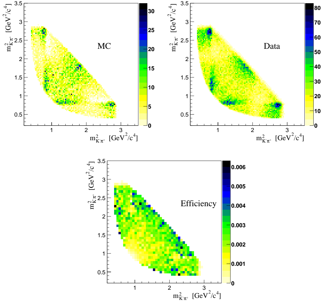
Figure 11.16: Dalitz-plot of the D^+ \rightarrow K^- \pi^+ \pi^+ decay in MC (left) and data (right). No background subtraction has been applied to data. The lower plot shows the non-uniformity of the trigger and reconstruction efficiency over the allowed Dalitz-space.
