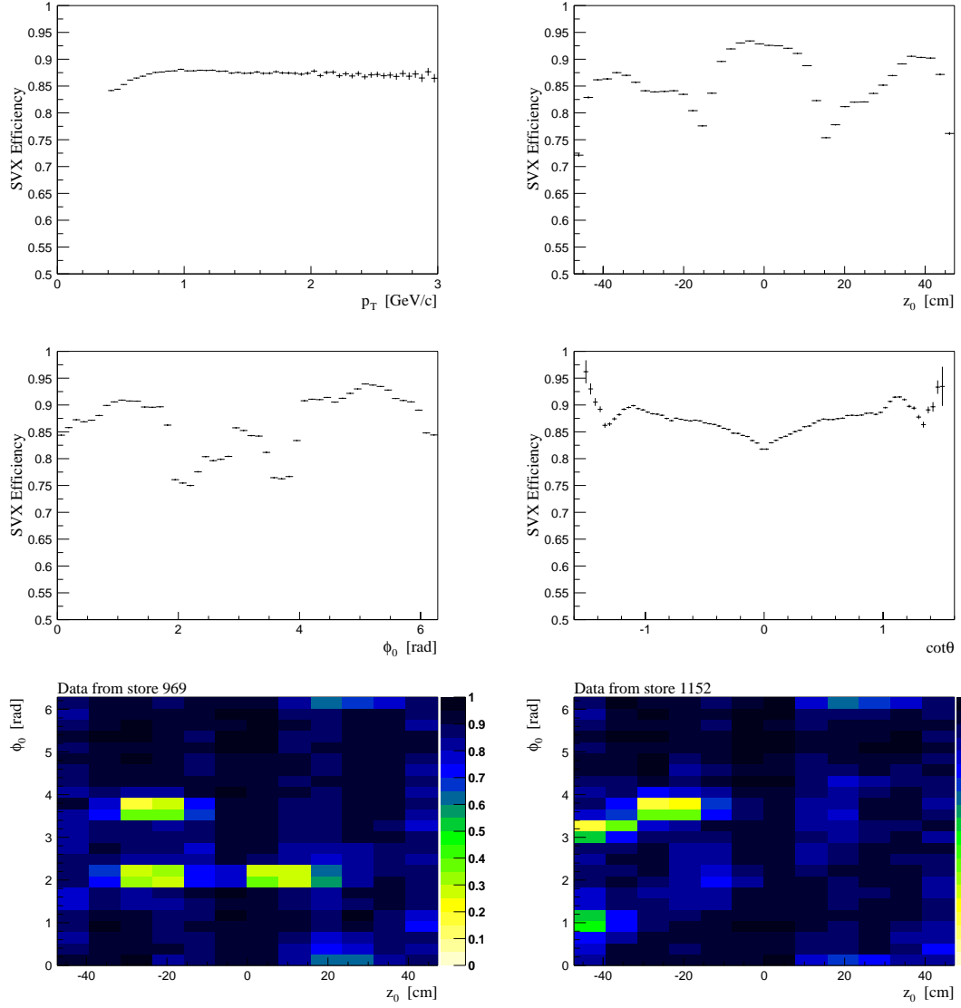
Figure 7.8: Single-track SVX efficiency as a function of p_T , z_0 , \phi_0 , and \cot\theta . The last two plots are the SVX efficiency as a function of z_0 and \phi_0 together for the data from two different beam stores, which shows the difference between their SVX configurations.
