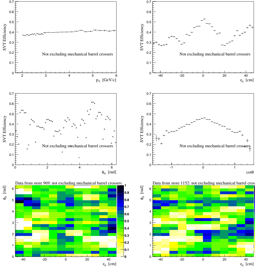
Figure 7.4: Single-track SVT efficiency as a function of p_T , z_0 , \phi_0 , and \cot \theta before excluding mechanical barrel-crossers. The last two plots are the SVT efficiency as a function of z_0 and \phi_0 together for the data from two different beam stores, which shows the difference between their SVT configuration.
