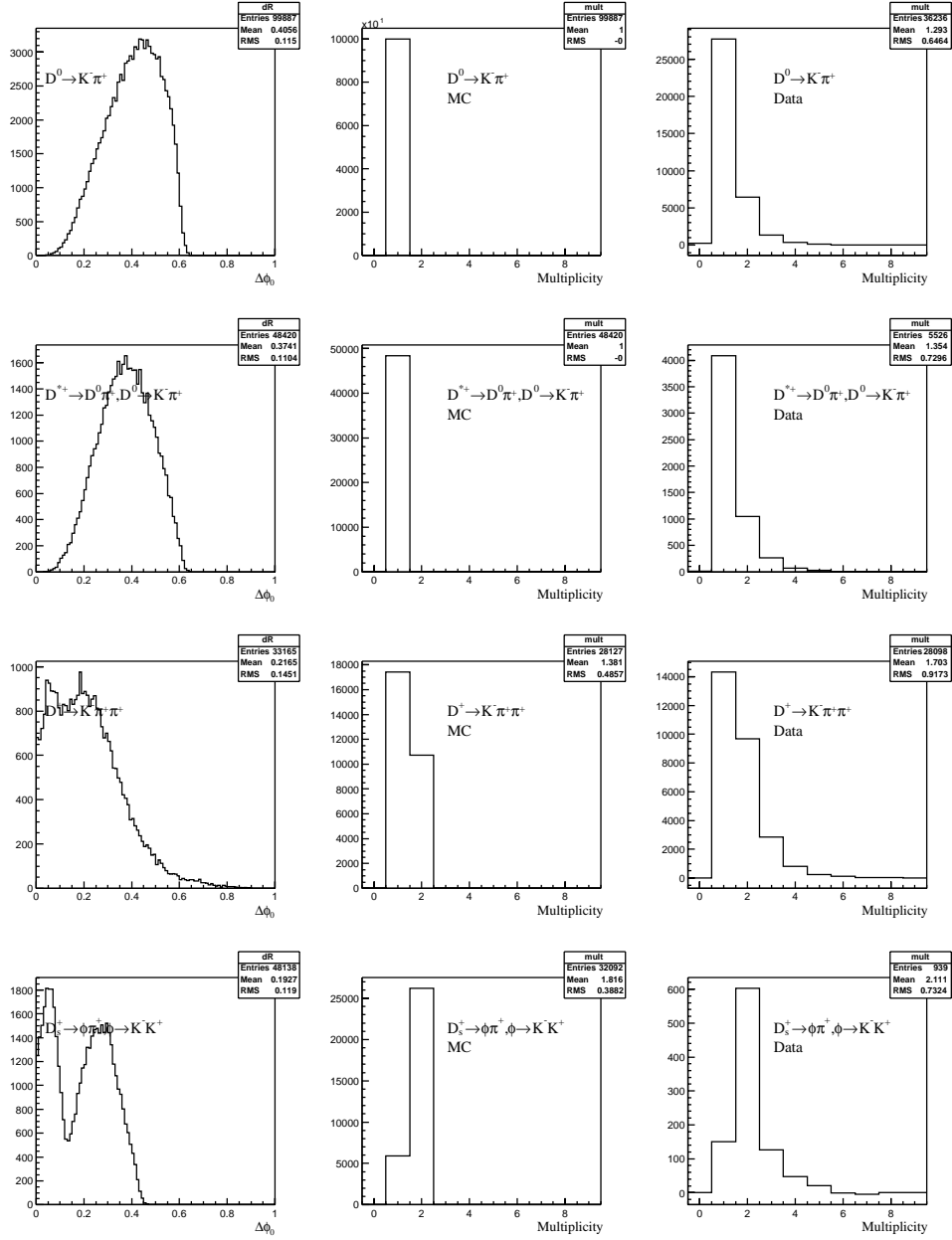
Figure 7.10: Left plots: The difference in angle between charm daughters with p_T \geq 2 \text{ GeV}/c (MC) after trigger and offline selection requirements. Middle plots: the MC multiplicity of tracks with p_T \geq 2 \text{ GeV}/c and |\Delta\phi| \leq 0.6 . The generator used for the MC is HeavyQuarkGen: one charm meson per event is generated; no fragmentation tracks are simulated. Right plots: the same multiplicity distribution for data.
