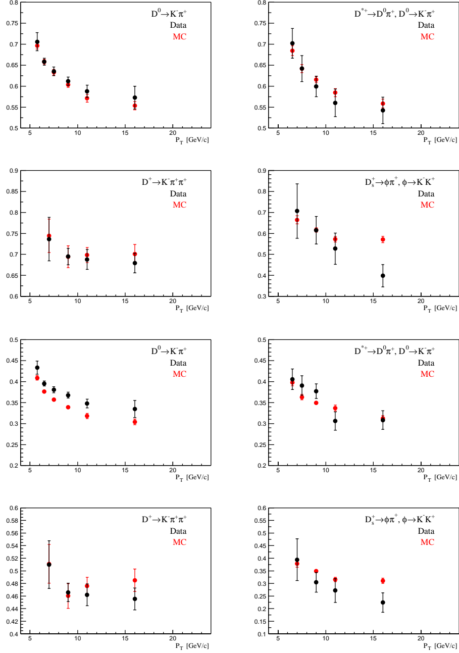
Figure 11.13: The ratio between the D meson yields with tight offline impact parameter requirements (150 \mu\text{m} in the upper four plots and 200 \mu\text{m} in the lower four plots) and no offline impact parameter requirement for MC (prompt D only) and data.
